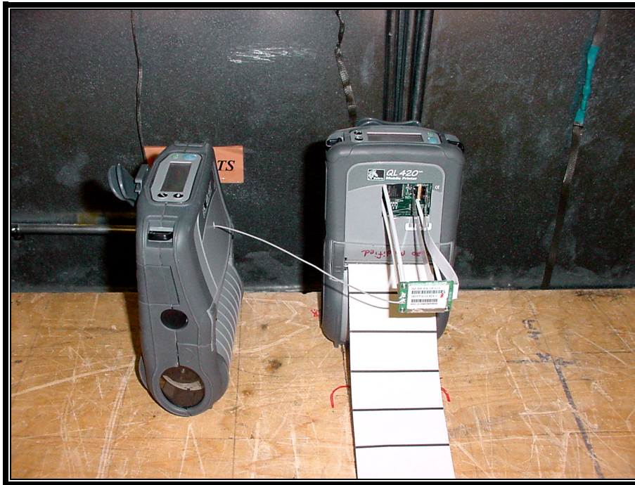
PHOTOGRAPH 11: CONDUCTED EMISSIONS FRONT VIEW USING QL-420 CQ17383-1 ANTENNA
