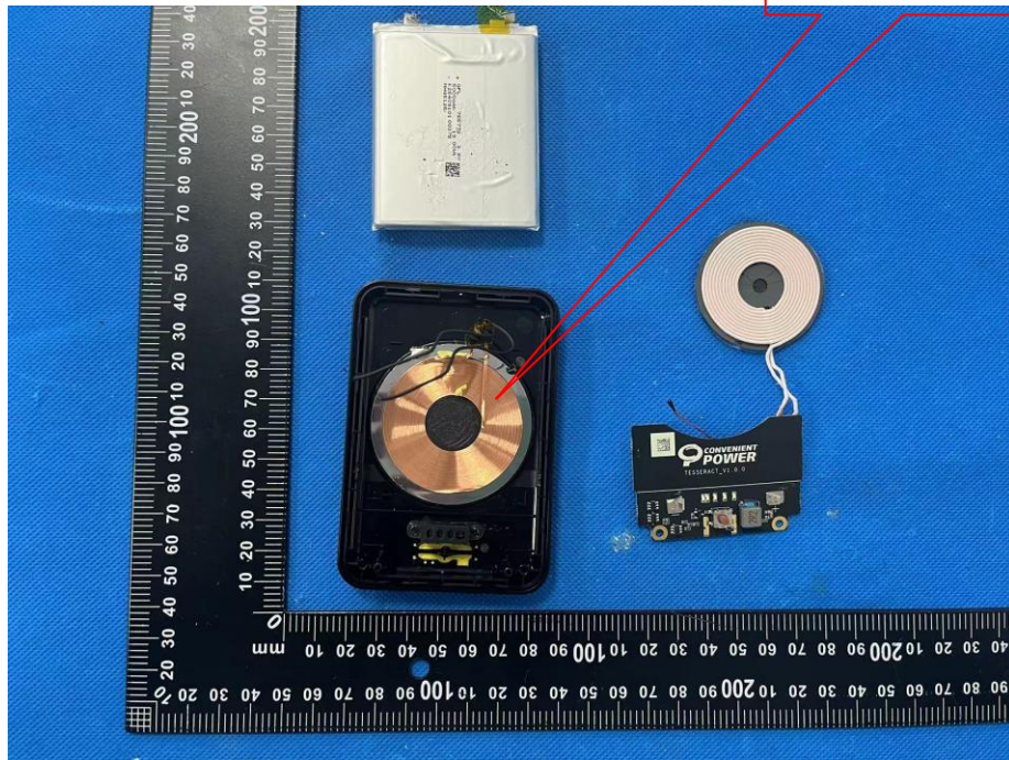
RX Antenna
