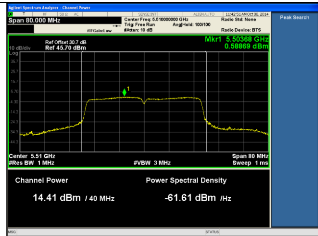
PSD-5510MHz-802.11n-40 Low-chain2
