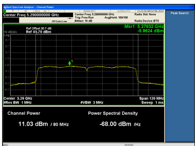
PSD-5290MHz-802.11ac-80 Mid-chain2
