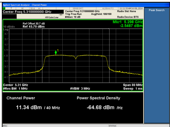
PSD-5310MHz-802.11n-40 High-chain2
