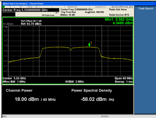
PSD-5550MHz-802.11n-40 Mid-chain1
