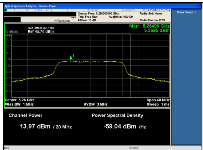
PSD-5260MHz-802.11a Low-chain2
