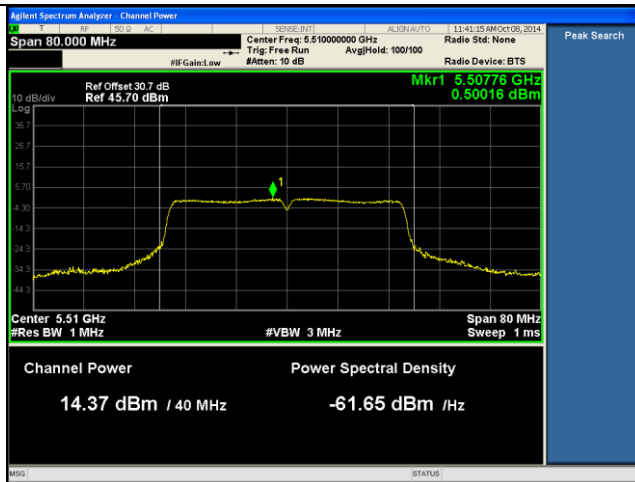
PSD-5510MHz-802.11n-40 Low-chain1
