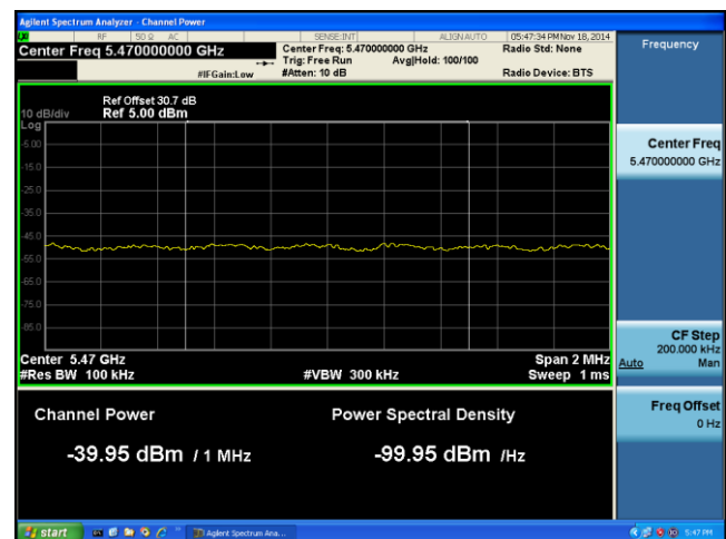
Band Edge-5470MHz-802.11a Low-Chain2
