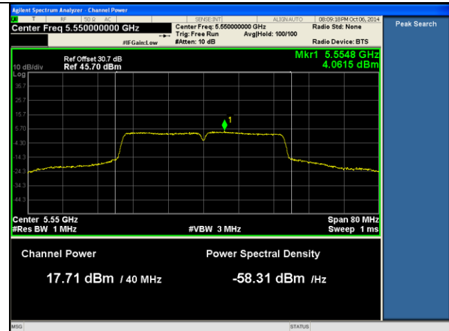
PSD-5550MHz-802.11n-40 Mid-chain2
