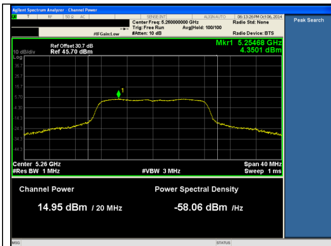
PSD-5260MHz-802.11a Low-chain1
