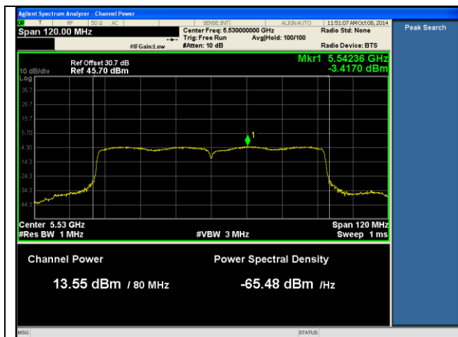
PSD-5530MHz-802.11ac-80 Mid-chain1
