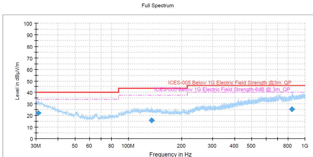
Figure 4: Spectral Diagrams, Radiated Emission, 30MHz-1000MHz, Vertical polarization
