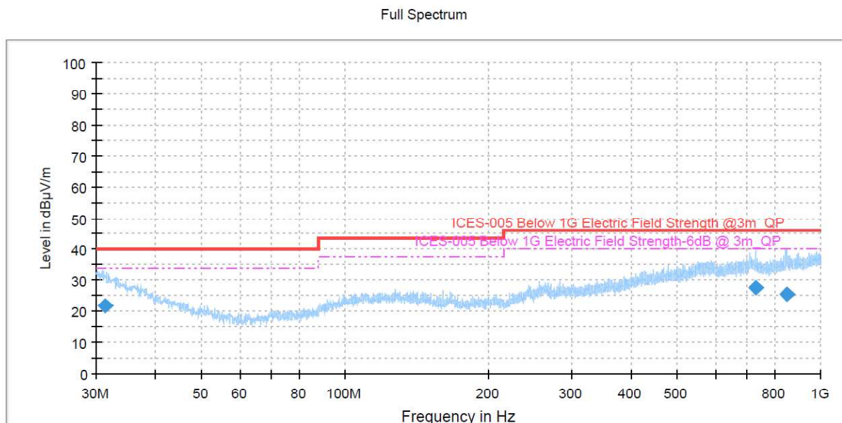
Figure 3: Spectral Diagrams, Radiated Emission, 30MHz-1000MHz, Horizontal polarization
