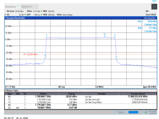
Band66-20MHz-64QAM-132572-100RB#0
