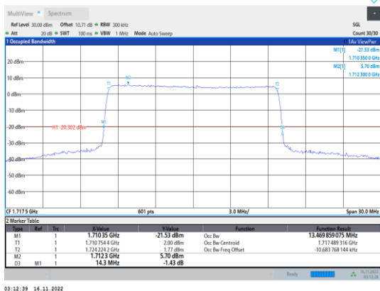
Band66-15MHz-64QAM-132047-75RB#0
