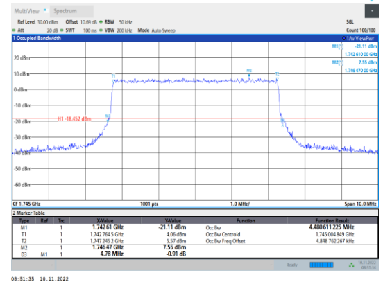
Band66-5MHz-16QAM-132322-25RB#0
