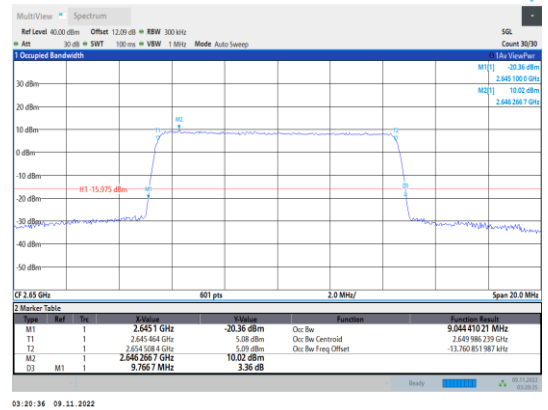
Band41-10MHz-QPSK-41190-50RB#0
