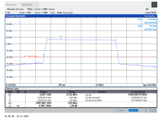
Band41-10MHz-64QAM-41190-50RB#0
