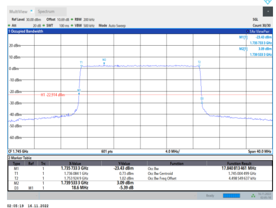
Band66-20MHz-64QAM-132322-100RB#0
