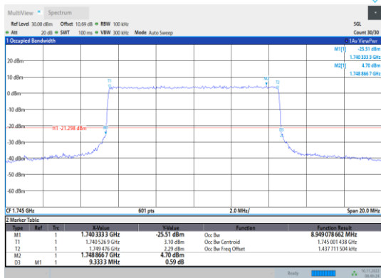
Band66-10MHz-16QAM-132322-50RB#0
