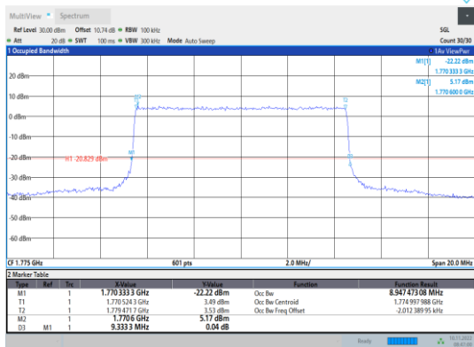
Band66-10MHz-16QAM-132622-50RB#0
