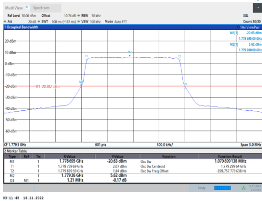
Band66-1.4MHz-64QAM-132665-6RB#0
