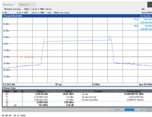
Band41-15MHz-64QAM-40115-75RB#0
