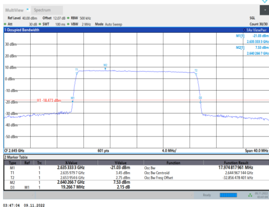
Band41-20MHz-16QAM-41140-100RB#0
