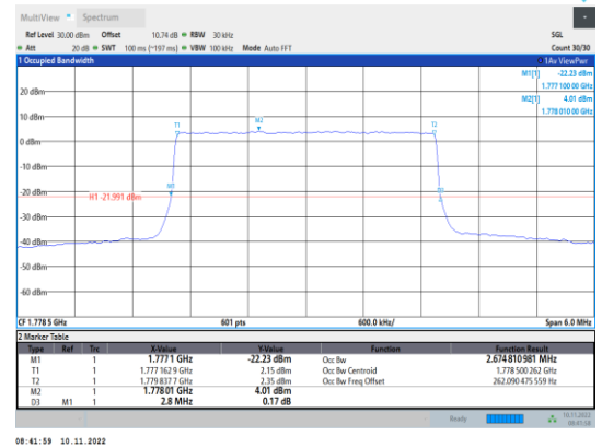
Band66-3MHz-QPSK-132657-15RB#0
