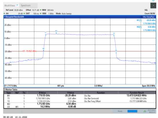
Band66-15MHz-16QAM-132047-75RB#0
