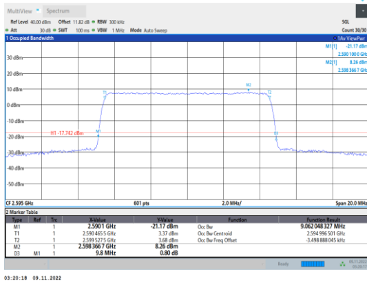
Band41-10MHz-16QAM-40640-50RB#0
