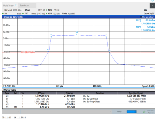
Band66-1.4MHz-64QAM-131979-6RB#0
