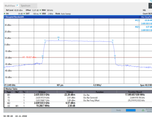
Band41-20MHz-64QAM-41140-100RB#0
