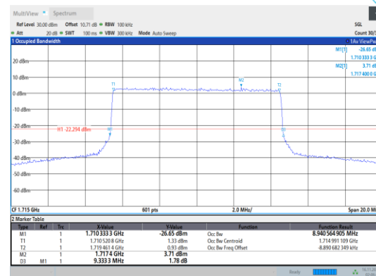
Band66-10MHz-64QAM-132022-50RB#0
