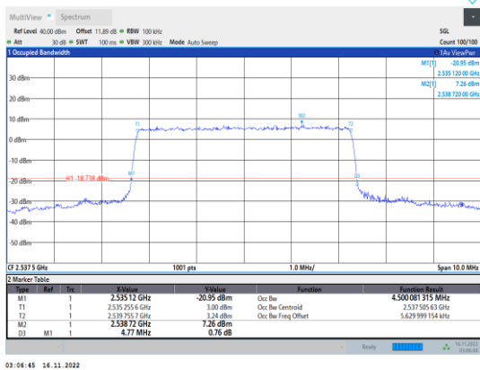
Band41-5MHz-64QAM-40065-25RB#0
