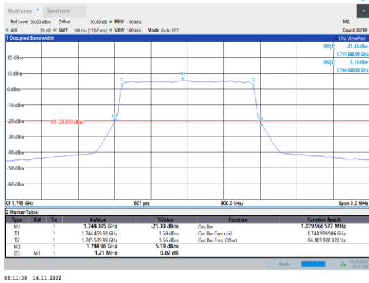
Band66-1.4MHz-64QAM-132322-6RB#0
