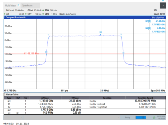
Band66-15MHz-16QAM-132322-75RB#0
