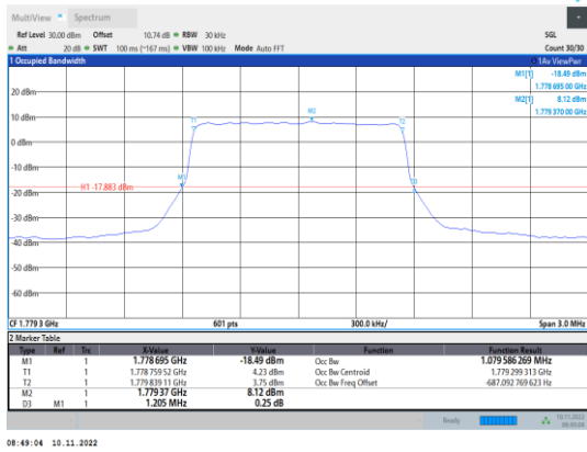
Band66-1.4MHz-QPSK-132665-6RB#0
