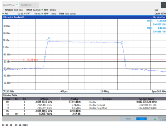
Band41-10MHz-16QAM-41190-50RB#0
