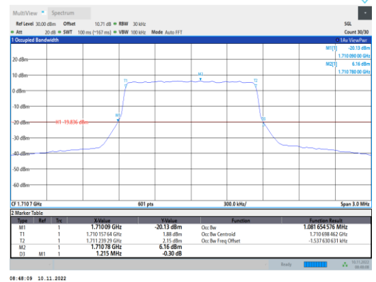
Band66-1.4MHz-16QAM-131979-6RB#0
