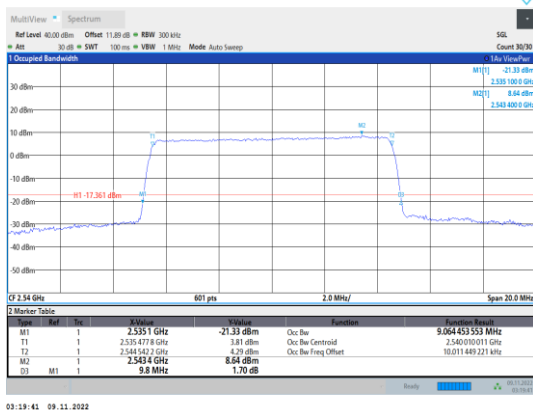
Band41-10MHz-16QAM-40090-50RB#0
