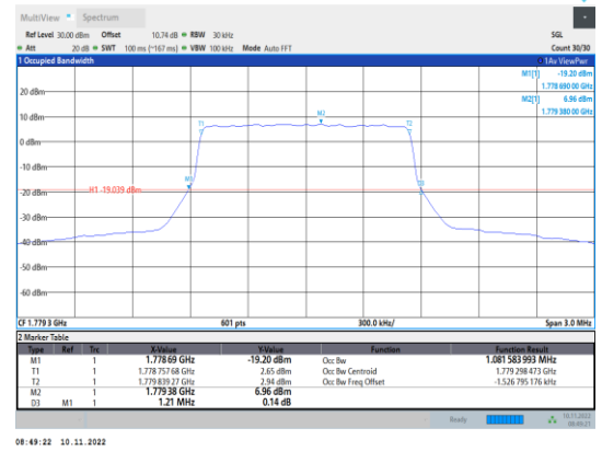
Band66-1.4MHz-16QAM-132665-6RB#0
