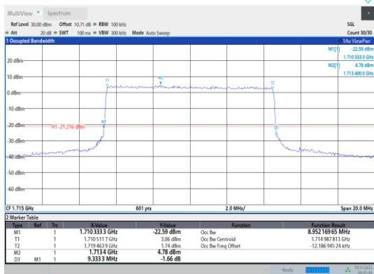
Band66-10MHz-16QAM-132022-50RB#0
