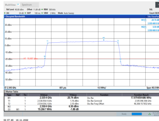
Band41-20MHz-64QAM-40140-100RB#0
