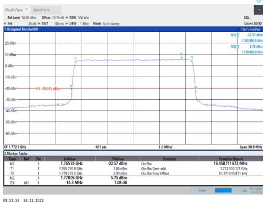
Band66-15MHz-64QAM-132597-75RB#0
