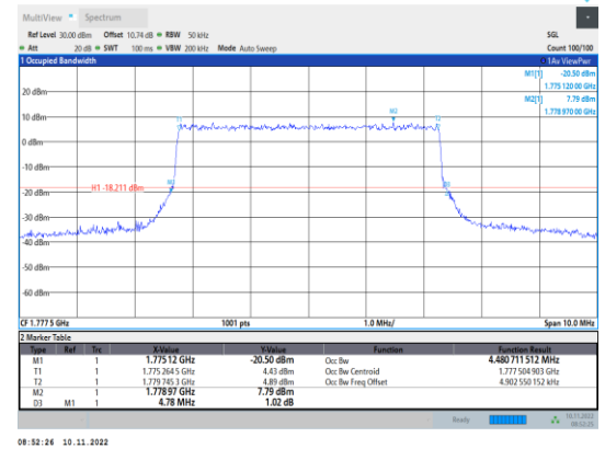
Band66-5MHz-16QAM-132647-25RB#0
