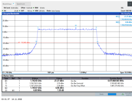
Band66-5MHz-64QAM-132322-25RB#0
