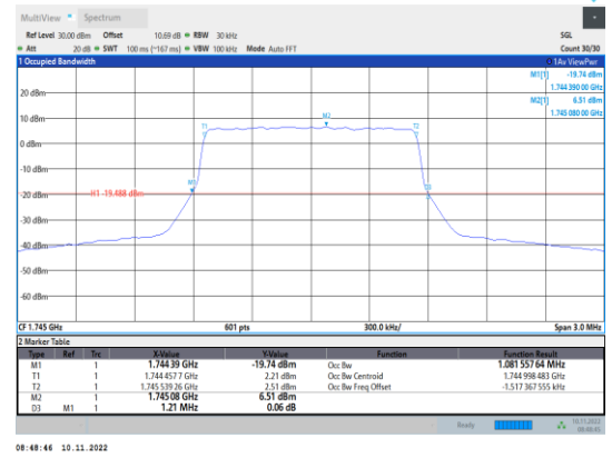
Band66-1.4MHz-16QAM-132322-6RB#0
