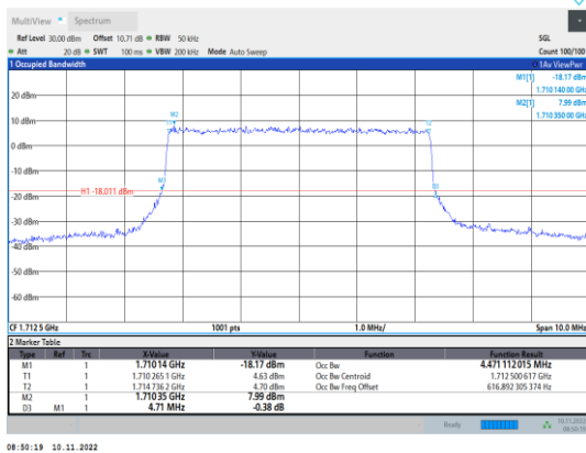
Band66-5MHz-QPSK-131997-25RB#0
