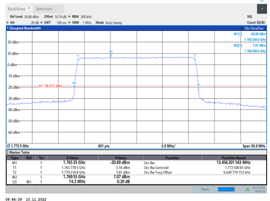
Band66-15MHz-16QAM-132597-75RB#0
