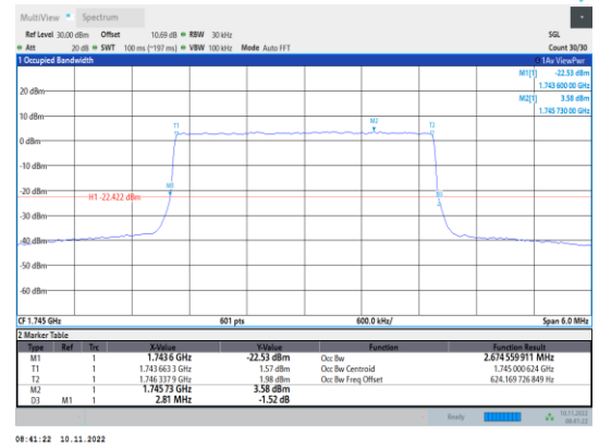
Band66-3MHz-QPSK-132322-15RB#0
