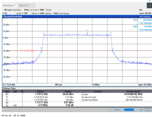
Band66-5MHz-64QAM-131997-25RB#0
