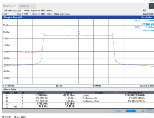
Band66-15MHz-64QAM-132322-75RB#0
