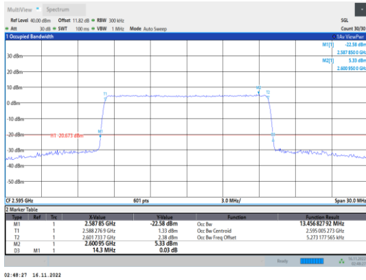
Band41-15MHz-64QAM-40640-75RB#0
