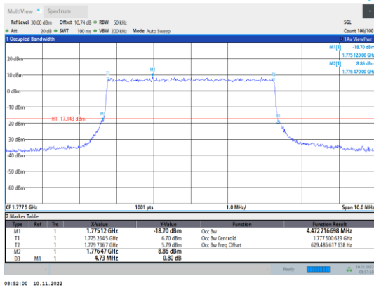
Band66-5MHz-QPSK-132647-25RB#0
