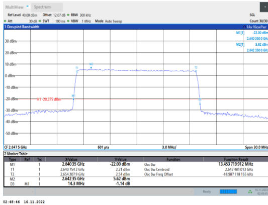
Band41-15MHz-64QAM-41165-75RB#0
