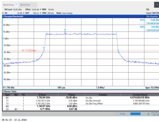
Band66-5MHz-QPSK-132322-25RB#0
