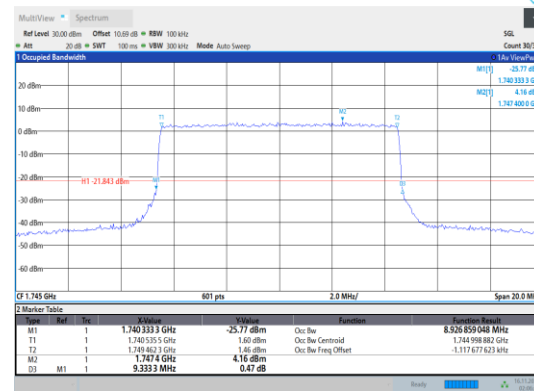
Band66-10MHz-64QAM-132322-50RB#0
