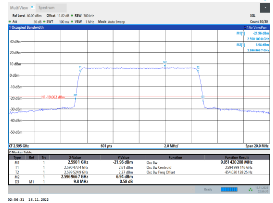
Band41-10MHz-64QAM-40640-50RB#0
