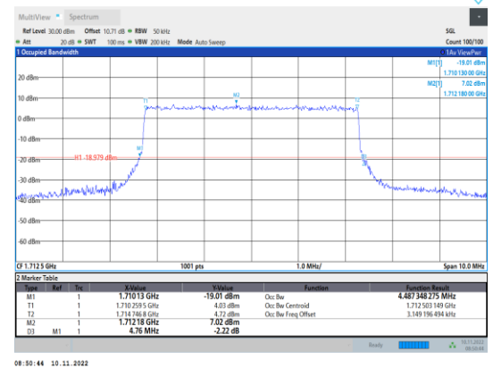
Band66-5MHz-16QAM-131997-25RB#0
