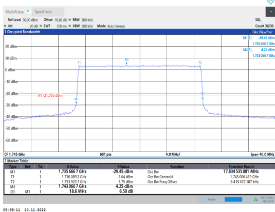
Band66-20MHz-16QAM-132322-100RB#0
