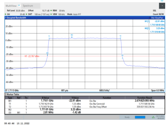
Band66-3MHz-QPSK-131987-15RB#0
