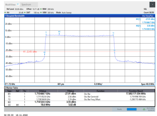
Band66-20MHz-64QAM-132072-100RB#0
