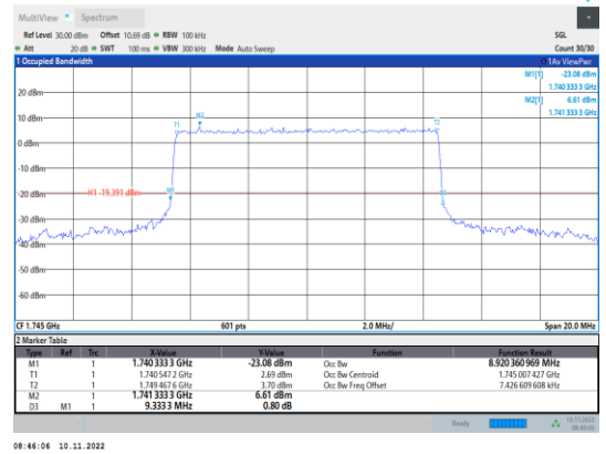
Band66-10MHz-QPSK-132322-50RB#0
