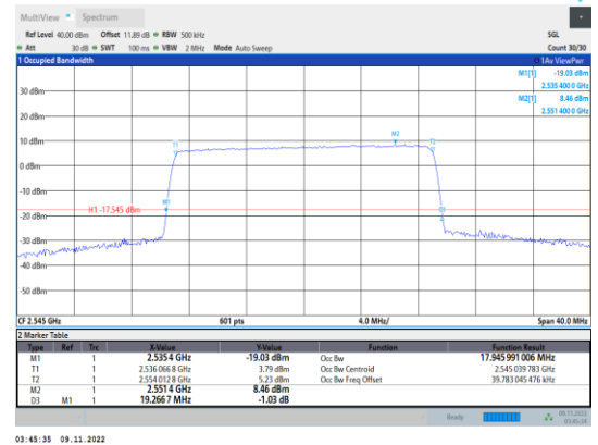
Band41-20MHz-QPSK-40140-100RB#0
