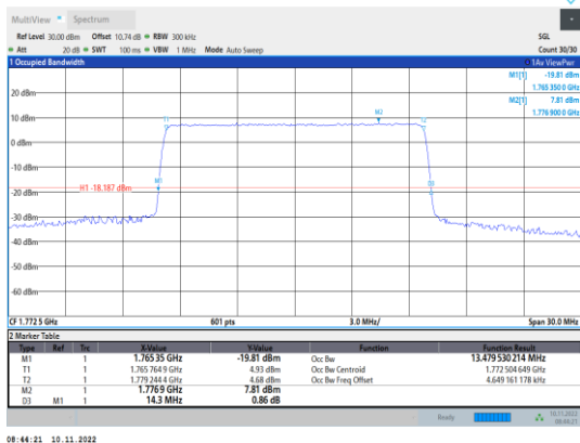
Band66-15MHz-QPSK-132597-75RB#0
