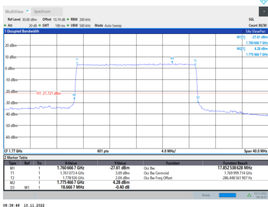
Band66-20MHz-16QAM-132572-100RB#0
