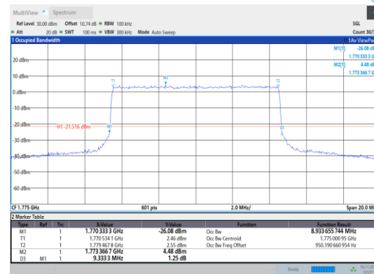
Band66-10MHz-64QAM-132622-50RB#0
