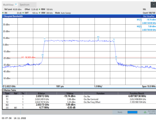
Band41-5MHz-64QAM-41215-25RB#0
