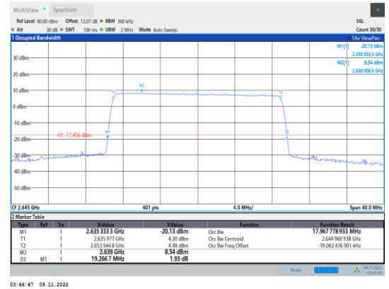
Band41-20MHz-QPSK-41140-100RB#0
