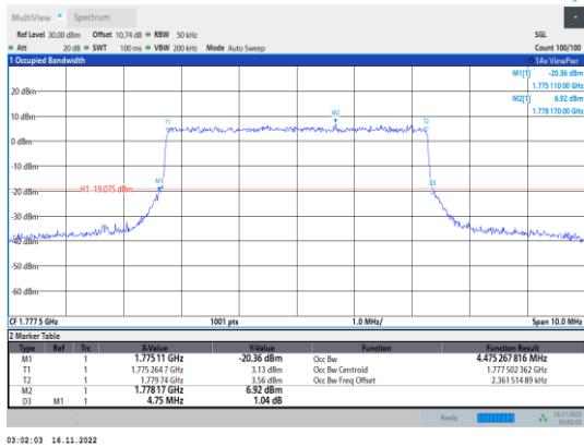
Band66-5MHz-64QAM-132647-25RB#0
