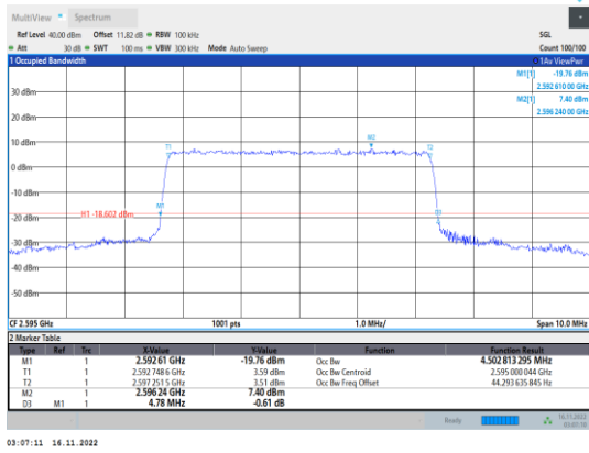
Band41-5MHz-64QAM-40640-25RB#0
