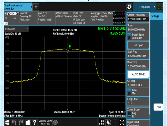
11AC40SISO-Ant2-5510
