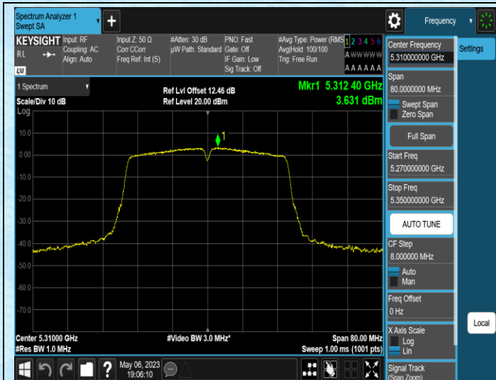
11AC40SISO-Ant2-5310
