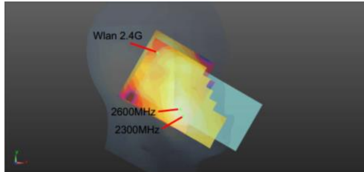
WWAN+WLAN2.4G Head
