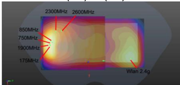
WWAN(5mm)+2.4G(5mm) Front
