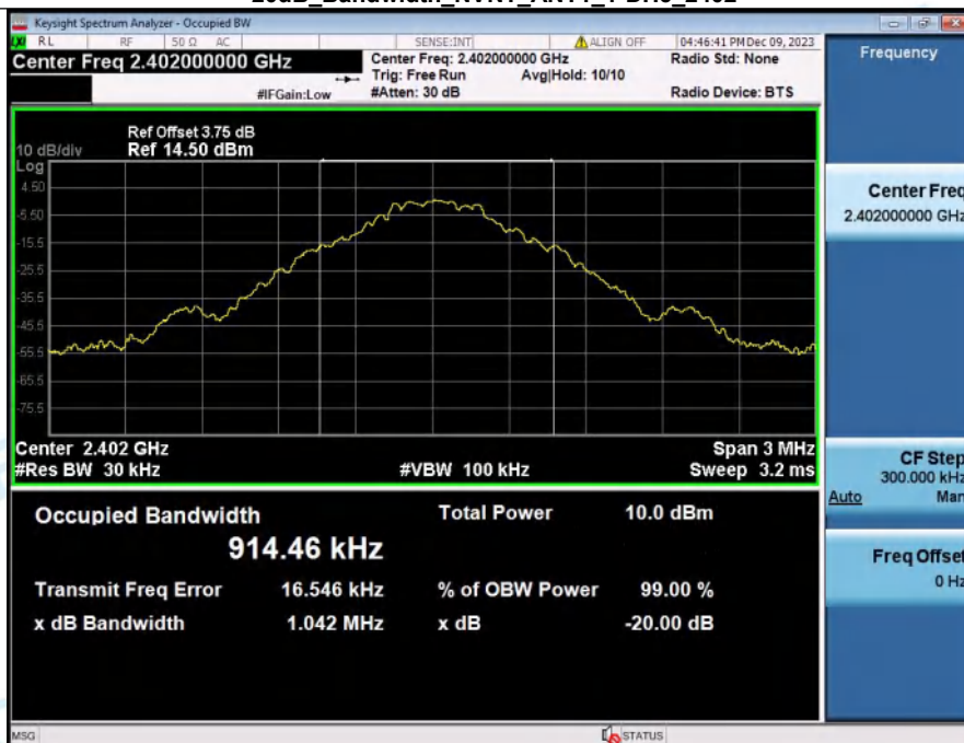
-20dB_Bandwidth_NVNT_ANT1_1-DH5_2402
