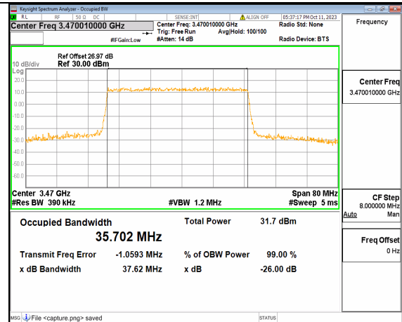
5A_n77(3450-3550MHz) 40M DFT-s-OFDM 64QAM Outer_Full Low
