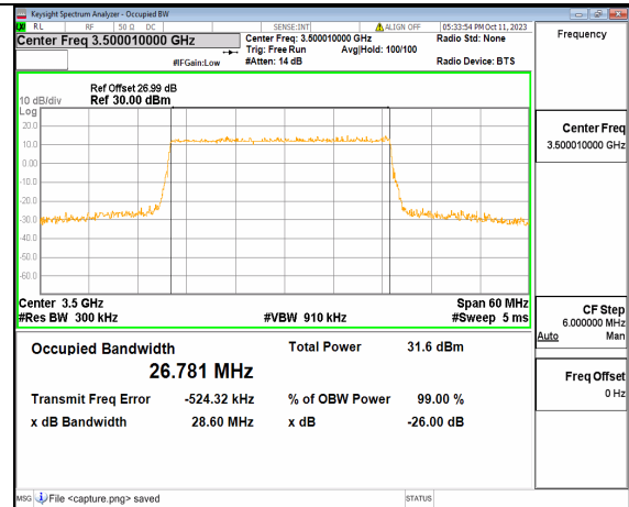
5A_n77(3450-3550MHz) 30M DFT-s-OFDM 64QAM Outer_Full Mid
