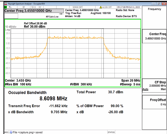
5A_n77(3450-3550MHz) 10M DFT-s-OFDM 64QAM Outer_Full Low
