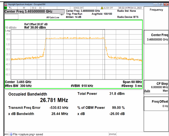
5A_n77(3450-3550MHz) 30M DFT-s-OFDM 64QAM Outer_Full Low
