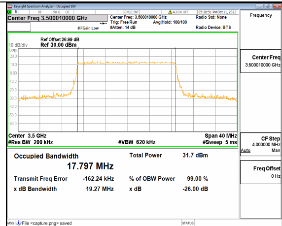
5A_n77(3450-3550MHz) 20M DFT-s-OFDM 64QAM Outer_Full Mid
