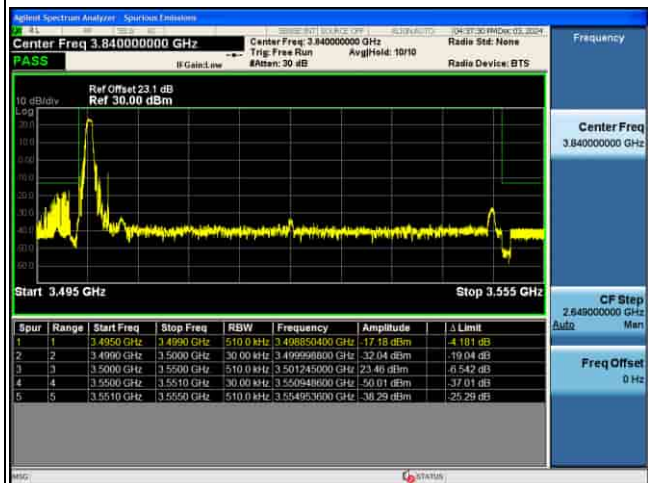
EDGE_5G_n77(K)_30KHz_P12-BPSK_50M_1RB@MAX_CH635000
