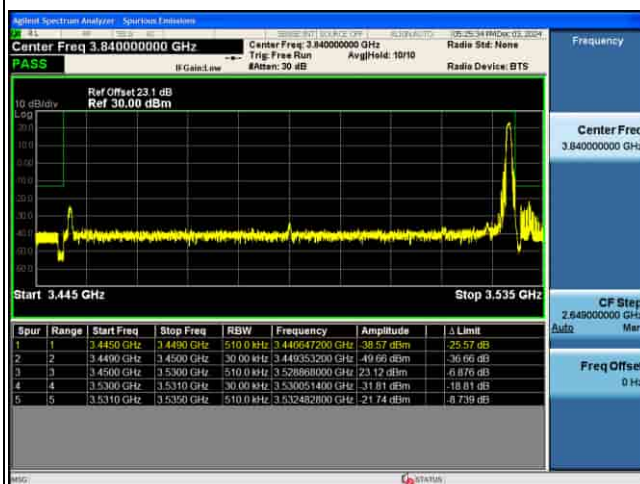
EDGE_5G_n77(K)_30KHz_P12-BPSK_80M_FULL RB@0_CH632668
