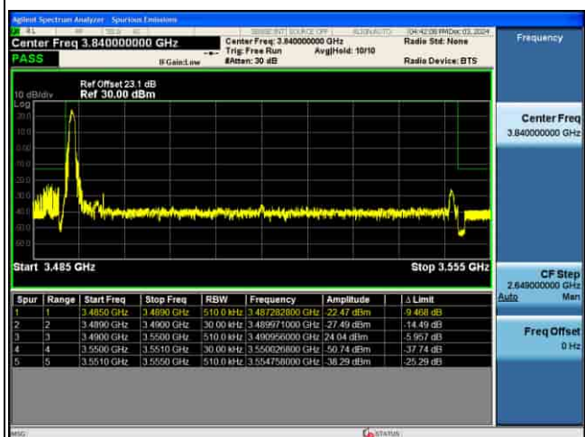
EDGE_5G_n77(K)_30KHz_Pi2-BPSK_60M_1RB@0_CH634666
