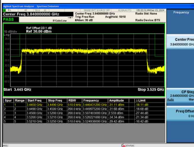
EDGE_5G_n77(K)_30KHz_P12-BPSK_70M_FULL RB@MAX_CH632334
