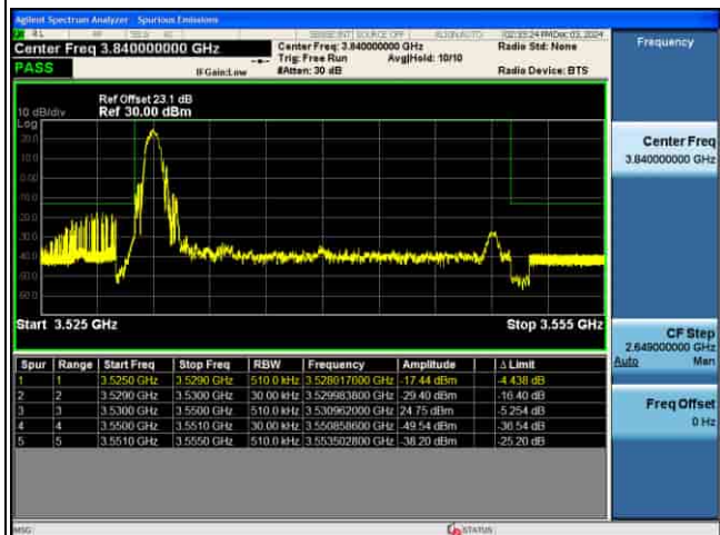
EDGE_5G_n77(K)_30KHz_P12-BPSK_20M_1RB@MAX_CH636000
