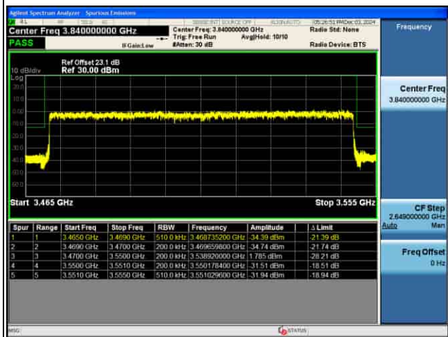
EDGE_5G_n77(K)_30KHz_P12-BPSK_90M_1RB@0_CH633666
