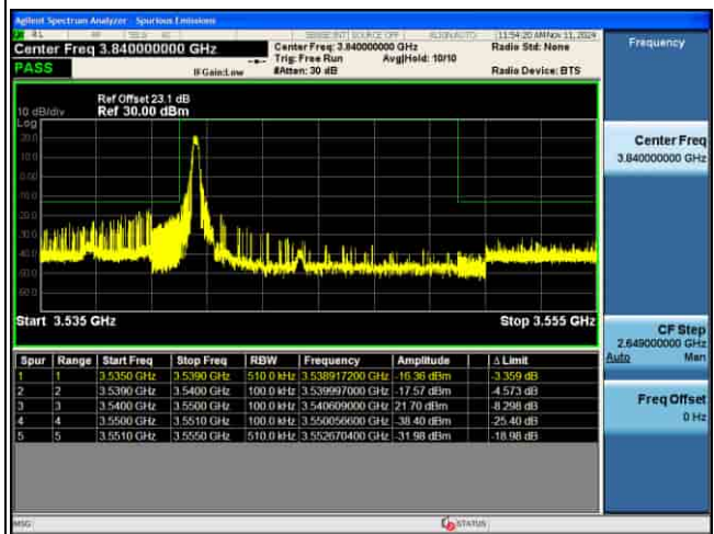
EDGE_4G_B42_QPSK_10M_1RB@MAX_CH43040
