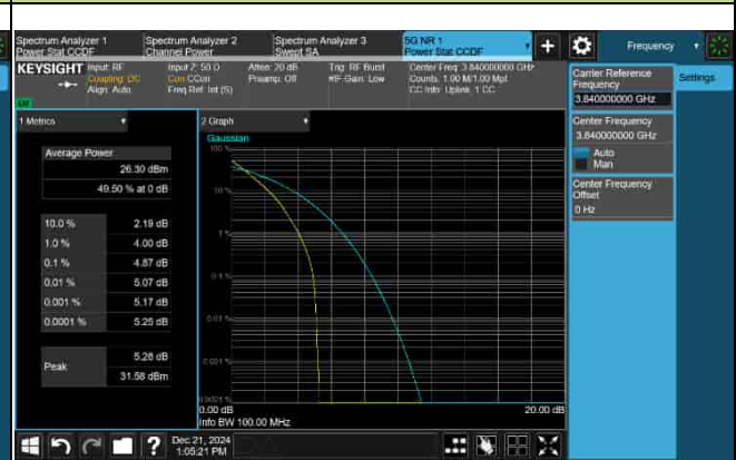
PAPR_5G_n77_30KHz_60M_3840MHz-64QAM
