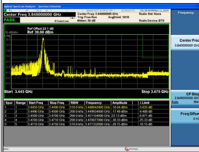
EDGE_4G_B42_QPSK_20M_1RB@MAX_CH42190
