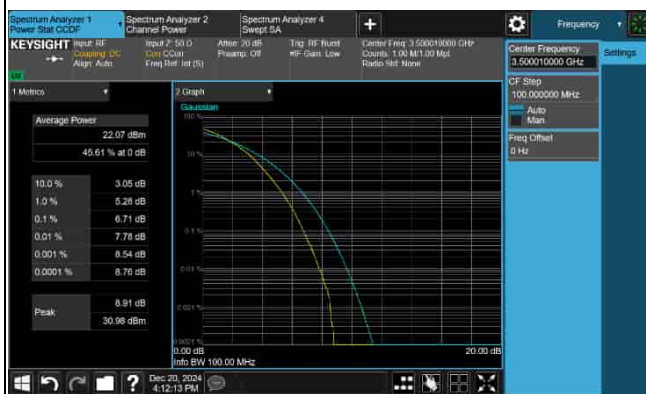
PAPR_5G_n77_30KHz_60M_3500.01MHz-256QAM
