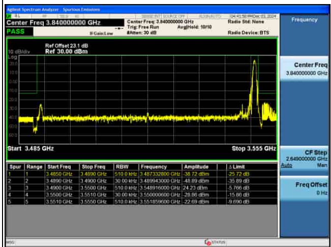
EDGE_5G_n77(K)_30KHz_P12-BPSK_60M_FULL RB@0_CH634666
