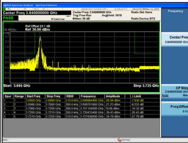
EDGE_4G_B43_QPSK_20M_1RB@MAX_CH44690
