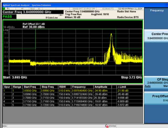
EDGE_4G_B43_QPSK_15M_FULL RB@0_CH44665
