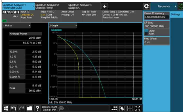
PAPR_5G_n77_30KHz_30M_3500.01MHz-16QAM
