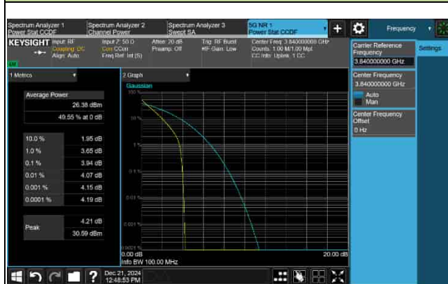
PAPR_5G_n77_30KHz_50M_3840MHz-16QAM
