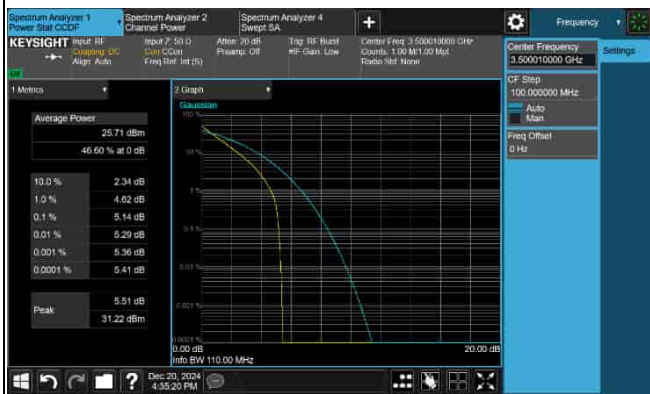
PAPR_5G_n77_30KHz_100M_3500.01MHz-16QAM
