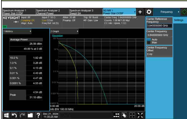
PAPR_5G_n77_30KHz_20M_3840MHz-16QAM
