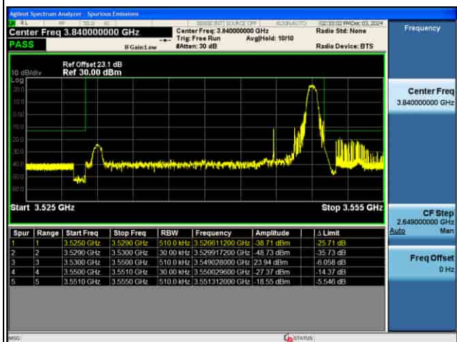
EDGE_5G_n77(K)_30KHz_P12-BPSK_20M_1RB@MAX_CH636000
