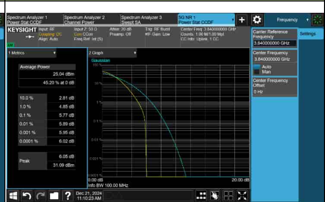
PAPR_5G_n77_30KHz_15M_3840MHz-64QAM
