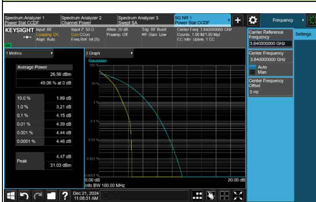
PAPR_5G_n77_30KHz_15M_3840MHz-16QAM
