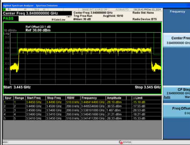
EDGE_5G_n77(K)_30KHz_Pi2-BPSK_90M_FULL RB@MAX_CH633000
