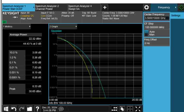
PAPR_5G_n77_30KHz_15M_3500.01MHz-256QAM
