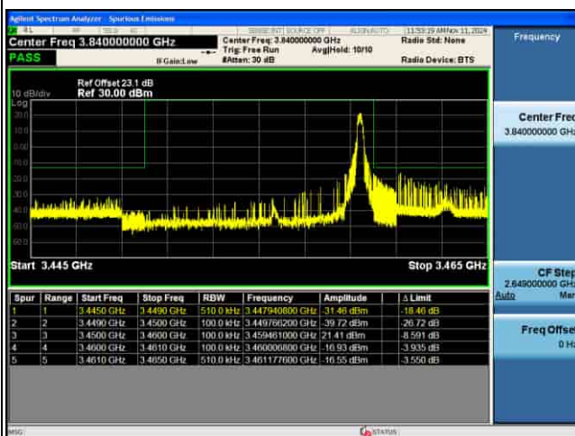
EDGE_4G_B42_QPSK_10M_FULL RB@0_CH42140
