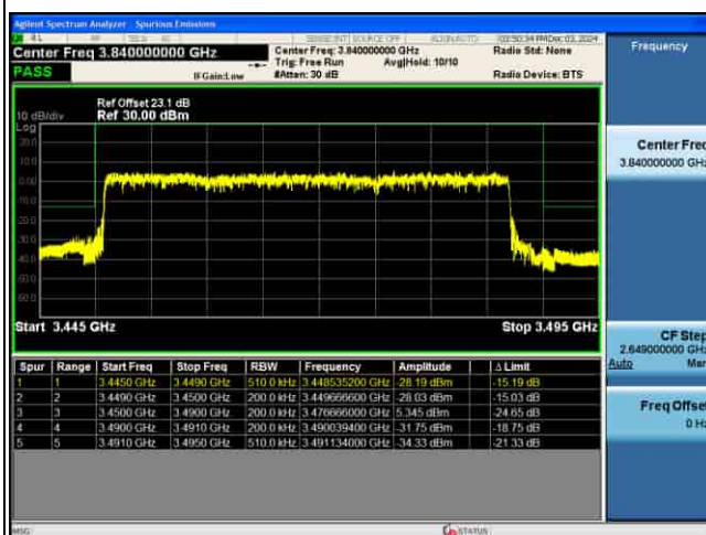
EDGE_5G_n77(K)_30KHz_P12-BPSK_40M_FULL RB@0_CH631334
