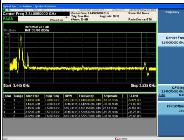
EDGE_5G_n77(K)_30KHz_P12-BPSK_70M_1RB@0_CH632334
