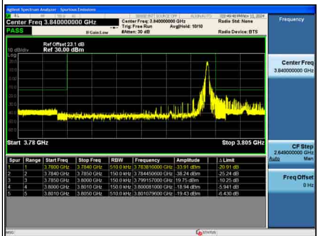
EDGE_4G_B43_QPSK_15M_FULL RB@0_CH45515
