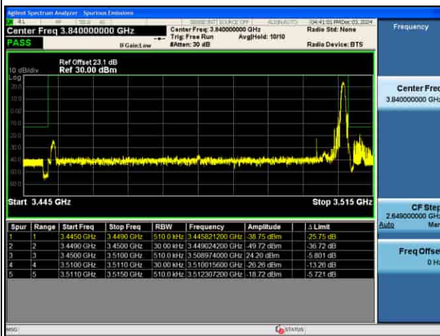
EDGE_5G_n77(K)_30KHz_P12-BPSK_60M_FULL RB@0_CH632000
