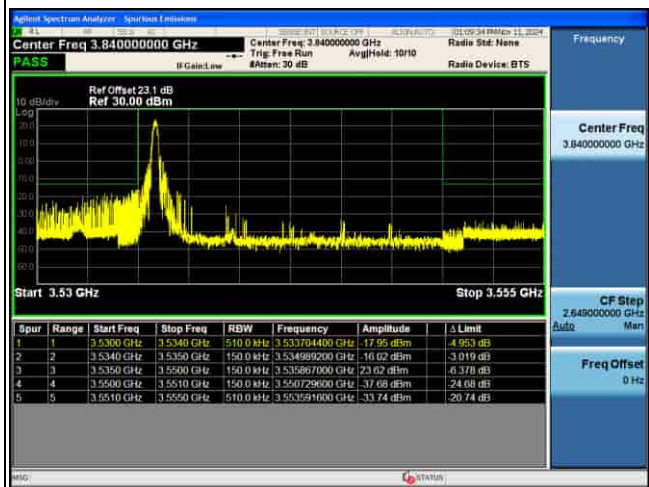
EDGE_4G_B42_QPSK_15M_1RB@MAX_CH43015
