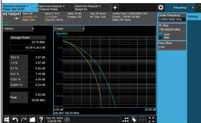
PAPR_5G_n77_30KHz_90M_3500.01MHz-256QAM
