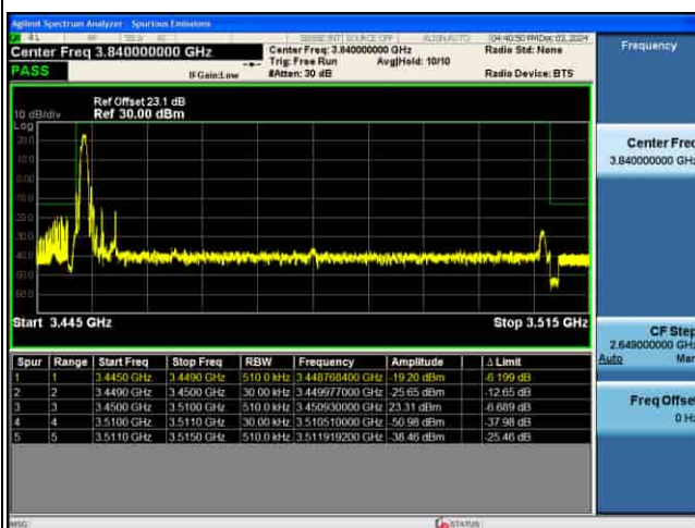
EDGE_5G_n77(K)_30KHz_Pi2-BPSK_60M_1RB@0_CH632000
