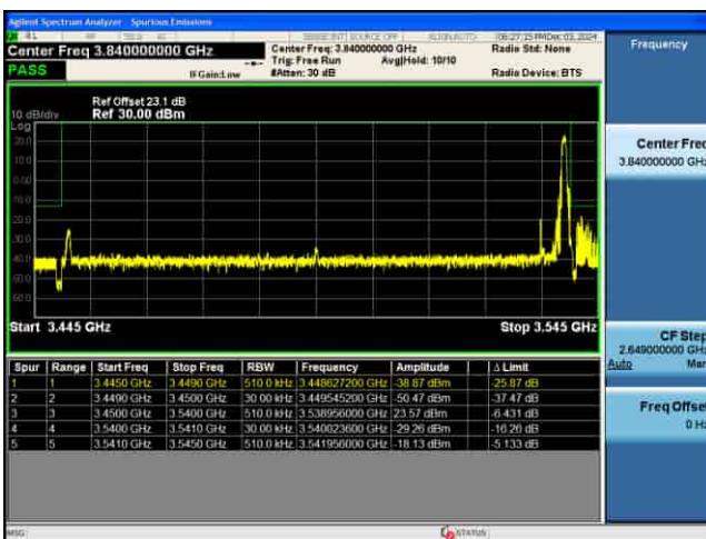
EDGE_5G_n77(K)_30KHz_P12-BPSK_90M_1RB@MAX_CH633000
