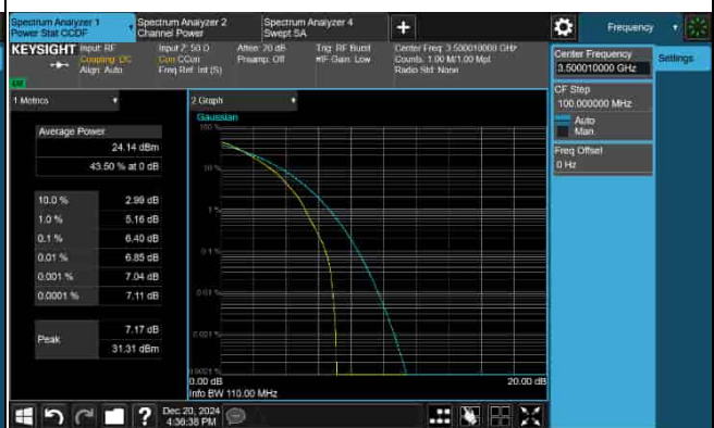
PAPR_5G_n77_30KHz_100M_3500.01MHz-64QAM
