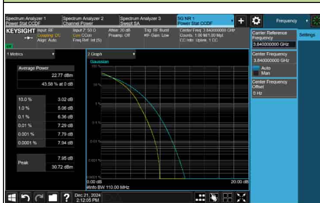
PAPR_5G_n77_30KHz_100M_3840MHz-256QAM
