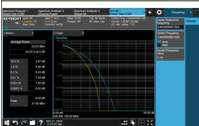
PAPR_5G_n77_30KHz_15M_3840MHz-256QAM
