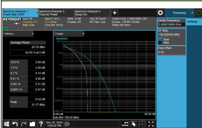
PAPR_5G_n77_30KHz_20M_3500.01MHz-16QAM
