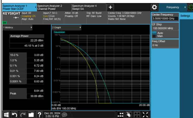
PAPR_5G_n77_30KHz_30M_3500.01MHz-256QAM
