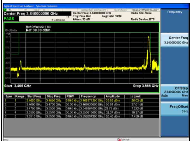
EDGE_5G_n77(K)_30KHz_P12-BPSK_80M_FULL RB@0_CH634000
