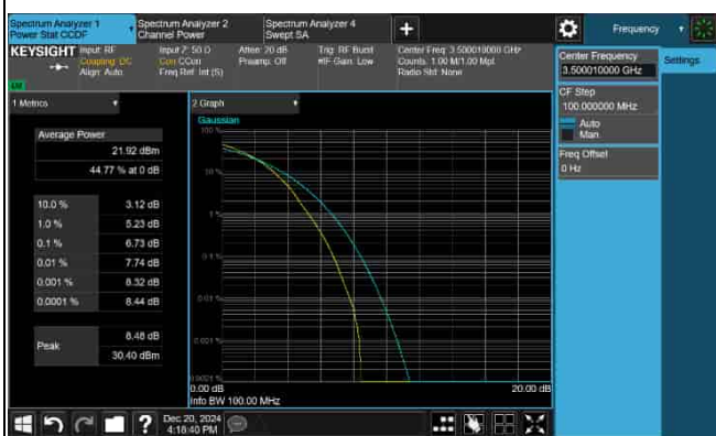
PAPR_5G_n77_30KHz_70M_3500.01MHz-256QAM
