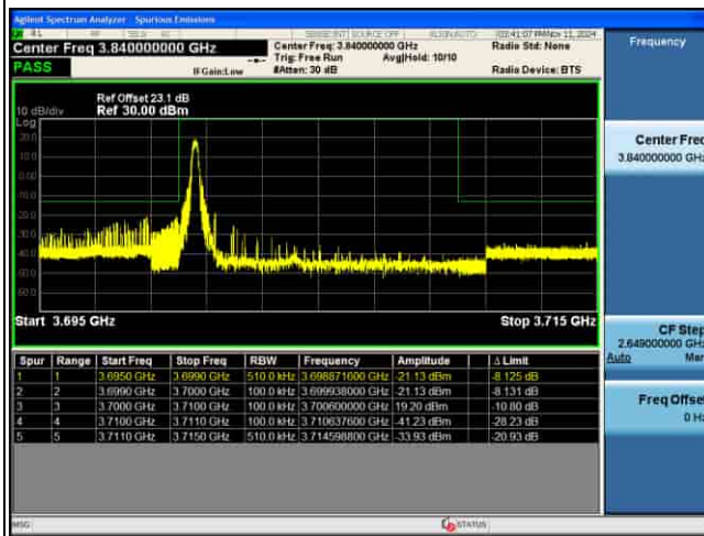
EDGE_4G_B43_QPSK_10M_1RB@MAX_CH44640
