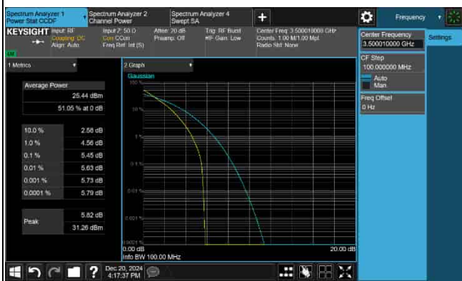
PAPR_5G_n77_30KHz_70M_3500.01MHz-16QAM
