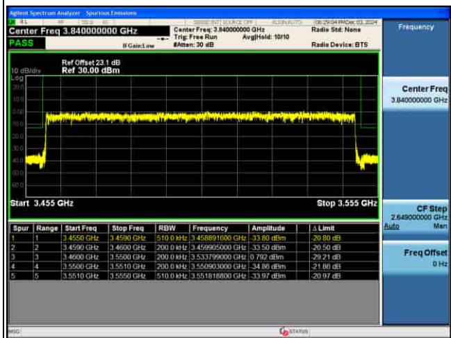
EDGE_5G_n77(K)_30KHz_Pi2-BPSK_90M_FULL RB@MAX_CH633666
