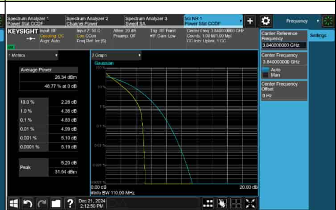
PAPR_5G_n77_30KHz_100M_3840MHz-64QAM
