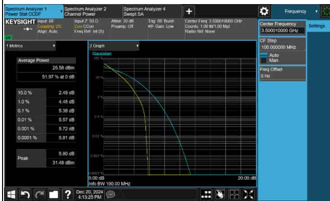
PAPR_5G_n77_30KHz_60M_3500.01MHz-16QAM
