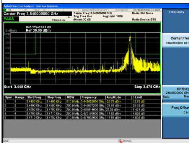
EDGE_4G_B42_QPSK_20M_FULL RB@0_CH42190
