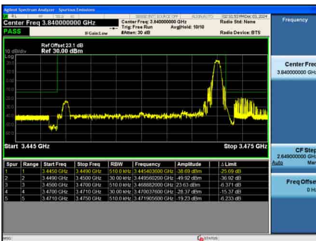
EDGE_5G_n77(K)_30KHz_P12-BPSK_20M_1RB@MAX_CH630668
