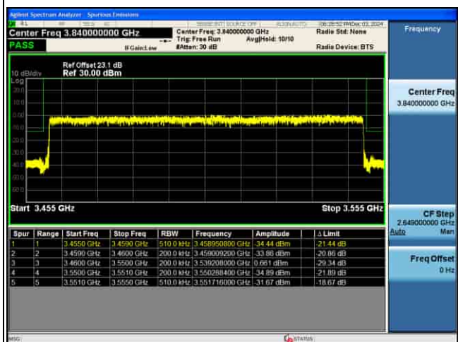
EDGE_5G_n77(K)_30KHz_Pi2-BPSK_100M_1RB@MAX_CH633334
