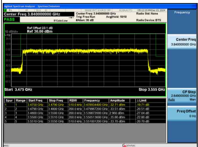
EDGE_5G_n77(K)_30KHz_P12-BPSK_70M_FULL RB@MAX_CH634332
