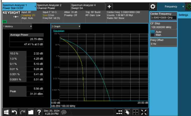
PAPR_5G_n77_30KHz_90M_3500.01MHz-16QAM
