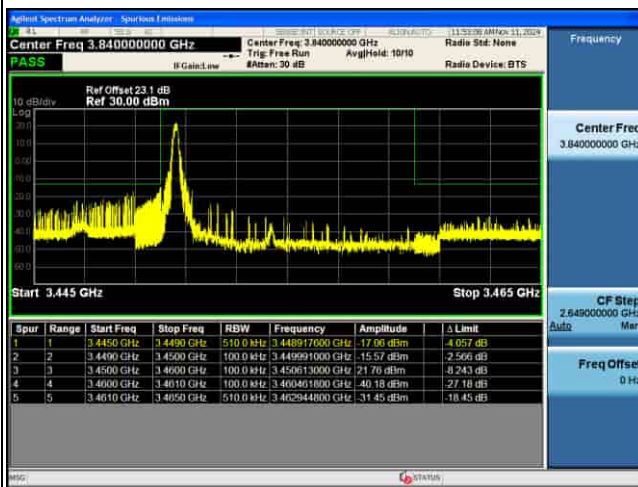
EDGE_4G_B42_QPSK_10M_1RB@MAX_CH42140
