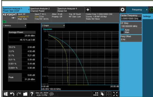
PAPR_5G_n77_30KHz_80M_3500.01MHz-16QAM
