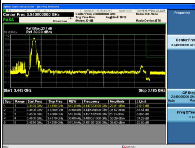
EDGE_5G_n77(K)_30KHz_Pi2-BPSK_30M_1RB@0_CH631000
