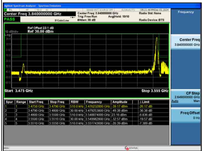
EDGE_5G_n77(K)_30KHz_P12-BPSK_70M_FULL RB@0_CH634332
