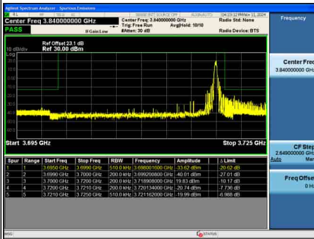
EDGE_4G_B43_QPSK_20M_FULL RB@0_CH44690
