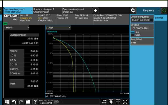
PAPR_5G_n77_30KHz_80M_3500.01MHz-64QAM
