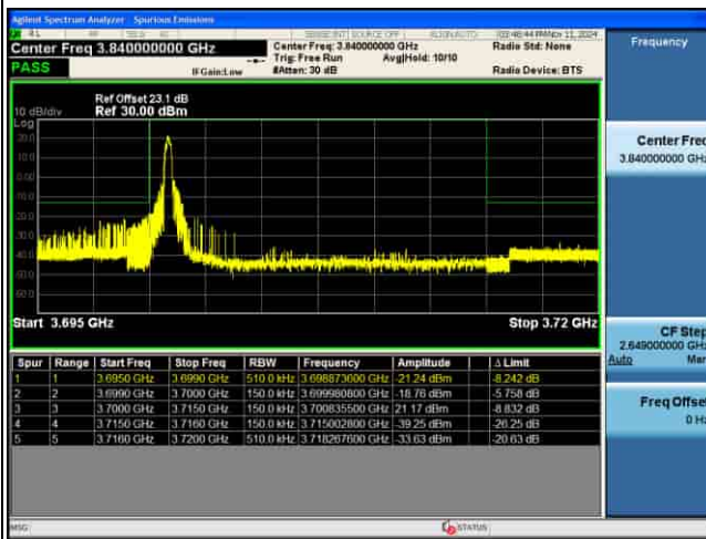
EDGE_4G_B43_QPSK_15M_1RB@MAX_CH44665
