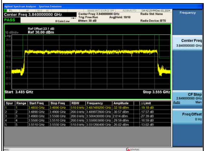
EDGE_5G_n77(K)_30KHz_P12-BPSK_70M_1RB@0_CH634332
