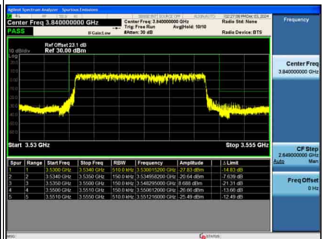
EDGE_5G_n77(K)_30KHz_P12-BPSK_15M_FULL RB@0_CH636166
