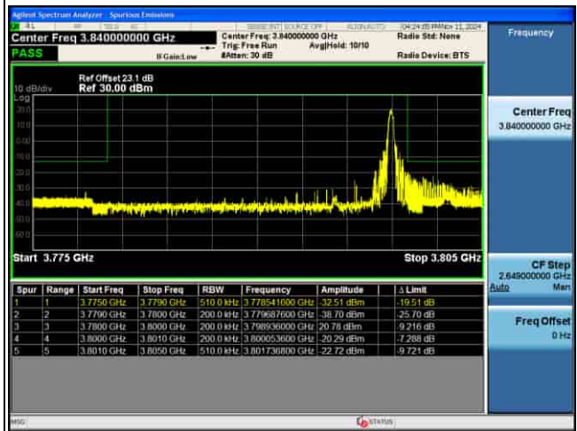
EDGE_4G_B43_QPSK_20M_FULL RB@0_CH45490
