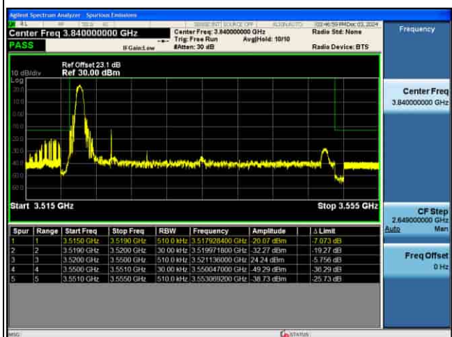
EDGE_5G_n77(K)_30KHz_Pi2-BPSK_30M_1RB@0_CH635666
