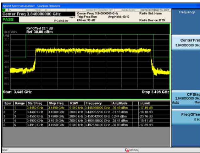
EDGE_5G_n77(K)_30KHz_P12-BPSK_50M_1RB@0_CH631668
