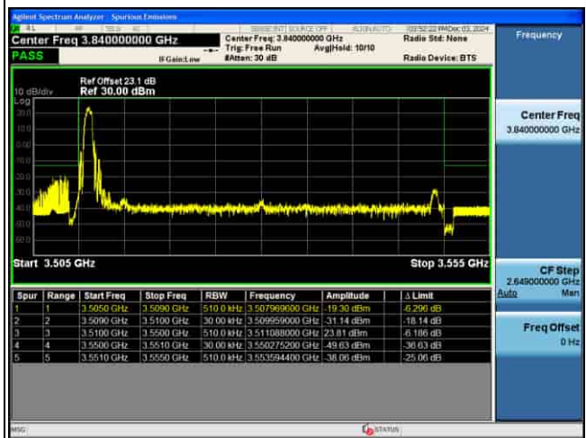
EDGE_5G_n77(K)_30KHz_P12-BPSK_40M_1RB@MAX_CH635332
