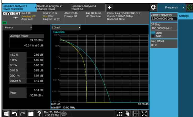
PAPR_5G_n77_30KHz_100M_3500.01MHz-256QAM
