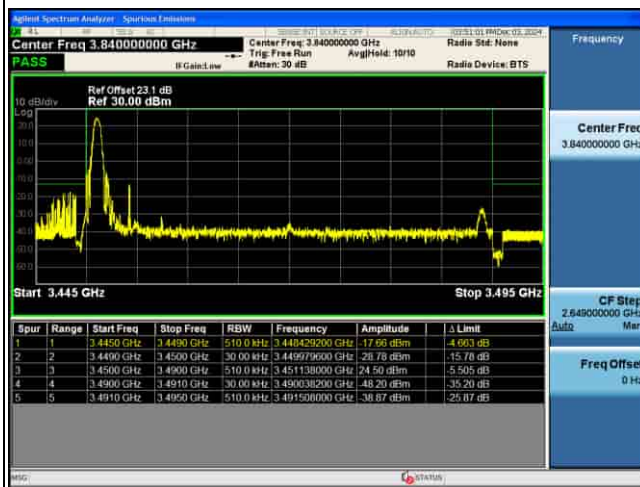
EDGE_5G_n77(K)_30KHz_P12-BPSK_40M_1RB@MAX_CH631334
