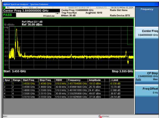
EDGE_5G_n77(K)_30KHz_P12-BPSK_90M_1RB@MAX_CH633666
