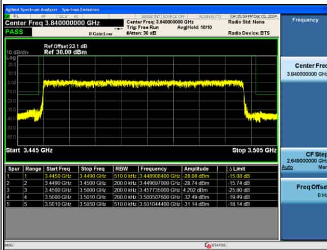
EDGE_5G_n77(K)_30KHz_Pi2-BPSK_50M_FULL RB@MAX_CH631668
