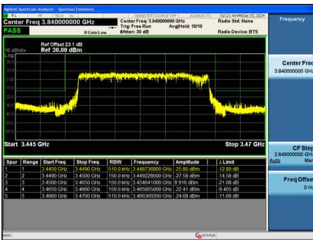
EDGE_5G_n77(K)_30KHz_P12-BPSK_20M_1RB@0_CH630668
