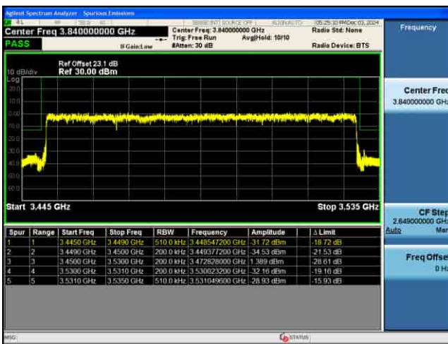
EDGE_5G_n77(K)_30KHz_P12-BPSK_90M_1RB@0_CH633000
