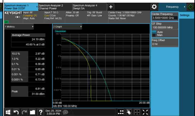
PAPR_5G_n77_30KHz_30M_3500.01MHz-64QAM
