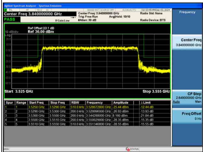
EDGE_5G_n77(K)_30KHz_Pi2-BPSK_20M_FULL RB@MAX_CH636000
