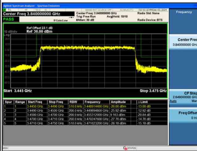
EDGE_5G_n77(K)_30KHz_Pi2-BPSK_20M_FULL RB@MAX_CH630668
