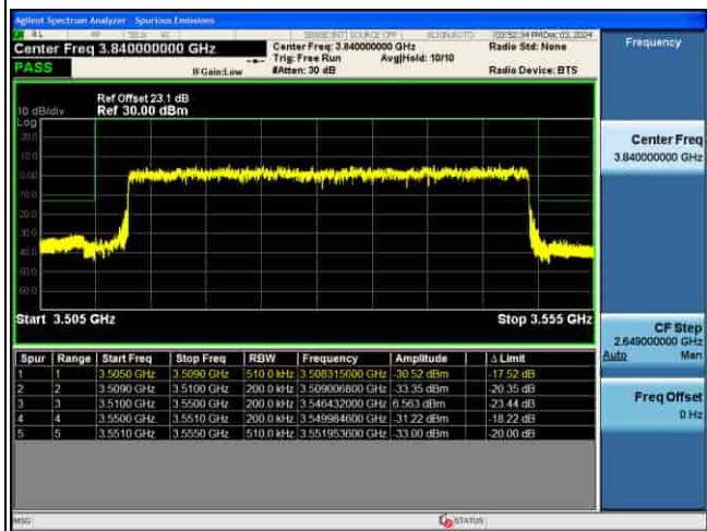
EDGE_5G_n77(K)_30KHz_P12-BPSK_50M_1RB@0_CH635000
