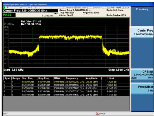
EDGE_5G_n77(K)_30KHz_P12-BPSK_20M_1RB@0_CH636000
