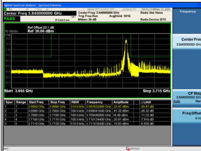
EDGE_4G_B43_QPSK_10M_FULL RB@0_CH44640
