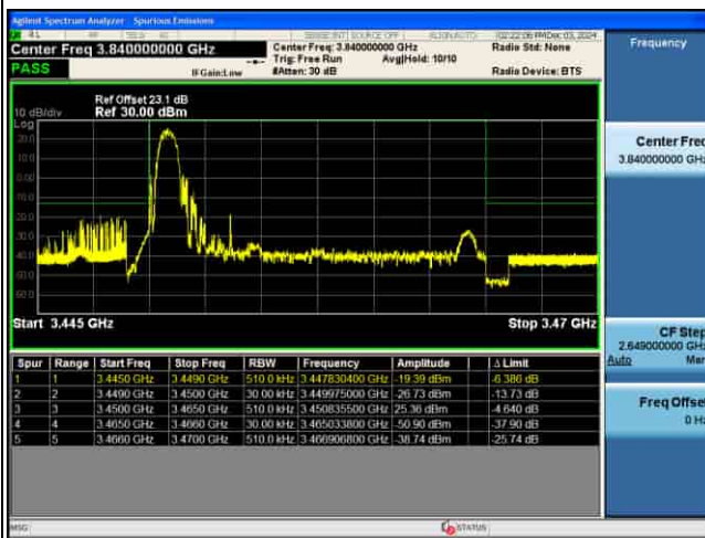
EDGE_5G_n77(K)_30KHz_P12-BPSK_15M_1RB@MAX_CH630500
