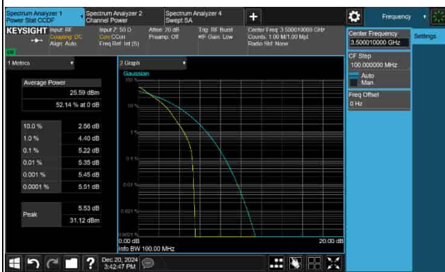
PAPR_5G_n77_30KHz_15M_3500.01MHz-16QAM
