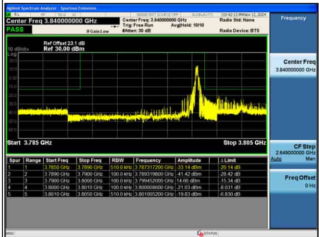
EDGE_4G_B43_QPSK_10M_FULL RB@0_CH45540
