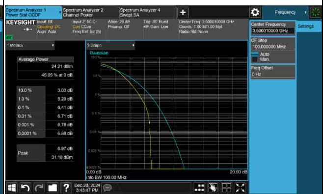
PAPR_5G_n77_30KHz_15M_3500.01MHz-64QAM
