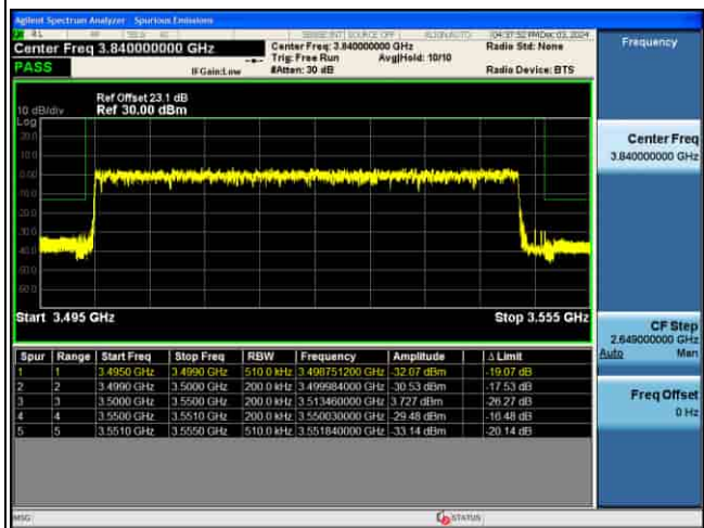
EDGE_5G_n77(K)_30KHz_Pi2-BPSK_50M_FULL RB@MAX_CH635000
