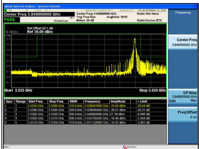
EDGE_4G_B42_QPSK_20M_FULL RB@0_CH42990
