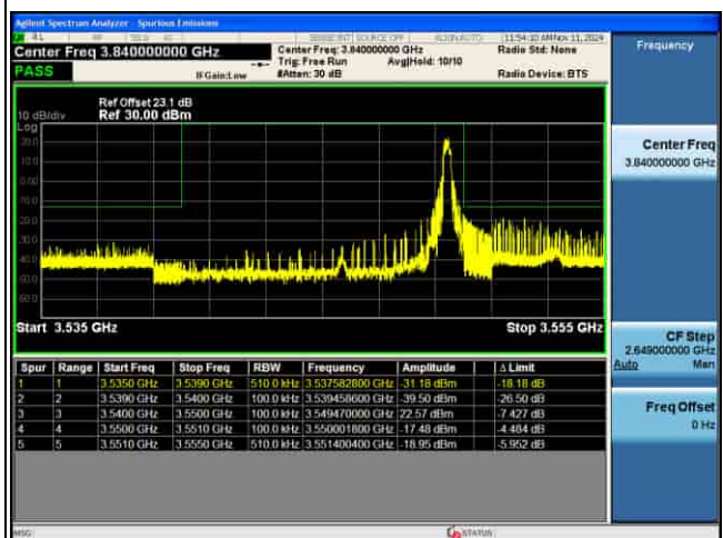
EDGE_4G_B42_QPSK_10M_FULL RB@0_CH43040
