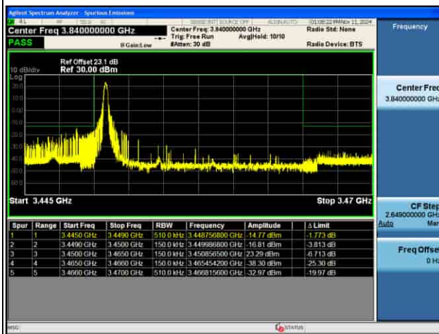
EDGE_4G_B42_QPSK_15M_1RB@MAX_CH42165
