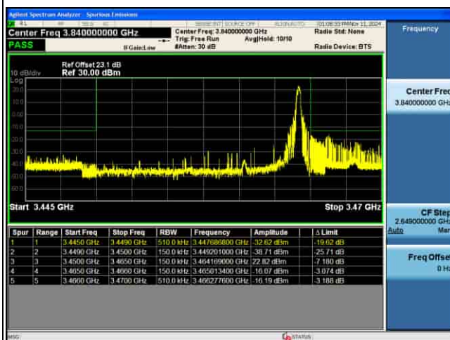
EDGE_4G_B42_QPSK_15M_FULL RB@0_CH42165
