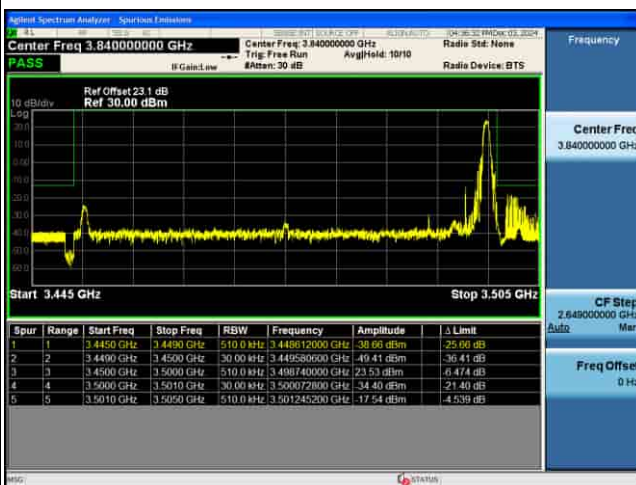
EDGE_5G_n77(K)_30KHz_P12-BPSK_50M_1RB@MAX_CH631668
