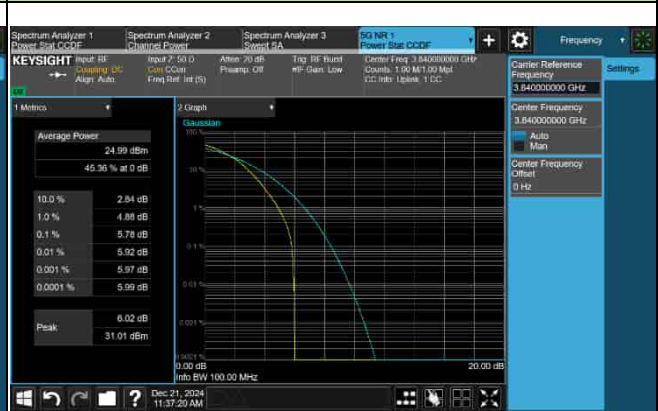
PAPR_5G_n77_30KHz_20M_3840MHz-64QAM
