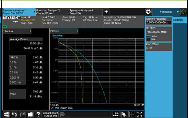
PAPR_5G_n77_30KHz_50M_3500.01MHz-64QAM
