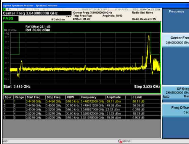
EDGE_5G_n77(K)_30KHz_P12-BPSK_70M_FULL RB@0_CH632334
