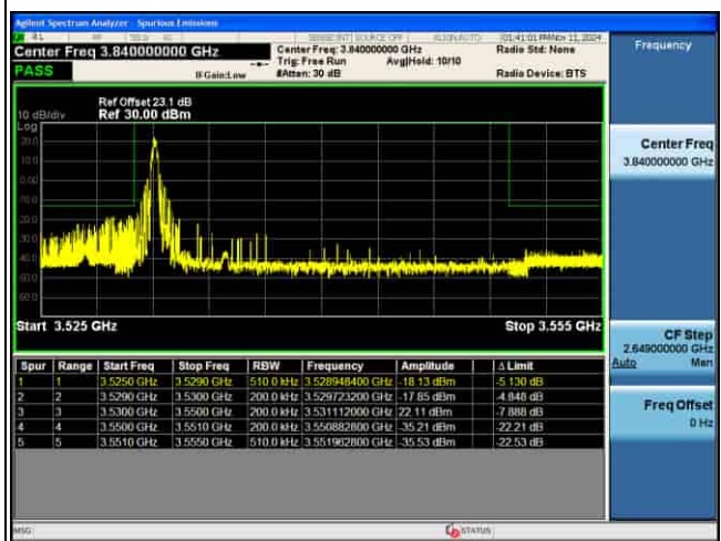
EDGE_4G_B42_QPSK_20M_1RB@MAX_CH42990
