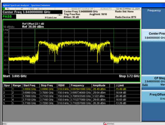
EDGE_4G_B43_QPSK_15M_FULL RB@0_CH44665
