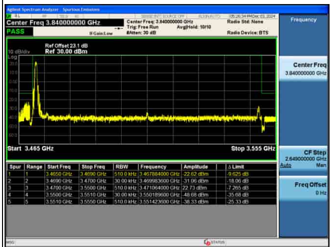
EDGE_5G_n77(K)_30KHz_P12-BPSK_80M_1RB@MAX_CH634000
