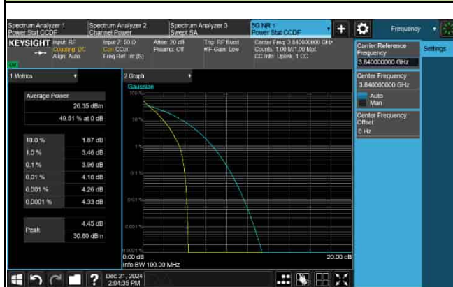
PAPR_5G_n77_30KHz_90M_3840MHz-16QAM
