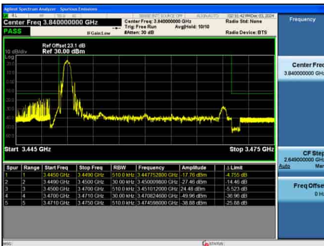
EDGE_5G_n77(K)_30KHz_P12-BPSK_20M_1RB@MAX_CH630668
