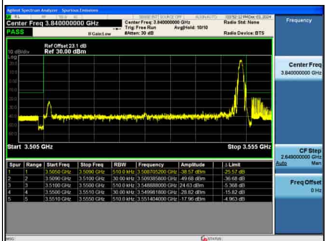
EDGE_5G_n77(K)_30KHz_P12-BPSK_40M_FULL RB@0_CH635332
