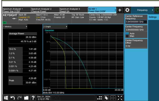
PAPR_5G_n77_30KHz_100M_3840MHz-16QAM
