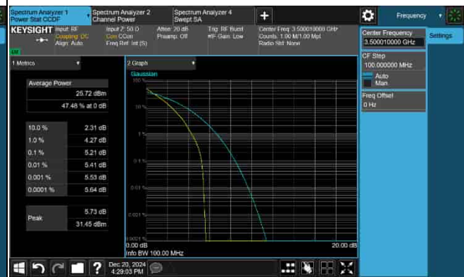
PAPR_5G_n77_30KHz_90M_3500.01MHz-64QAM
