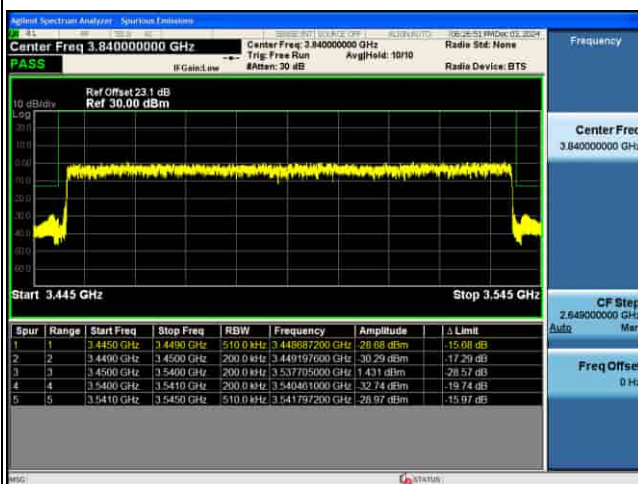
EDGE_5G_n77(K)_30KHz_Pi2-BPSK_100M_1RB@0_CH633334
