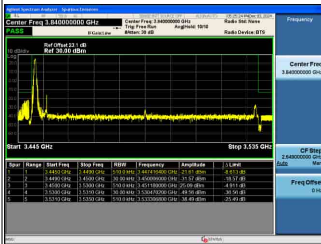
EDGE_5G_n77(K)_30KHz_P12-BPSK_80M_1RB@MAX_CH632668
