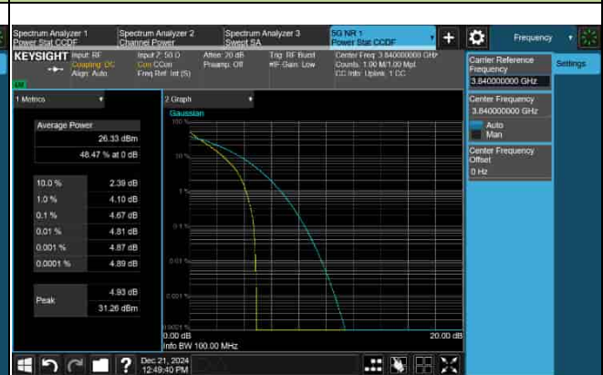
PAPR_5G_n77_30KHz_50M_3840MHz-64QAM
