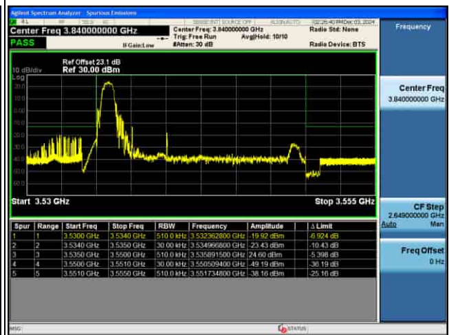
EDGE_5G_n77(K)_30KHz_P12-BPSK_15M_1RB@MAX_CH636166
