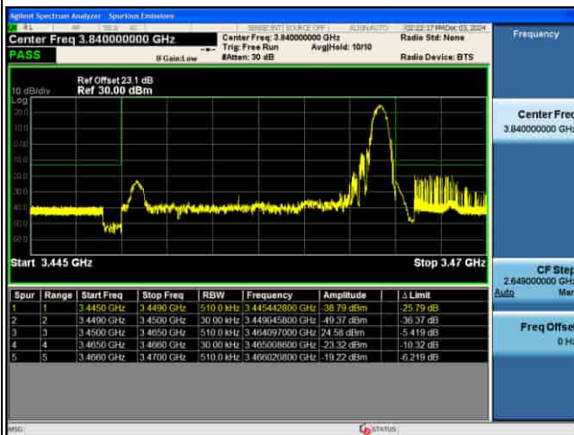
EDGE_5G_n77(K)_30KHz_P12-BPSK_15M_FULL RB@0_CH630500
