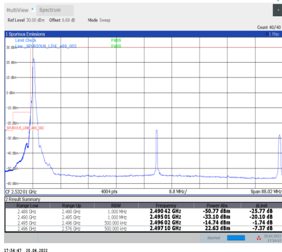
1-N41--30-80-L-1-DFT-PI2BPSK-Edge_1RB_Left-1@0-Ant0-PASS-see graph
