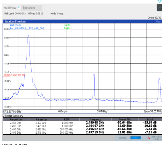
1-N41--30-50-L-4-CP-QPSK-Edge_1RB_Left-1@0-Ant0-PASS-see graph
