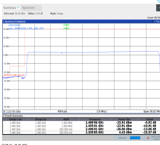
1-N41--30-50-L-6-CP-QPSK-Outer_Full-133@0-Ant0-PASS-see graph
