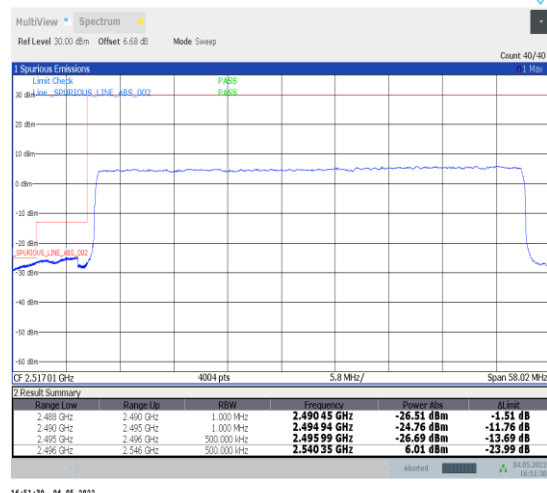
1-N41--30-50-L-3-DFT-PI2BPSK-Outer_Full-128@0-Ant0-PASS-see graph
