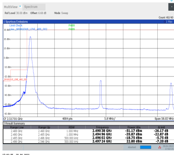
1-N41--30-50-L-1-DFT-PI2BPSK-Edge_1RB_Left-1@0-Ant0-PASS-see graph
