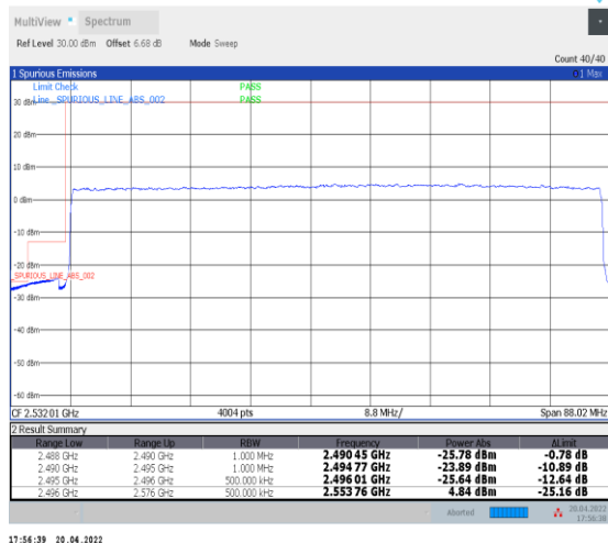
1-N41--30-80-L-3-DFT-PI2BPSK-Outer_Full-216@0-Ant0-PASS-see graph
