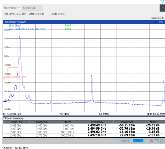
1-N41--30-80-L-4-CP-QPSK-Edge_1RB_Left-1@0-Ant0-PASS-see graph
