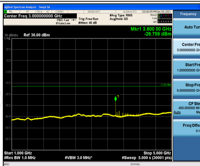
Band5-3MHz-QPSK-20415-1RB#0-Range5:5000~12000MHz
