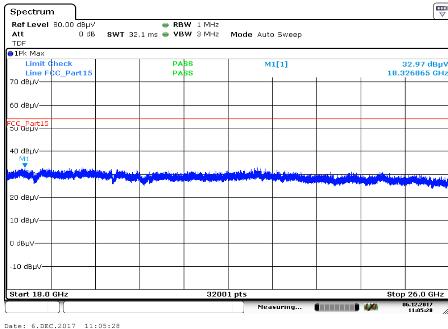
Plot 2: Middle channel, 18 GHz to 26 GHz, vertical & horizontal polarization, peak & average
