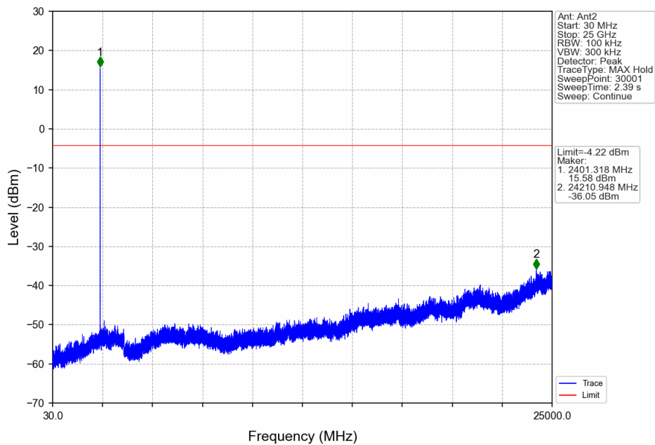
1M_LCH_2402MHz_Ant2_NTNV
