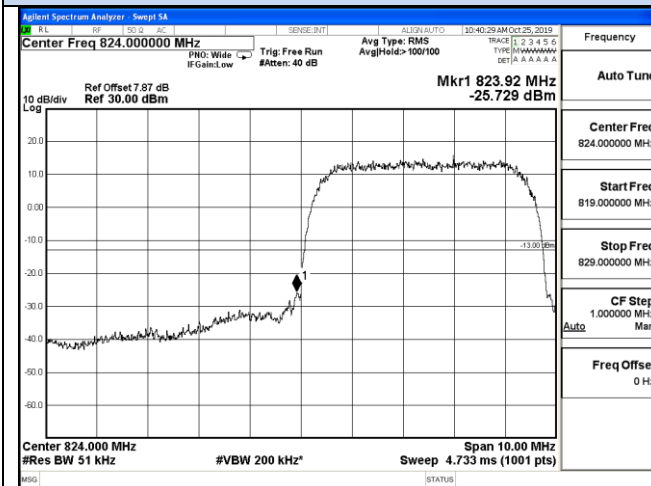
Channel 4132 / 826.4 MHz
