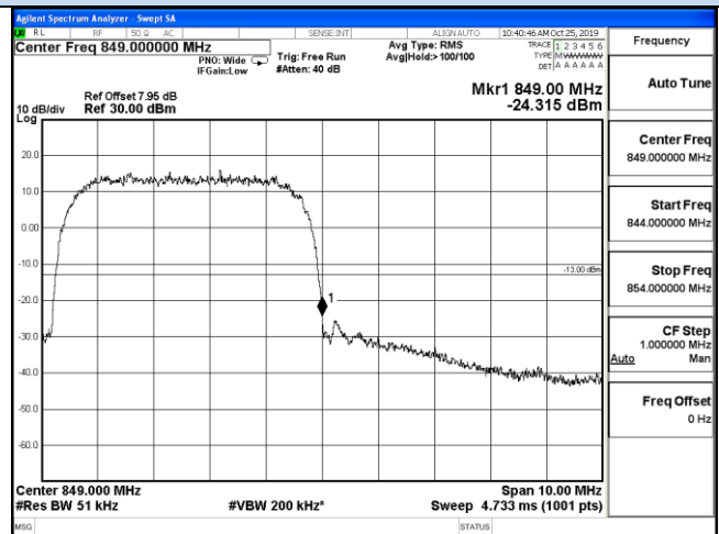
Channel 4233 / 846.6 MHz
