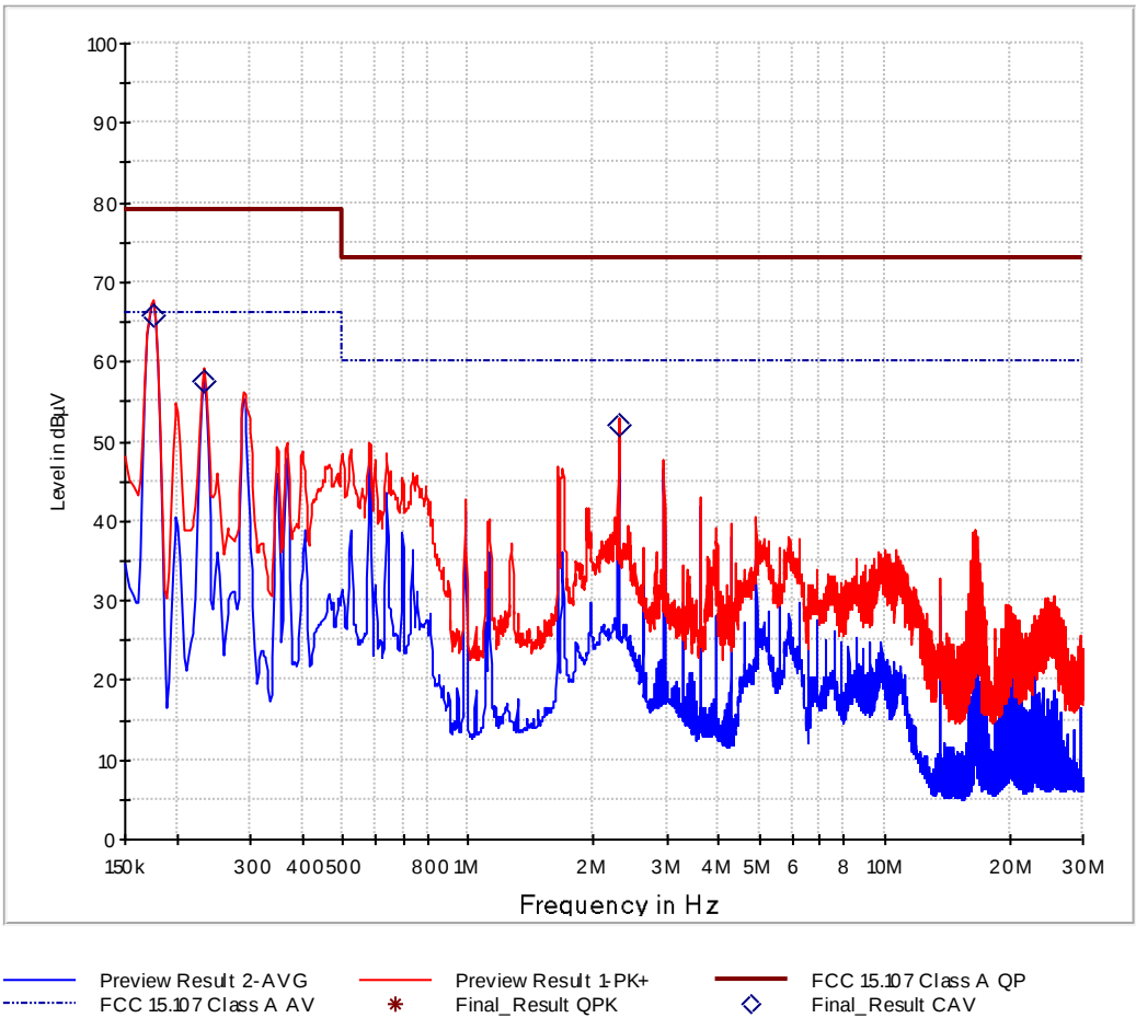
Line Minus - 150 kHz to 30 MHz
