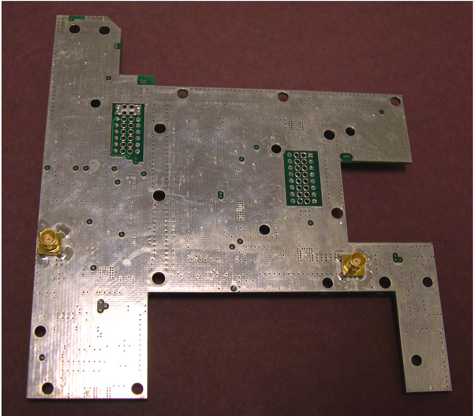
Digivance Street Coverage Solution (SCS) Power Amplifier 4244602E Rev A Board Back
