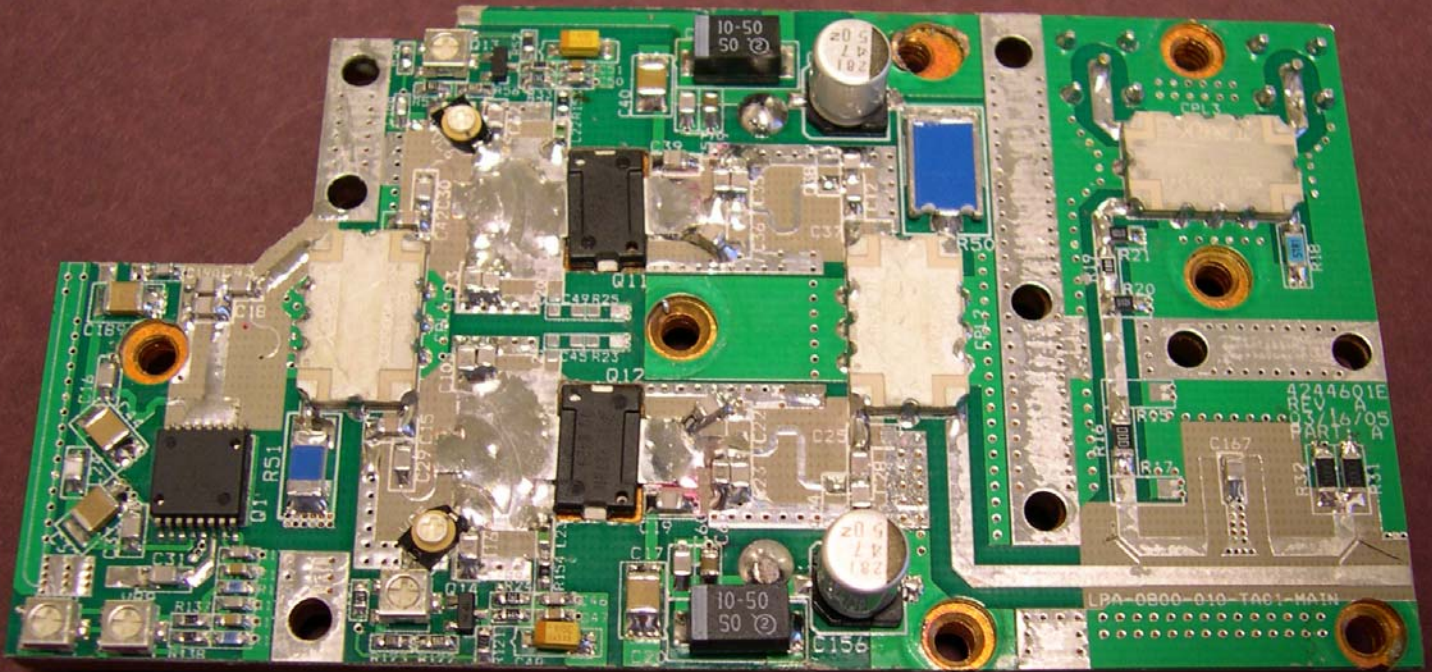
Digivance Street Coverage Solution (SCS) Power Amplifier 4244601E Rev A Board Front
