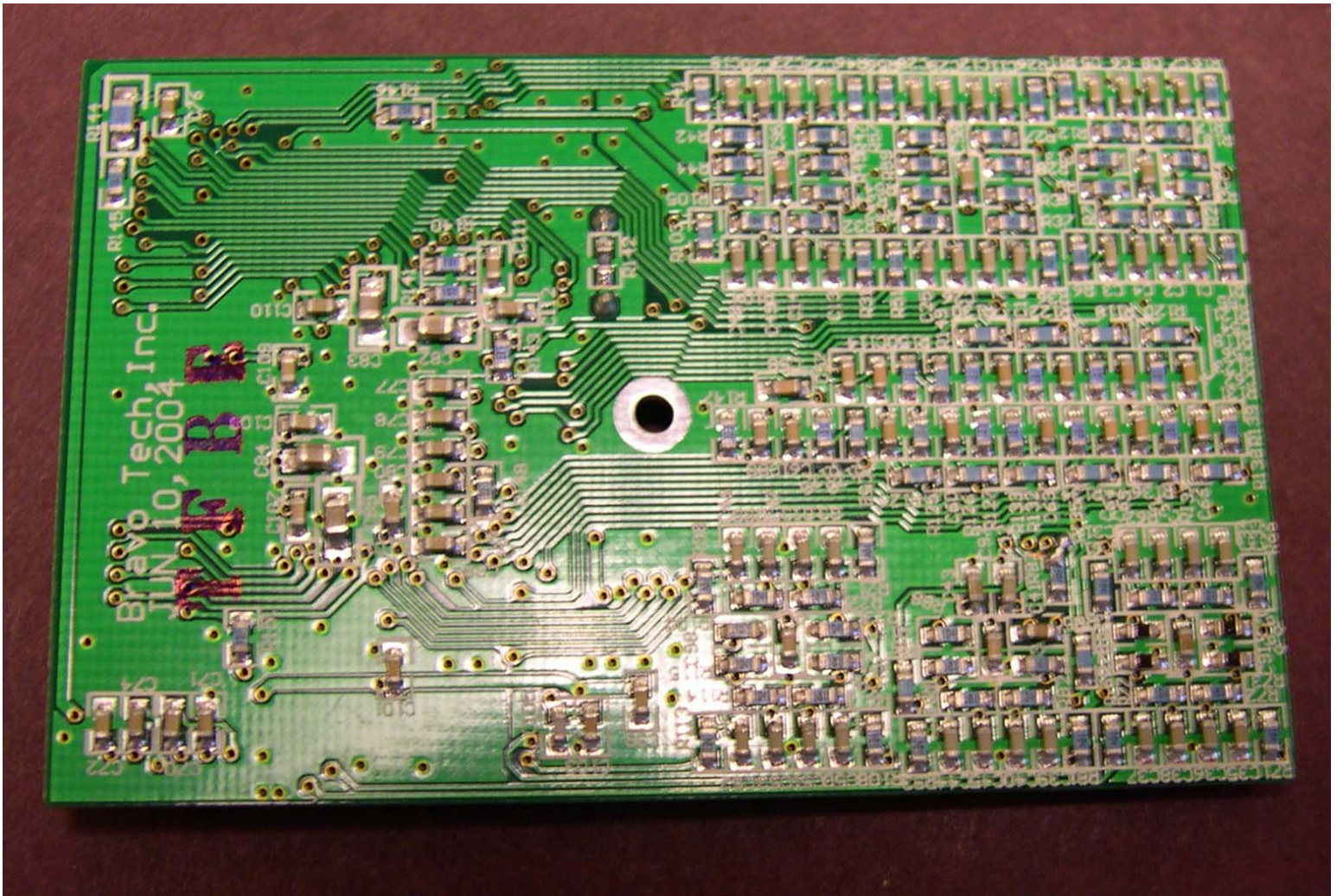
Digivance Street Coverage Solution (SCS) Power Amplifier Universal II 003 Board Back
