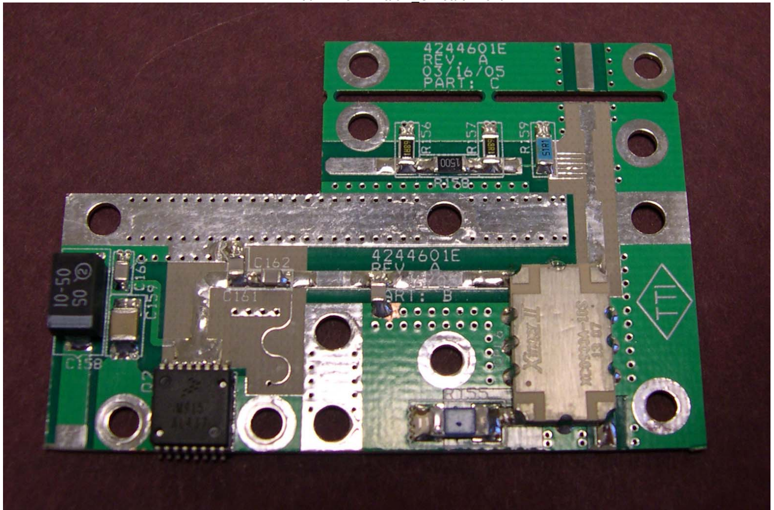
Digivance Street Coverage Solution (SCS) Power Amplifier 4244601E Rev A Part B C Board Front
