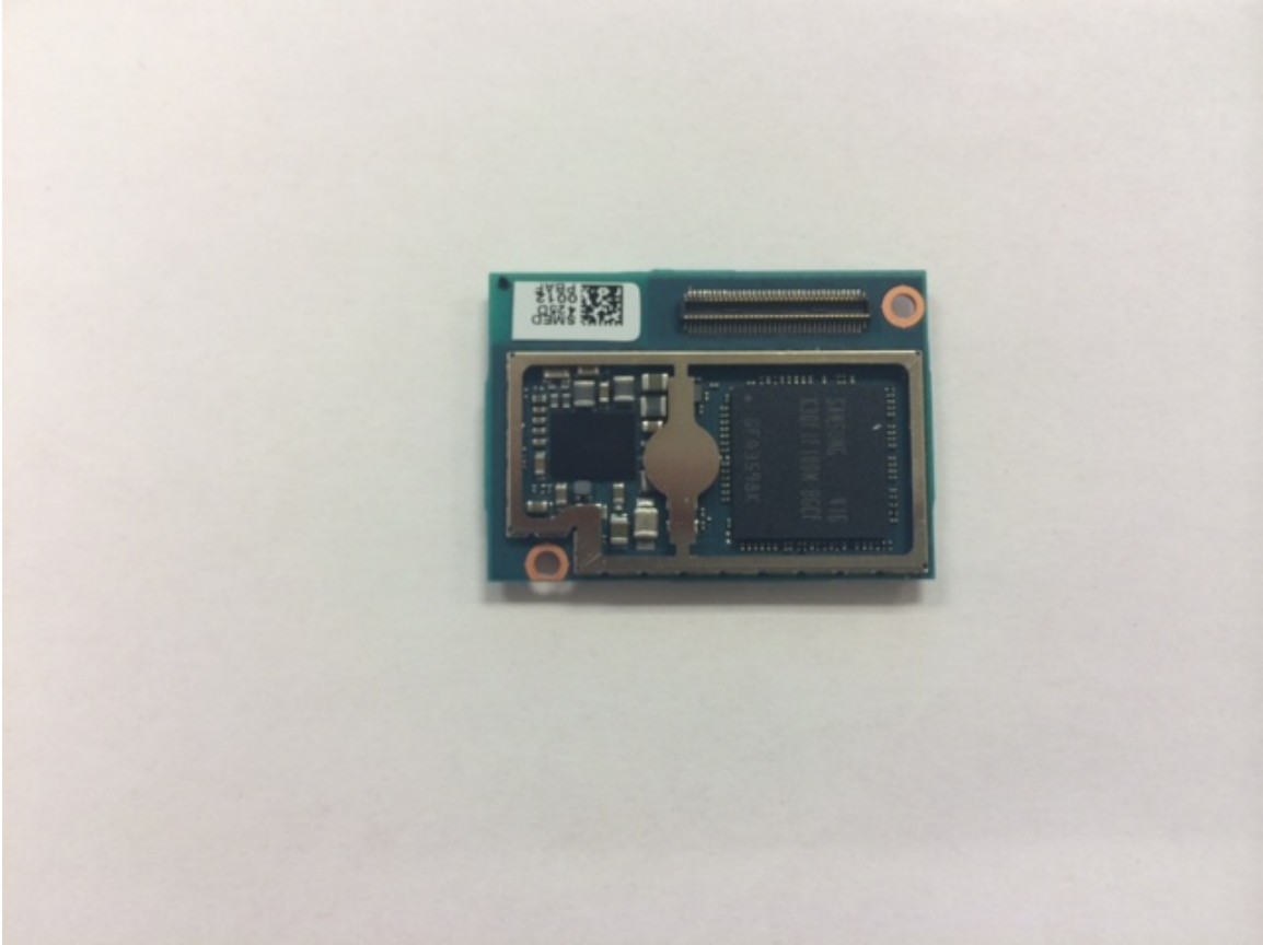
Edison back without shield
