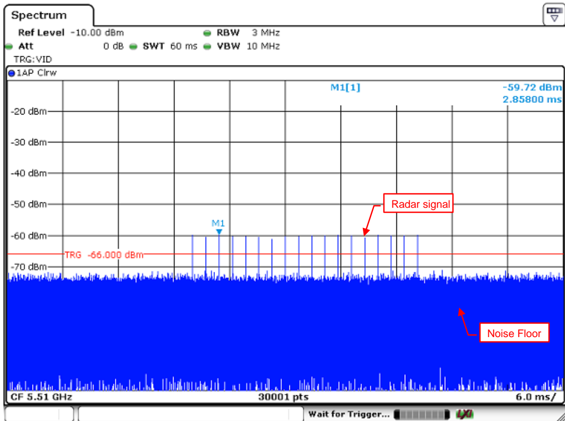
Radar Signal 0
