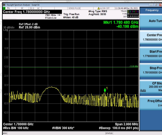
Band66-5MHz-QPSK-132647-1RB#24
