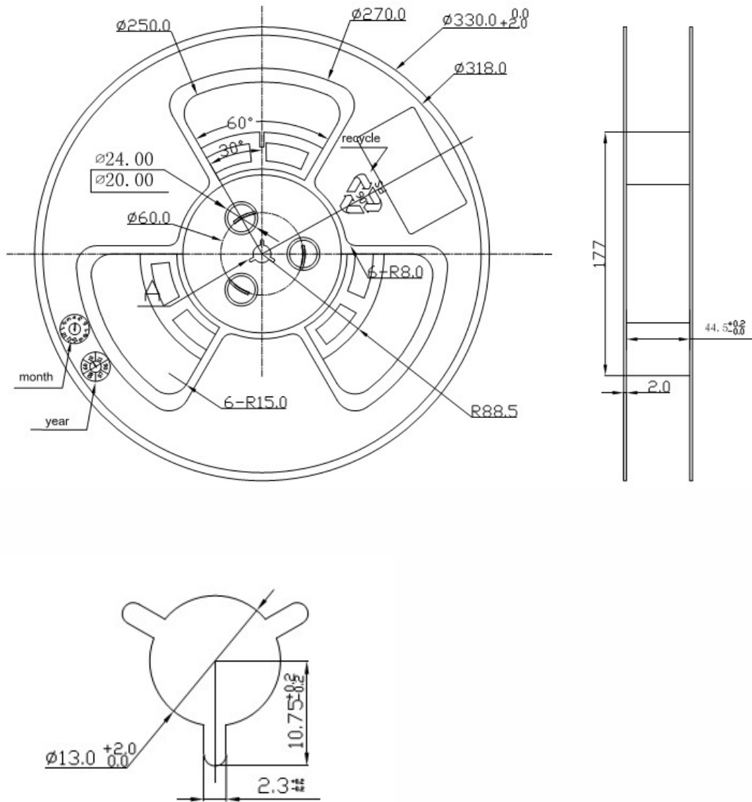
Figure 35: Reel Detail
