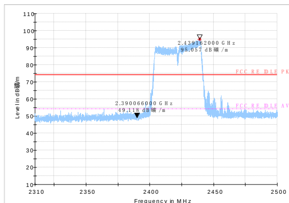
Peak detector
