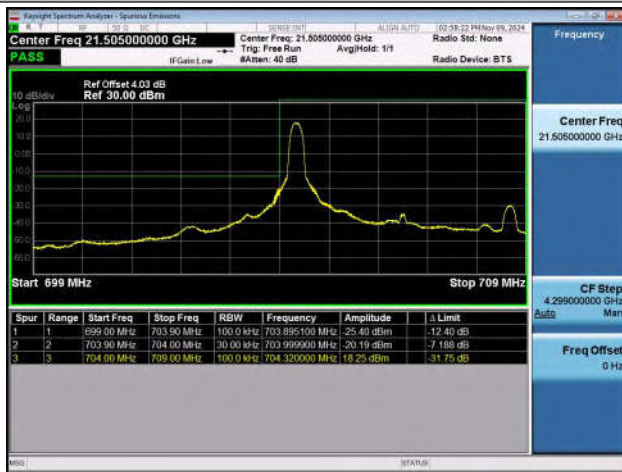
Band17_5MHz_QPSK_23825_1RB#24
