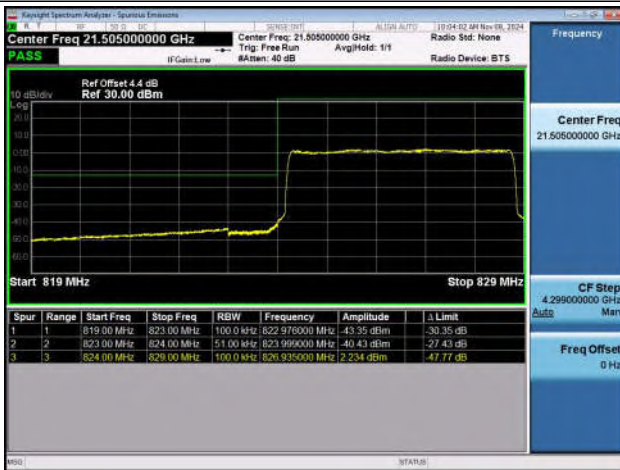
Band5_5MHz_QPSK_20425_25RB#0
