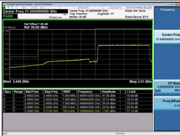
Band7_10MHz_QPSK_20800_50RB#0
