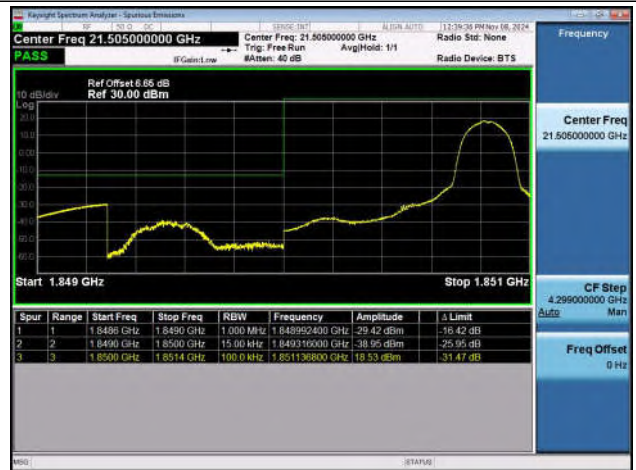
Band25_1.4MHz_QPSK_26047_1RB#5
