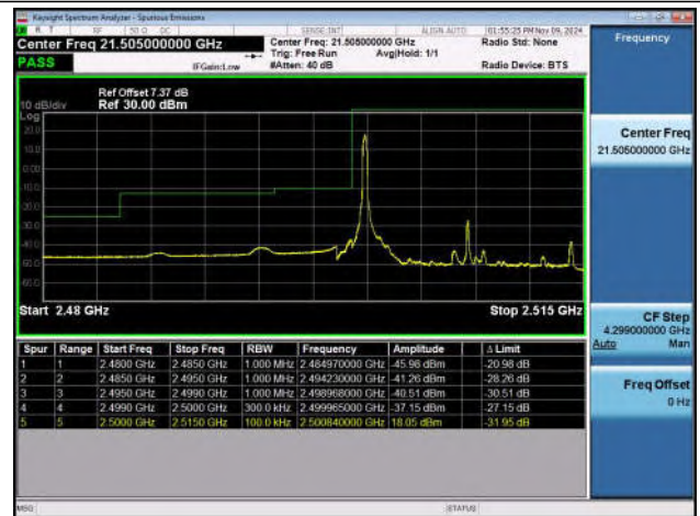
Band7_15MHz_QPSK_21375_1RB#74
