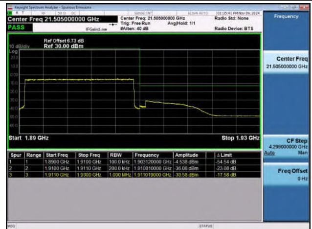
Band2_20MHz_QPSK_19100_100RB#0
