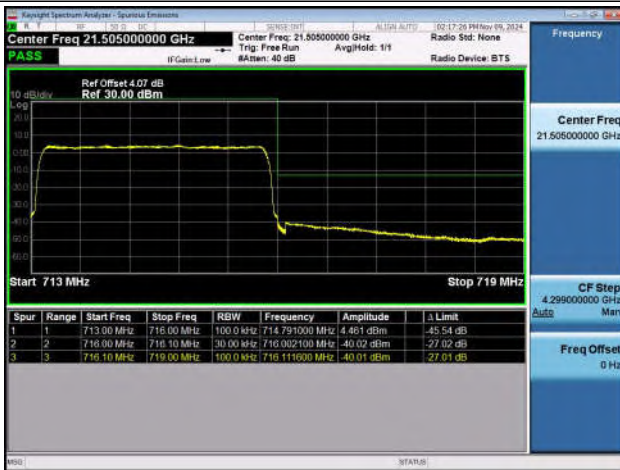
Band12_3MHz_QPSK_23165_15RB#0
