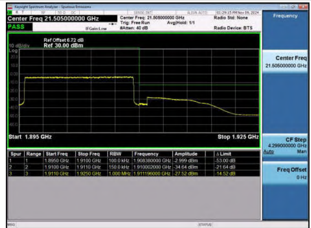
Band2_20MHz_QPSK_18700_100RB#0
