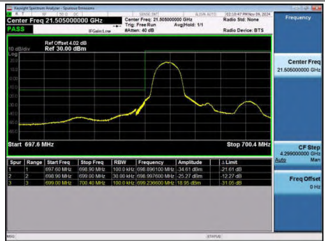
Band12_1.4MHz_QPSK_23173_1RB#5
