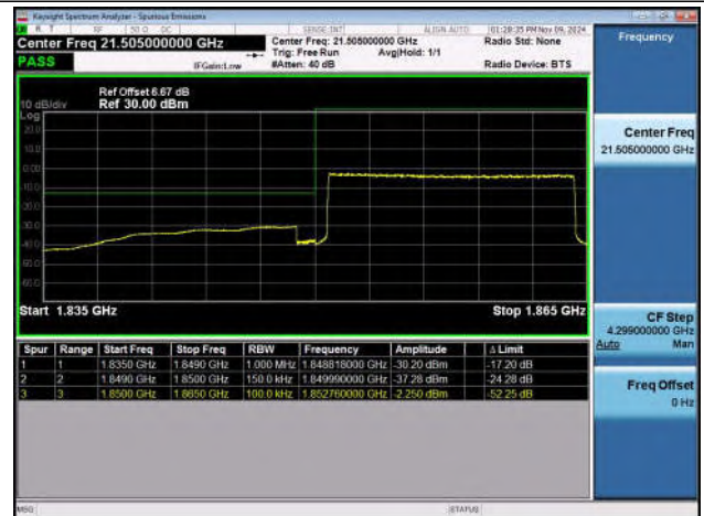
Band2_15MHz_QPSK_18675_75RB#0
