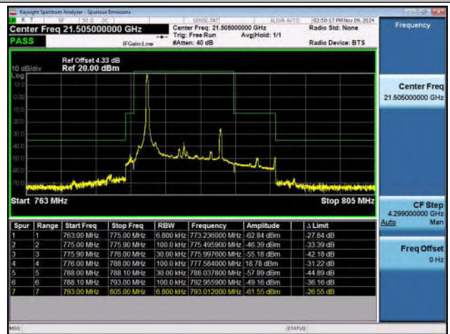
Band13_10MHz_QPSK_23230_1RB#0
