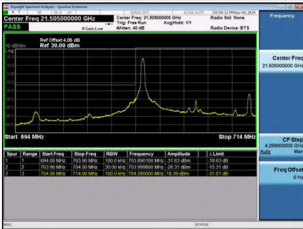
Band17_10MHz_QPSK_23800_1RB#49
