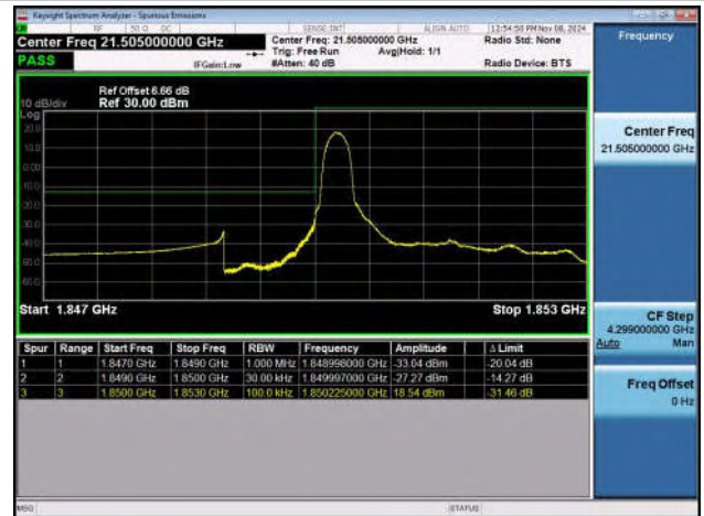
Band25_3MHz_QPSK_26055_15RB#0
