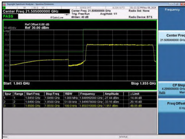
Band25_10MHz_QPSK_26090_50RB#0
