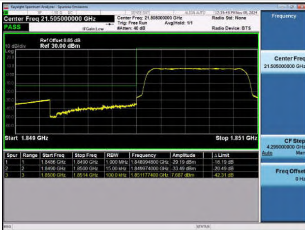
Band25_3MHz_QPSK_26055_1RB#14
