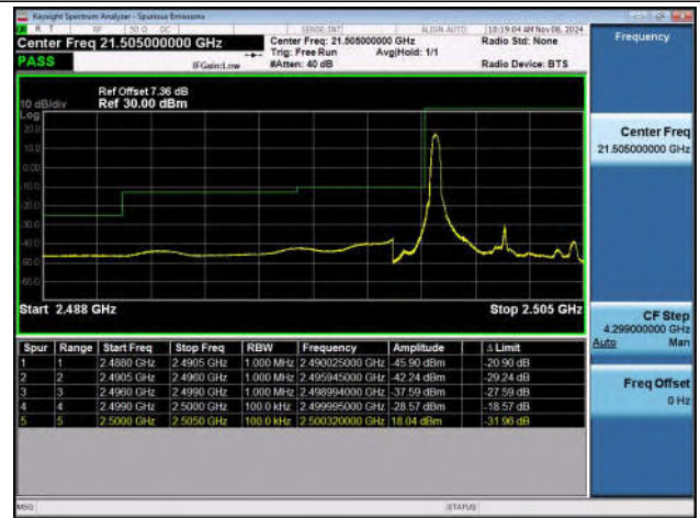
Band7_5MHz_QPSK_20775_1RB#0
