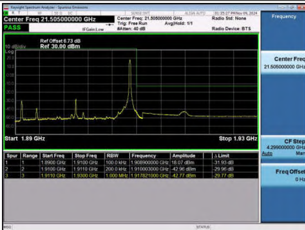
Band2_20MHz_QPSK_19100_1RB#99
