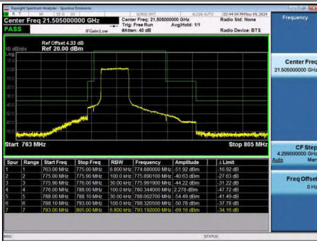
Band13_5MHz_QPSK_23255_25RB#0
