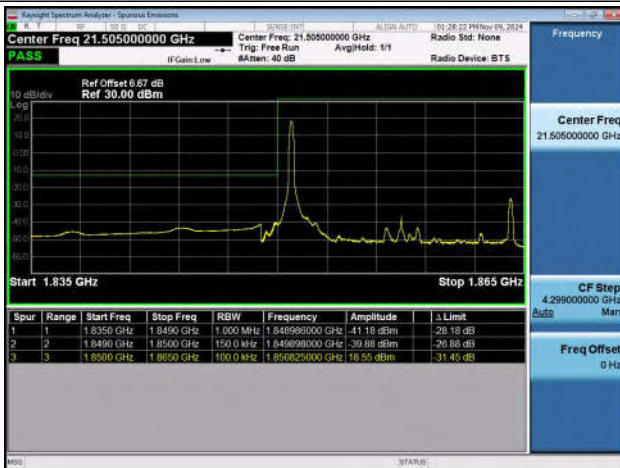
Band2_15MHz_QPSK_18675_1RB#0
