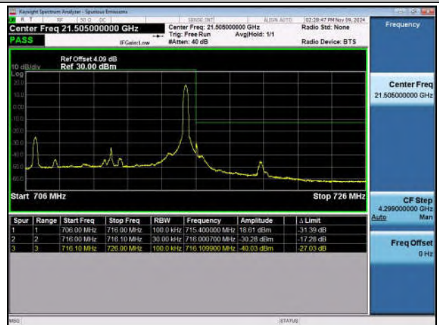
Band12_10MHz_QPSK_23130_1RB#49
