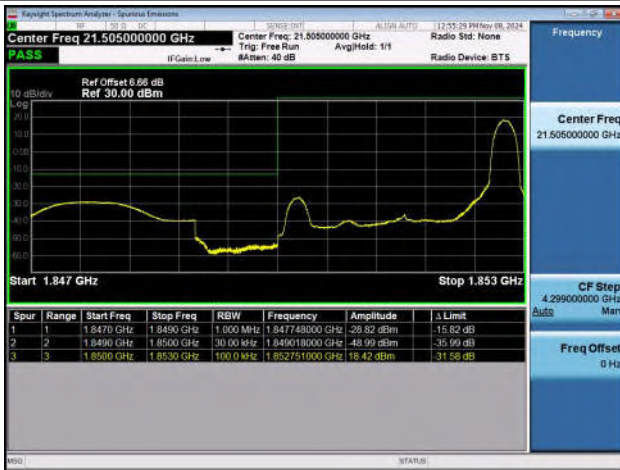
Band25_5MHz_QPSK_26065_1RB#0
