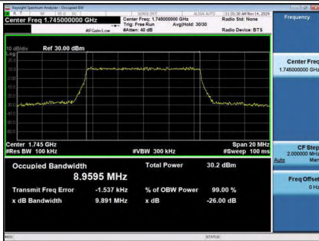
Band66-10MHz-QPSK-132322-50RB#0-PASS
