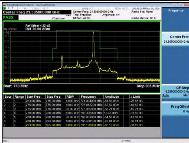
Band17_5MHz_QPSK_23755_1RB#0
