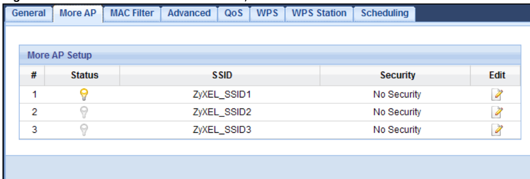
Figure 37 Network > Wireless LAN 2.4G/5G > More AP
