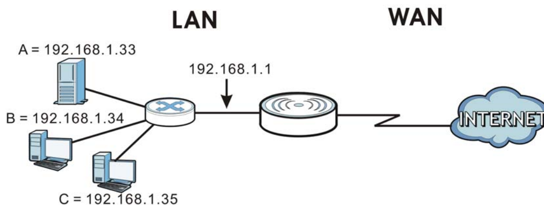
Figure 61 Multiple Servers Behind NAT Example
