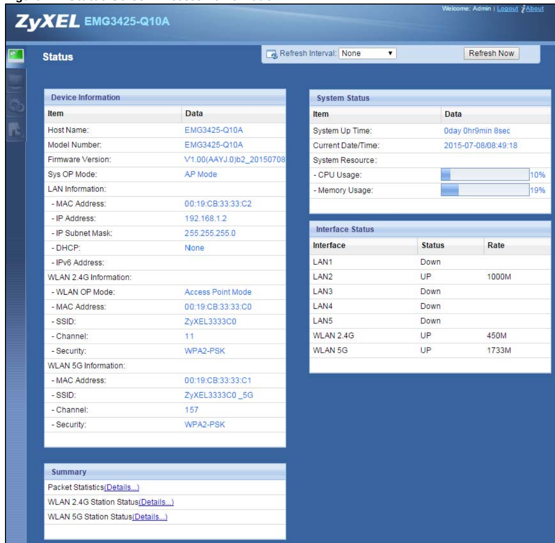
Figure 14 Status Screen: Access Point Mode
