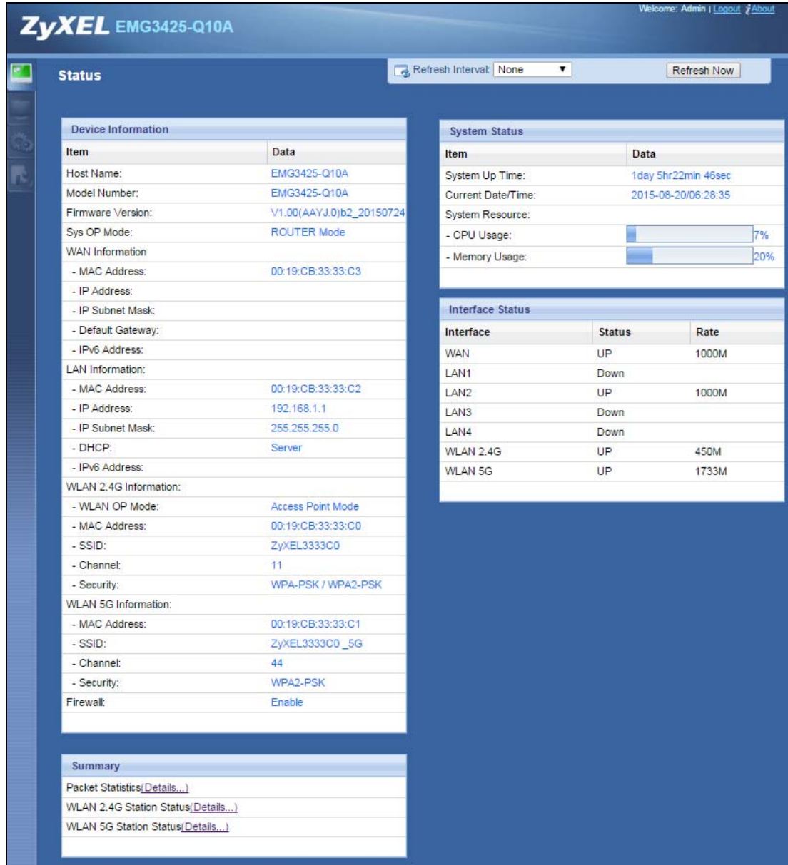
Figure 9 Status Screen: Router Mode
