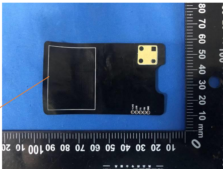
Receiving antenna
