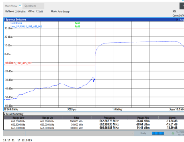
1-N71-PC3-15-5-L-3-DFT-PI2BPSK-Outer_Full-25@0-Ant0-1--PASS-see graph
