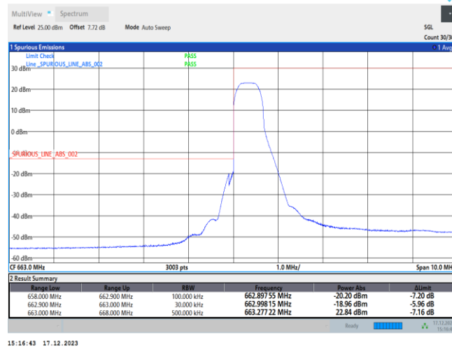
1-N71-PC3-15-5-L-1-DFT-PI2BPSK-Edge_1RB_Left-1@0-Ant0-1--PASS-see graph
