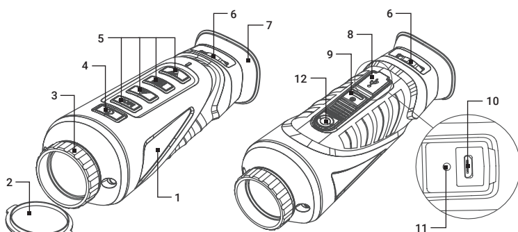
FIGURE 1-1. MAIN PARTS
