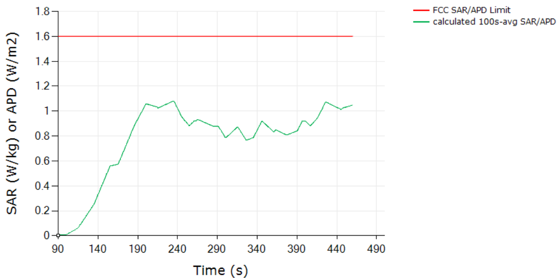
SAR (or APD) (Test Sequence 2) Tech: LTE, Band 25
