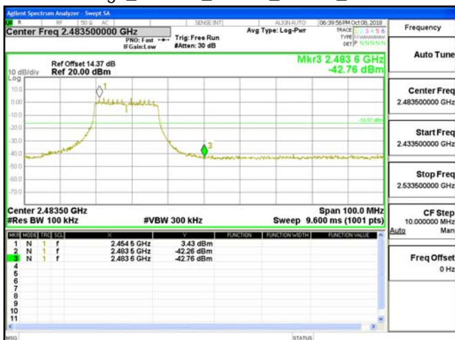
Band Edge_802.11n_20MHz_Chain0_2462MHz
