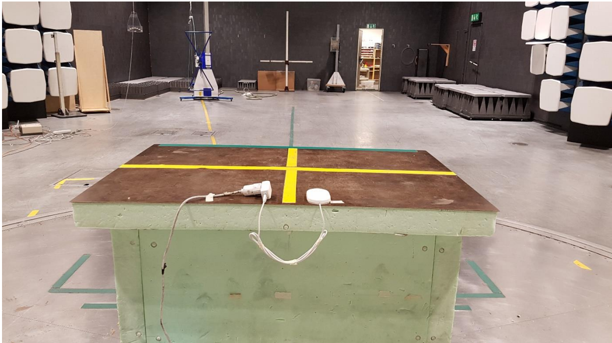
Photo of the test setup for radiated emission
