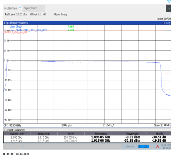
1-N25--15-20-H-6-CP-QPSK-Outer_Full-106@0-A nt0-seegraph-PASS-see graph
