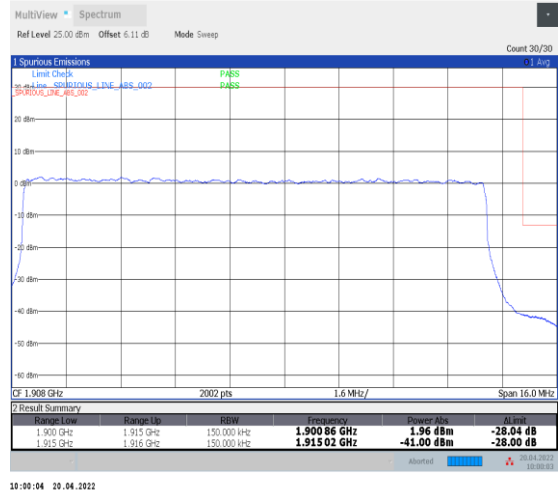
1-N25--15-15-H-3-DFT-PI2BPSK-Outer_Full-75@ 0-Ant0-seegraph-PASS-see graph
