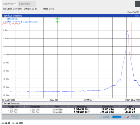
1-N25--15-15-H-2-DFT-PI2BPSK-Edge_1RB_Right-1 @78-Ant0-seegraph-PASS-see graph
