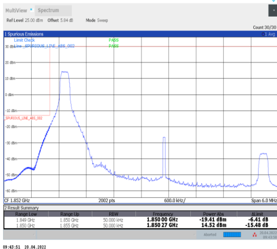
1-N25--15-5-L-4-CP-QPSK-Edge_1RB_Left-1@0-Ant0-seegraph-PASS-see graph
