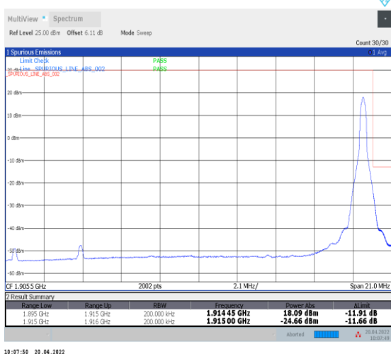
1-N25--15-20-H-5-CP-QPSK-Edge_1RB_Right-1@105 -Ant0-seegraph-PASS-see graph
