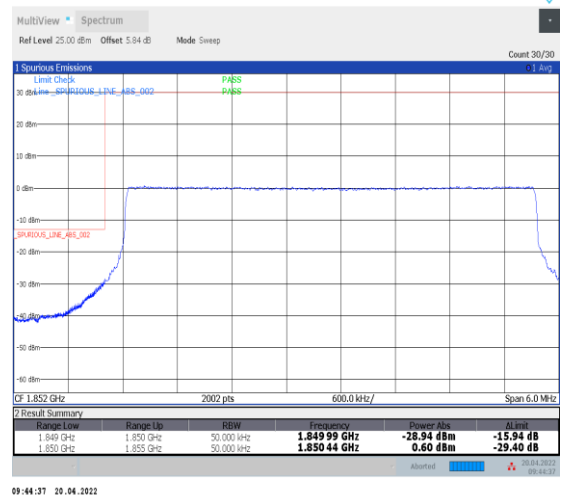
1-N25--15-5-L-6-CP-QPSK-Outer_Full-25@0-Ant0-seegraph-PASS-see graph
