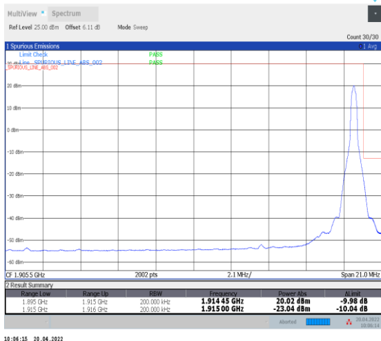
1-N25--15-20-H-2-DFT-PI2BPSK-Edge_1RB_Right-1 @105-Ant0-seegraph-PASS-see graph
