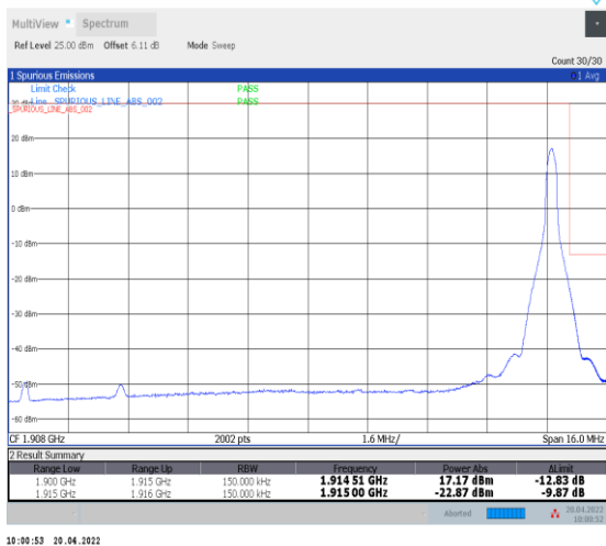
1-N25--15-15-H-5-CP-QPSK-Edge_1RB_Right-1@78- Ant0-seegraph-PASS-see graph
