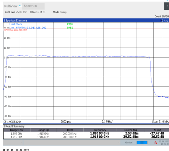
1-N25--15-20-H-3-DFT-PI2BPSK-Outer_Full-100 @0-Ant0-seegraph-PASS-see graph
