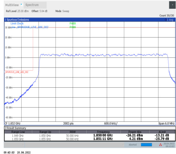
1-N25--15-5-L-3-DFT-PI2BPSK-Outer_Full-25@0-Ant0-seegraph-PASS-see graph
