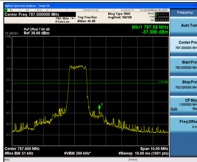
Band13-5MHz-16QAM-23255-6-0-High--37.40-PASS
