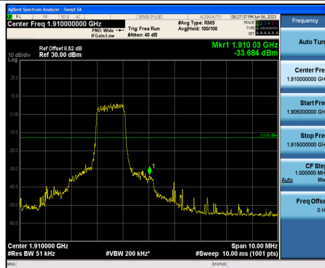
Band2-15MHz-16QAM-19125-6-0-High--33.68-PASS
