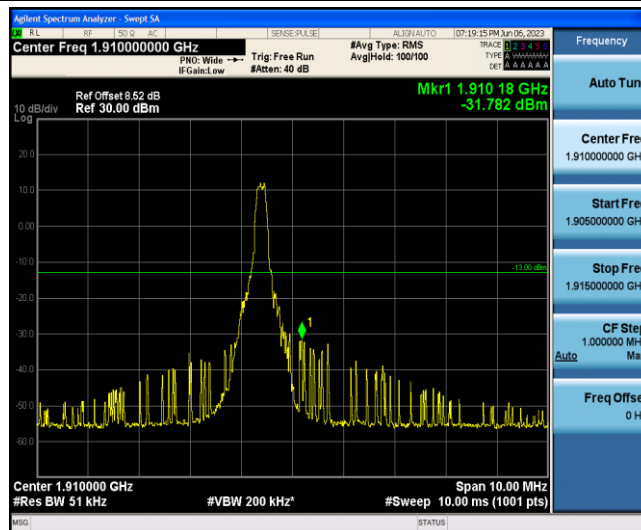
Band2-1.4MHz-16QAM-19193-1-5-High--31.78-PASS
