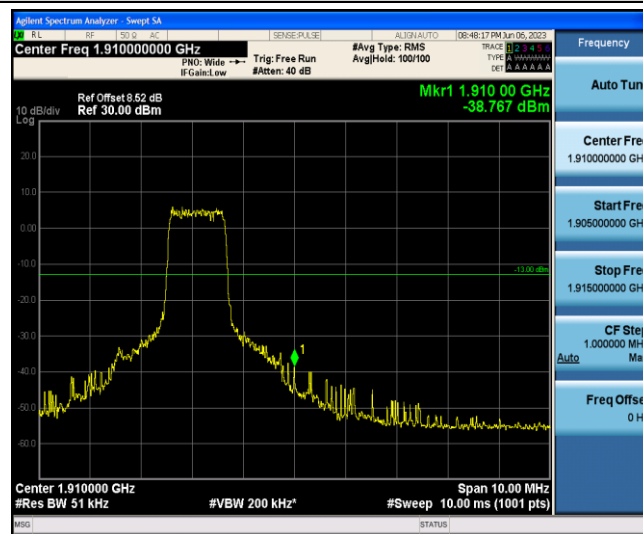
Band2-20MHz-QPSK-19100-6-0-High--38.77-PASS
