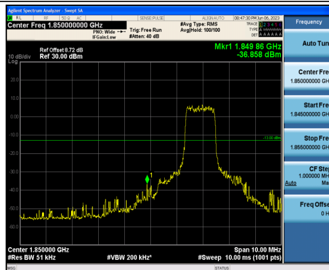
Band2-20MHz-QPSK-18700-6-0-Low--36.86-PASS
