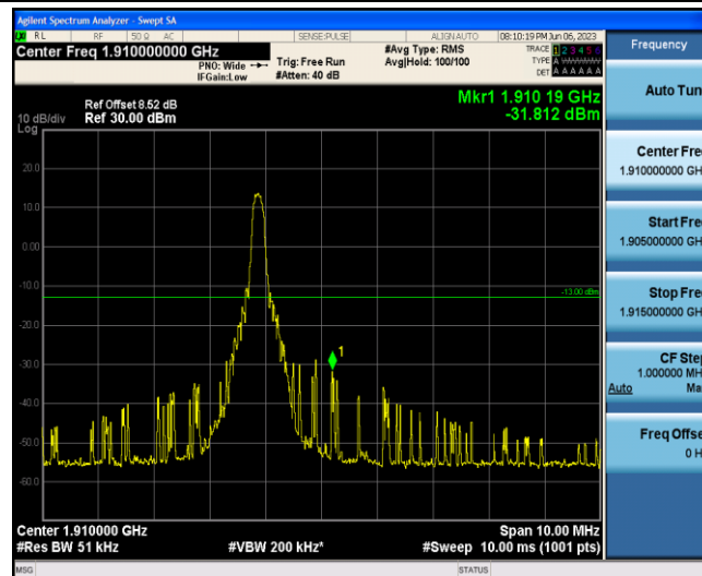
Band2-10MHz-QPSK-19150-1-5-High--31.81-PASS
