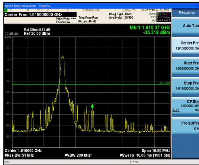
Band2-20MHz-QPSK-19100-1-5-High--35.32-PASS
