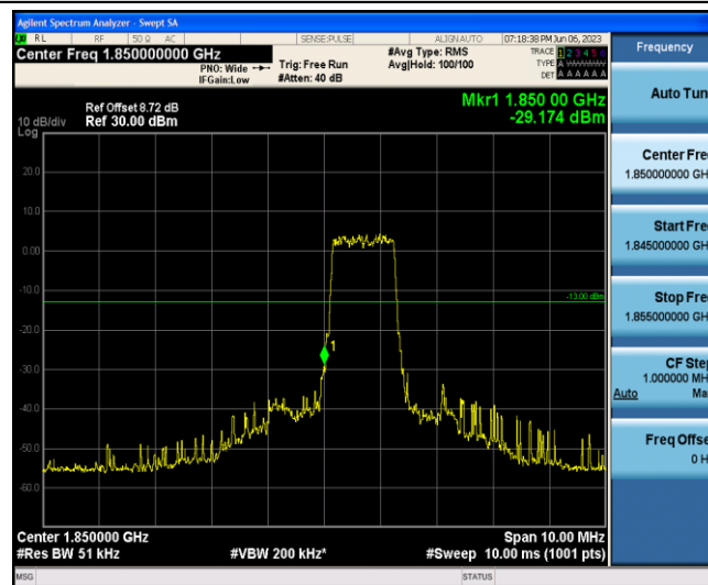
Band2-1.4MHz-QPSK-18607-6-0-Low--29.17-PASS
