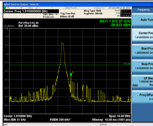
Band2-1.4MHz-QPSK-19193-1-5-High--26.62-PASS
