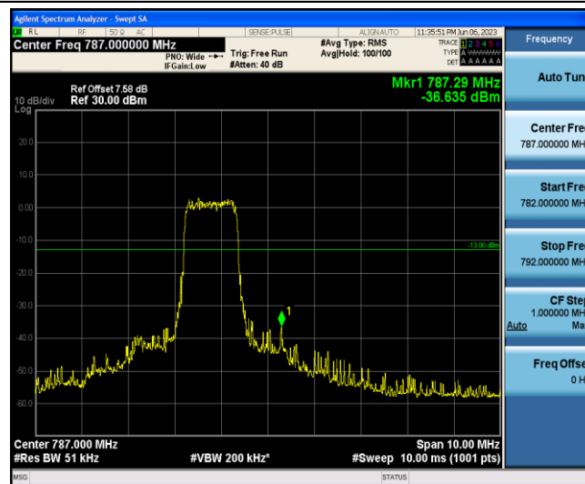
Band13-10MHz-QPSK-23230-6-0-High--36.64-PASS
