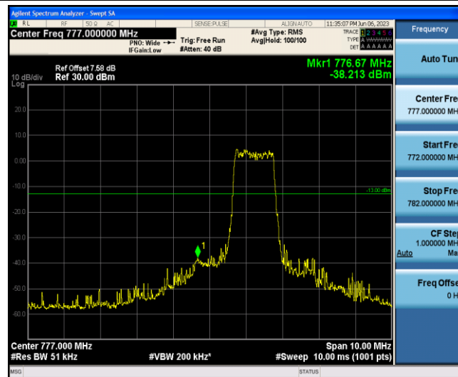
Band13-10MHz-QPSK-23230-6-0-Low--38.21-PASS
