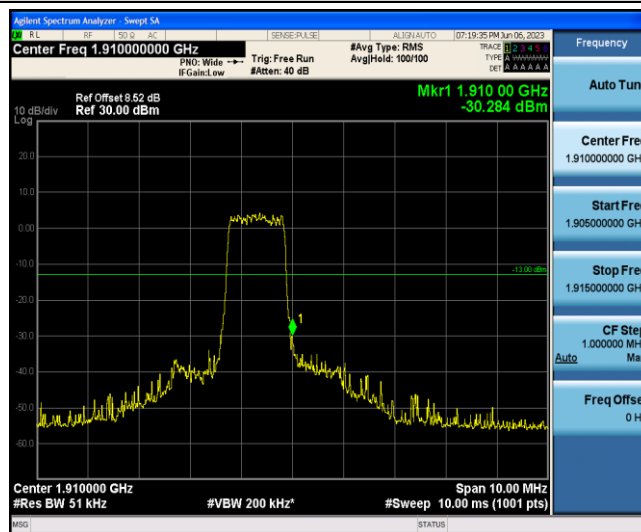
Band2-1.4MHz-16QAM-19193-6-0-High--30.28-PASS
