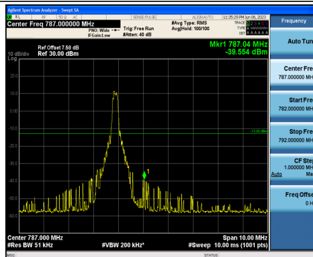
Band13-10MHz-QPSK-23230-1-5-High--39.55-PASS
