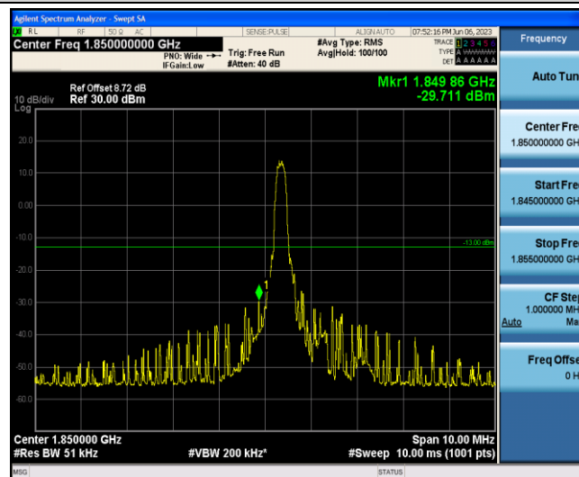
Band2-5MHz-16QAM-18625-1-0-Low--29.71-PASS
