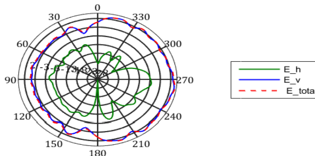
frequency=2450MHz, X-Y Plane
