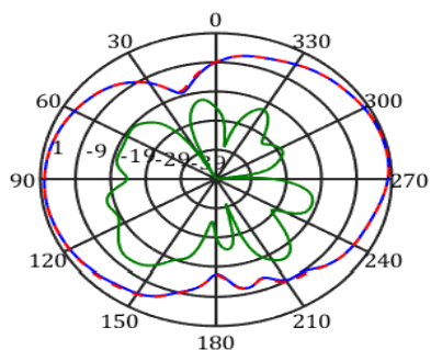
frequency=2450MHz, Y-Z Plane
