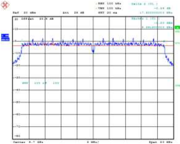
Figure 7-21: 6 dB Bandwidth
