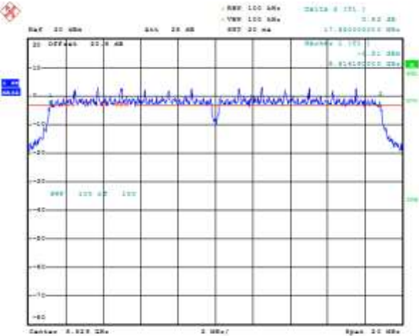
Figure 7-22: 6 dB Bandwidth
