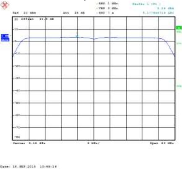
Figure 8-67: Peak Power Spectral Density SISO Secondary, 802.11ac, Channel 36, MCS0 Mbps
