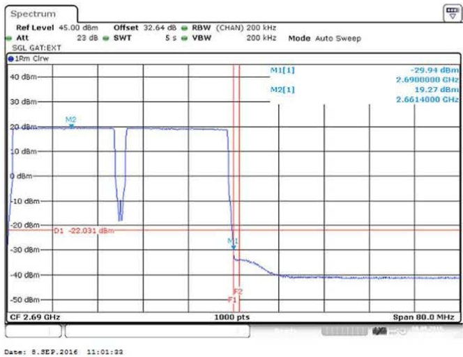
Figure 144 Spurious Emissions (Upper Band Edge) – QPSK (2660.0/2680.0 MHz) (2 X 20 MHz Channel BW)
