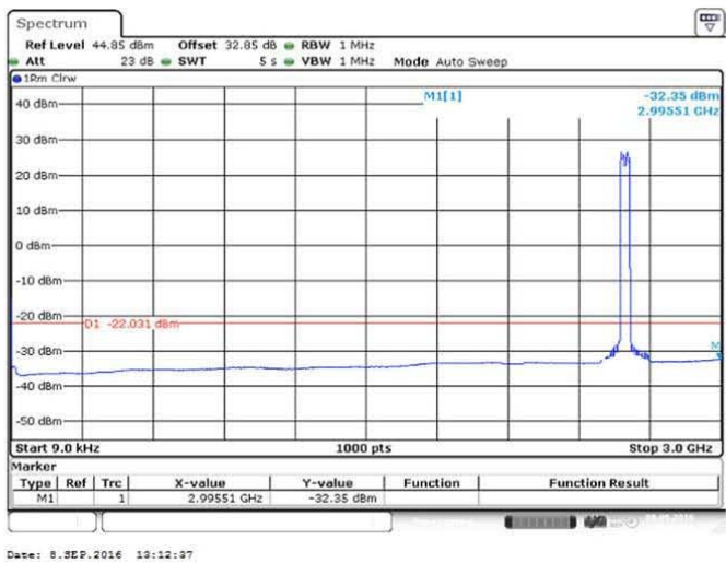
Figure 97 Spurious Emissions (9kHz – 3GHz) - QPSK (2583.0/2603.0 MHz) (2 X 20 MHz Channel BW)
