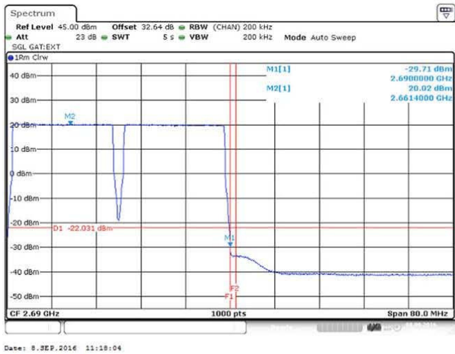
Figure 148 Spurious Emissions (Upper Band Edge) – 64QAM (2660.0/2680.0 MHz) (2 X 20 MHz Channel BW)
