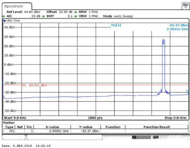
Figure 105 Spurious Emissions (9kHz – 3GHz) – 16QAM (2583.0/2603.0 MHz) (2 X 20 MHz Channel BW)
