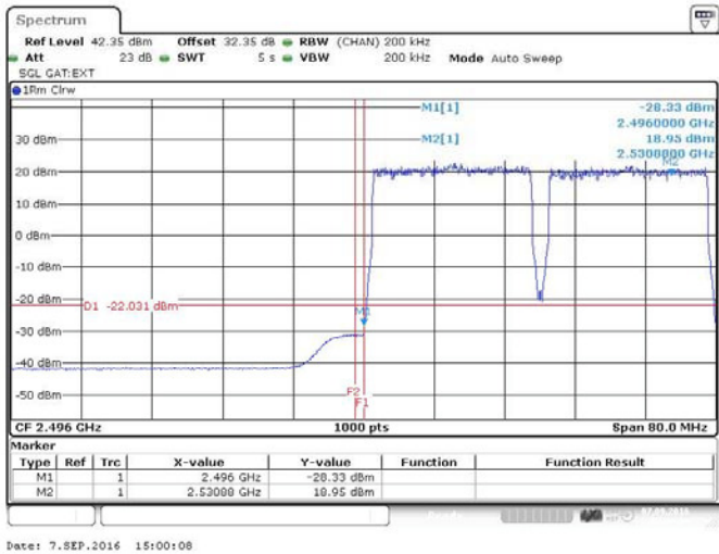
Figure 139 Spurious Emissions (Lower Band Edge) – 16QAM (2506.0/2526.0 MHz) (2 X 20 MHz Channel BW)
