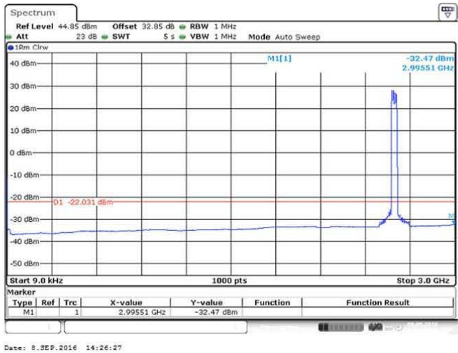
Figure 145 Spurious Emissions (9kHz – 3GHz) – QPSK (2583.0/2603.0 MHz) (2 X 20 MHz Channel BW)
