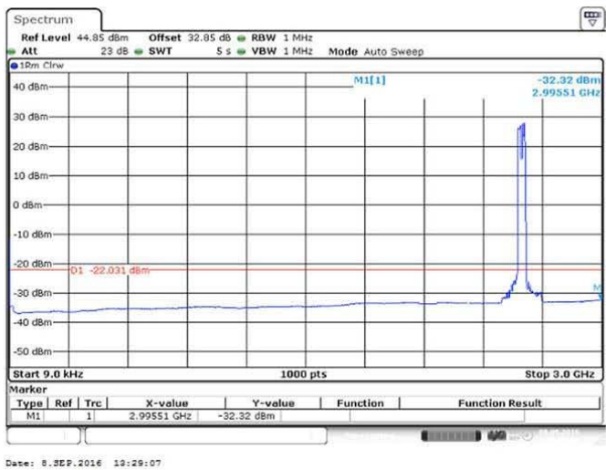
Figure 109 Spurious Emissions (9kHz – 3GHz) - QPSK (2583.0/2603.0 MHz) (2 X 20 MHz Channel BW)
