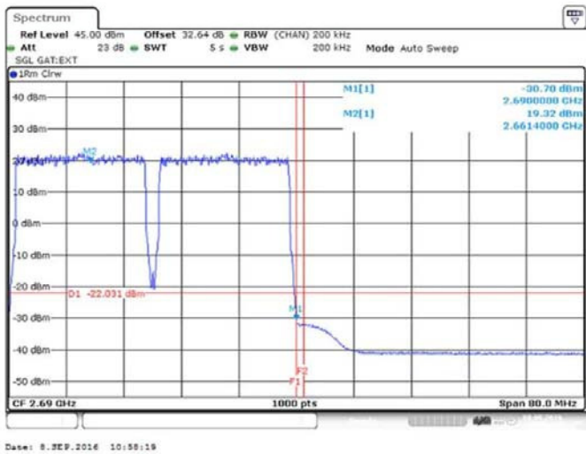
Figure 140 Spurious Emissions (Upper Band Edge) – 16QAM (2660.0/2680.0 MHz) (2 X 20 MHz Channel BW)
