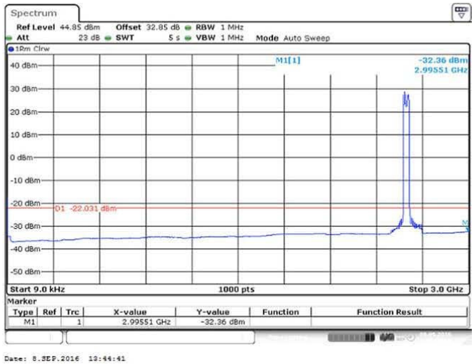
Figure 117 Spurious Emissions (9kHz – 3GHz) – 16QAM (2583.0/2603.0 MHz) (2 X 20 MHz Channel BW)
