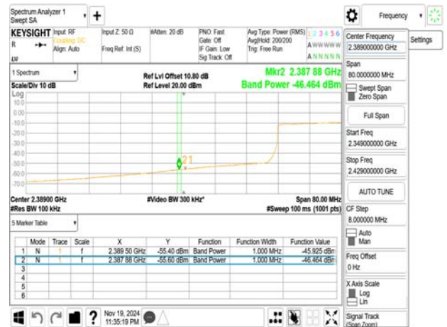
802.11ax_40MHz_2432MHz_RU242_61
