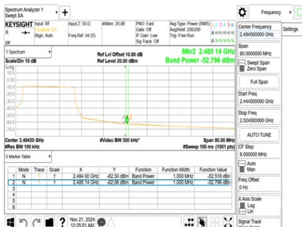
802.11ax_40MHz_2447MHz_RU484
