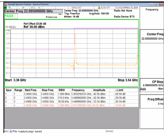
n78(3450-3550MHz) 90M DFT-s-OFDM 16QAM Edge_1RB_Left Low
