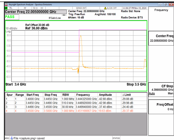
n78(3450-3550MHz) 50M DFT-s-OFDM 16QAM Edge_1RB_Left Low
