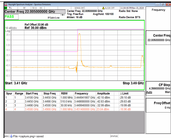
n78(3450-3550MHz) 40M DFT-s-OFDM 16QAM Edge_1RB_Left Low
