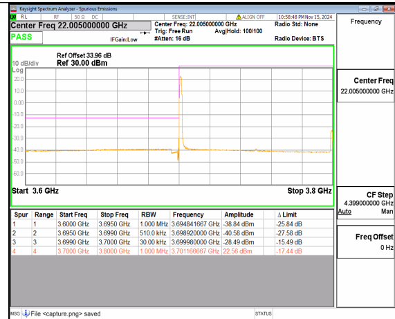
n77(3700-3980MHz) 100M DFT-s-OFDM 16QAM Edge_1RB_Left Low
