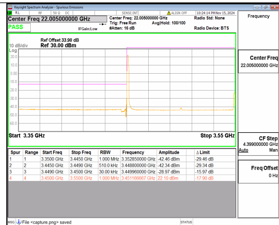
n77(3450-3550MHz) 100M DFT-s-OFDM 16QAM Edge_1RB_Left Low
