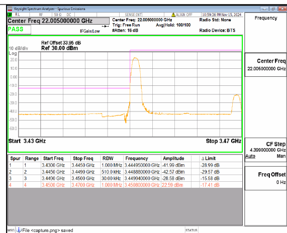
n78(3450-3550MHz) 20M DFT-s-OFDM BPSK Edge_1RB_Left Low
