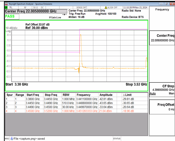
n78(3450-3550MHz) 70M DFT-s-OFDM 16QAM Edge_1RB_Left Low
