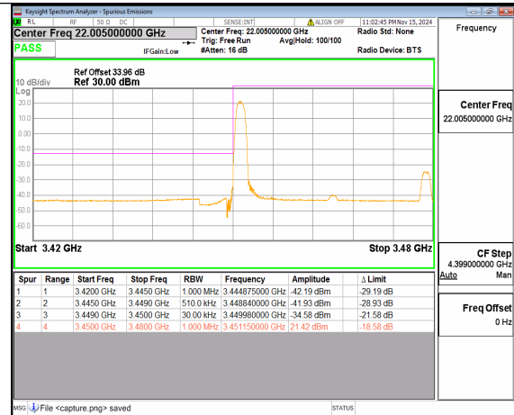
n78(3450-3550MHz) 30M DFT-s-OFDM 16QAM Edge_1RB_Left Low
