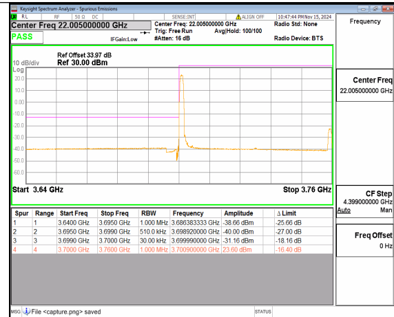
n77(3700-3980MHz) 60M DFT-s-OFDM 16QAM Edge_1RB_Left Low
