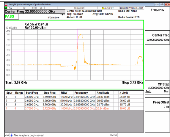
n77(3700-3980MHz) 20M DFT-s-OFDM 16QAM Edge_1RB_Left Low
