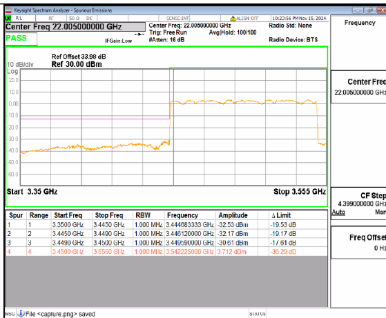
n77(3450-3550MHz) 100M DFT-s-OFDM 16QAM Outer_Full Low
