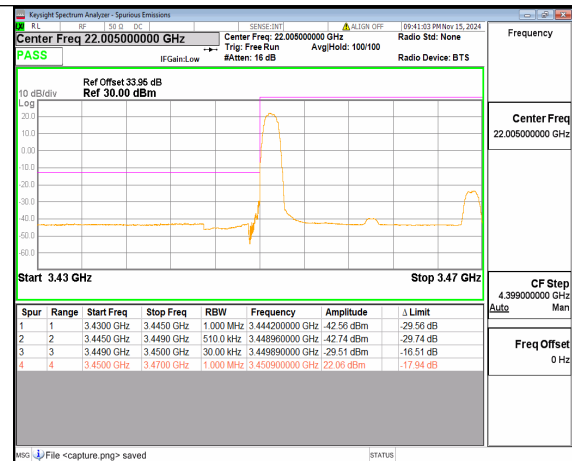
n77(3450-3550MHz) 20M DFT-s-OFDM 16QAM Edge_1RB_Left Low
