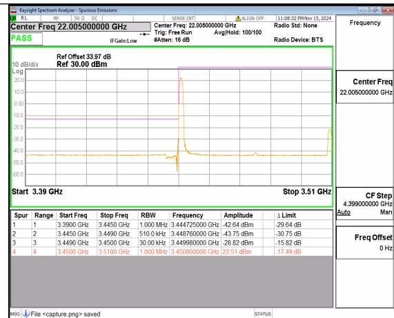
n78(3450-3550MHz) 60M DFT-s-OFDM 16QAM Edge_1RB_Left Low
