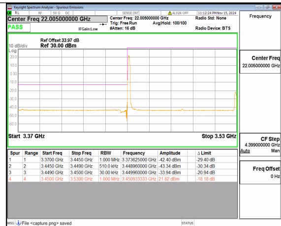
n78(3450-3550MHz) 80M DFT-s-OFDM 16QAM Edge_1RB_Left Low
