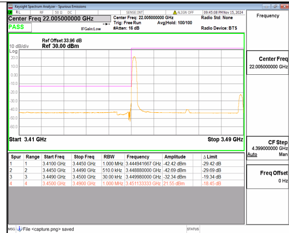
n77(3450-3550MHz) 40M DFT-s-OFDM 16QAM Edge_1RB_Left Low
