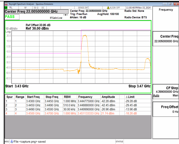
n78(3450-3550MHz) 20M DFT-s-OFDM 16QAM Edge_1RB_Left Low
