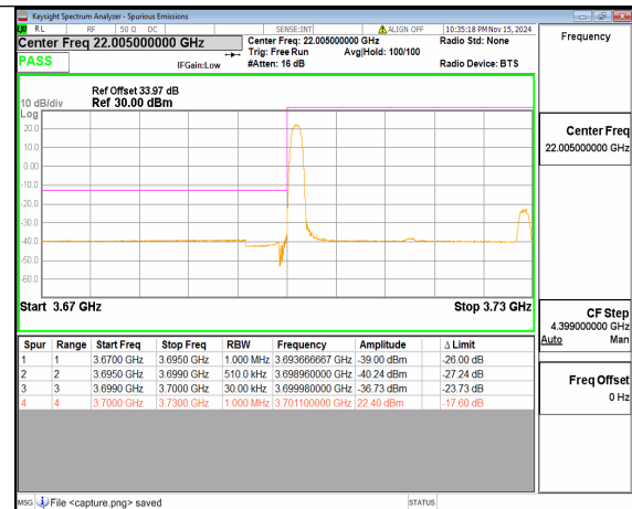
n77(3700-3980MHz) 30M DFT-s-OFDM 16QAM Edge_1RB_Left Low
