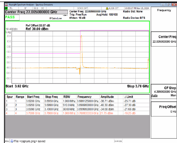
n77(3700-3980MHz) 80M DFT-s-OFDM 16QAM Edge 1RB Left Low
