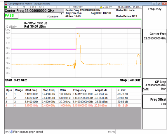
n77(3450-3550MHz) 30M DFT-s-OFDM 16QAM Edge_1RB_Left Low
