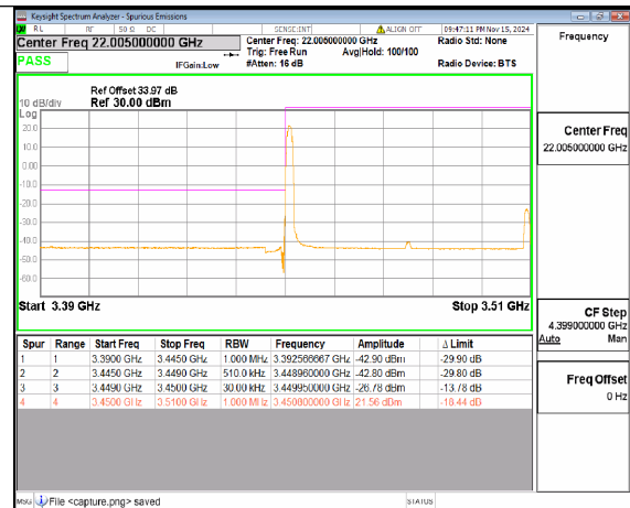
n77(3450-3550MHz) 60M DFT-s-OFDM 16QAM Edge_1RB_Left Low
