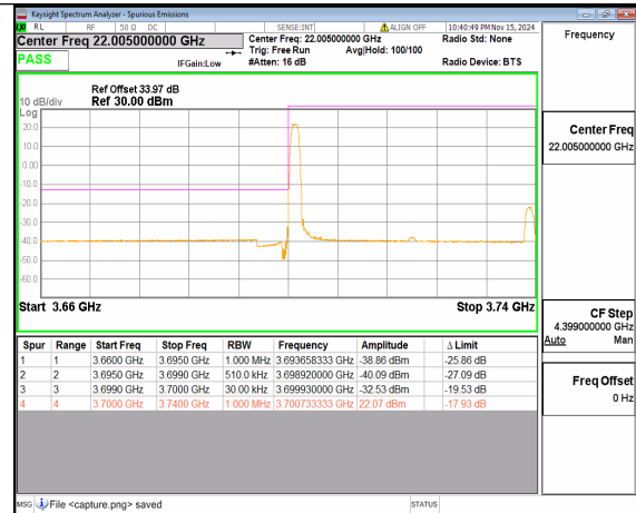
n77(3700-3980MHz) 40M DFT-s-OFDM 16QAM Edge_1RB_Left Low
