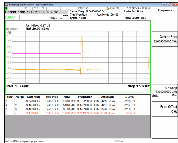
n77(3450-3550MHz) 80M DFT-s-OFDM 16QAM Edge_1RB_Left Low
