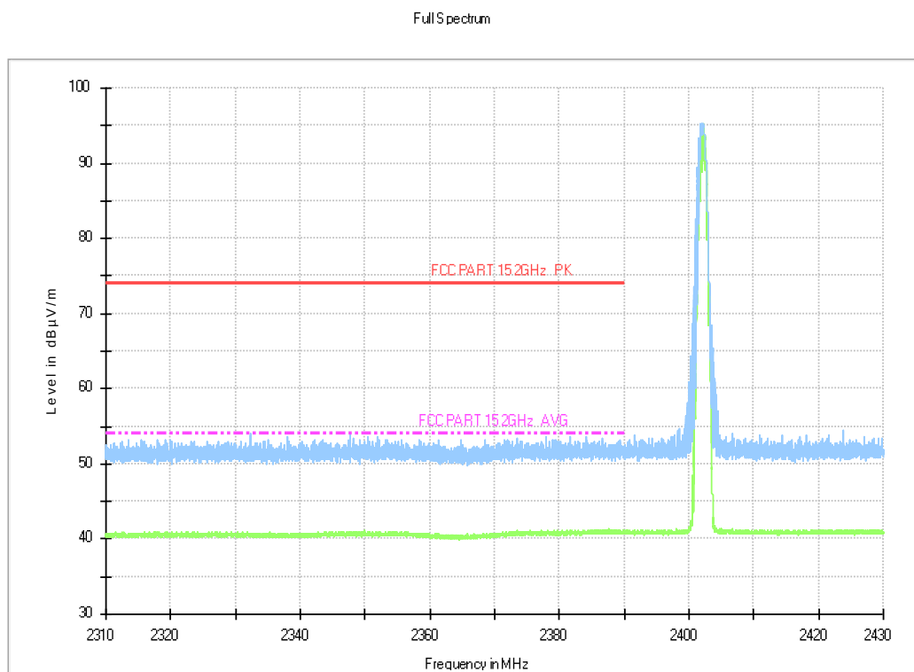
Fig.13. Frequency Band Edges: GFSK, Channel 0, 2.31 GHz – 2.43GHz
