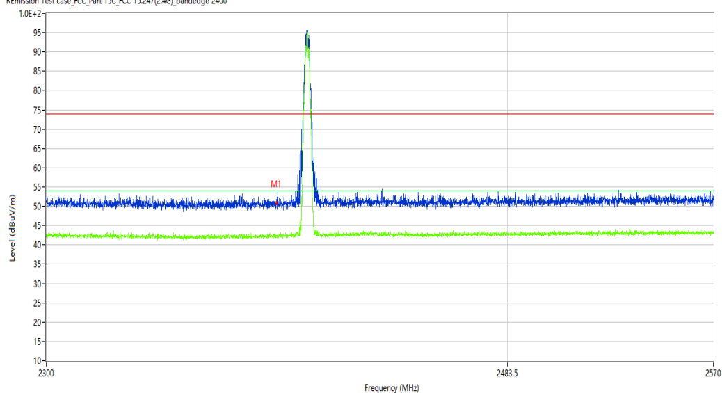
R Emission Test case_FCC_Part 15C_FCC 15.247(Z.4G)_bandedge 2400
