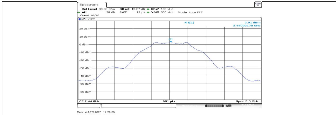
BLE_1M_Ant1_2440_0~Reference
