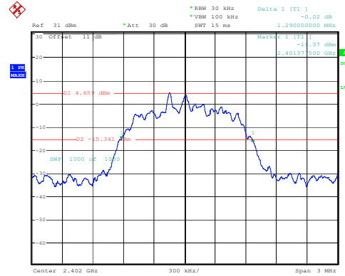
2DH1_Low 1.290MHz
