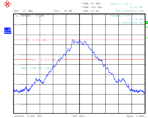
DH1_Middle 0.889MHz
