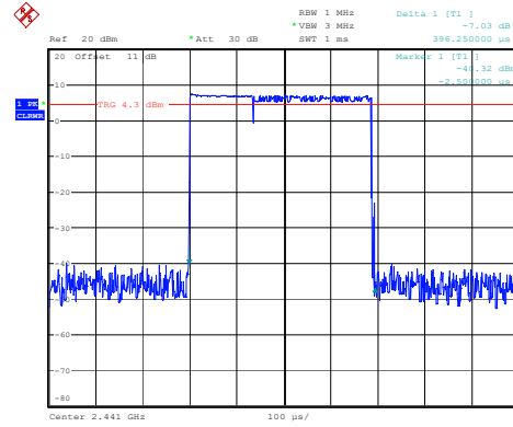
2DH1_Hopping 0.396ms
