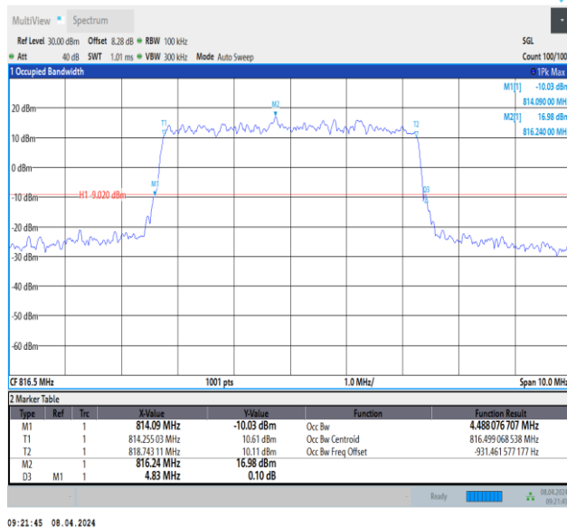
26(814-824)-5MHz-64QAM-26715-25RB#0-PASS
