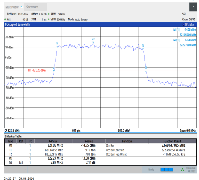
26(814-824)-3MHz-64QAM-26775-15RB#0-PASS
