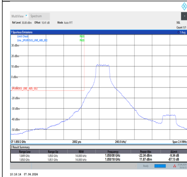
Band2_1.4MHz_16QAM_18607_1RB#0
