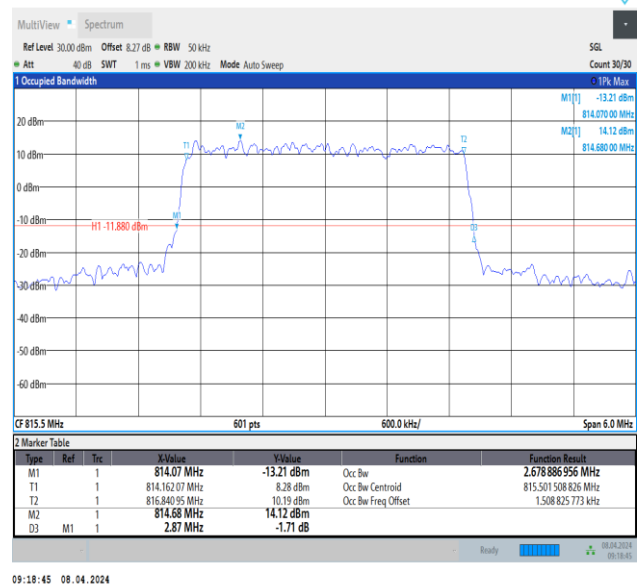
26(814-824)-3MHz-64QAM-26705-15RB#0-PASS
