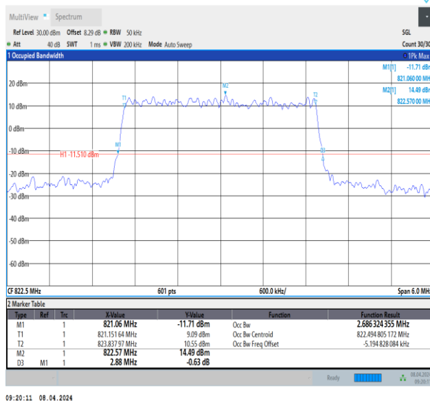
26(814-824)-3MHz-16QAM-26775-15RB#0-PASS
