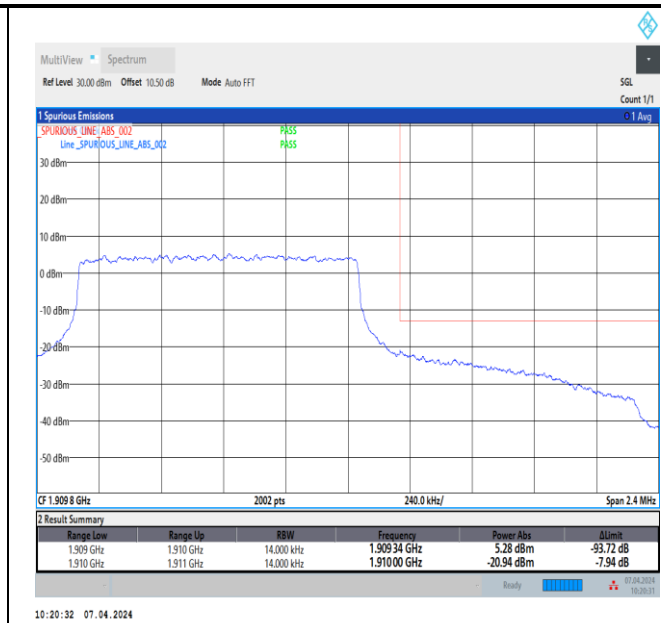
Band2_1.4MHz_QPSK_19193_6RB#0
