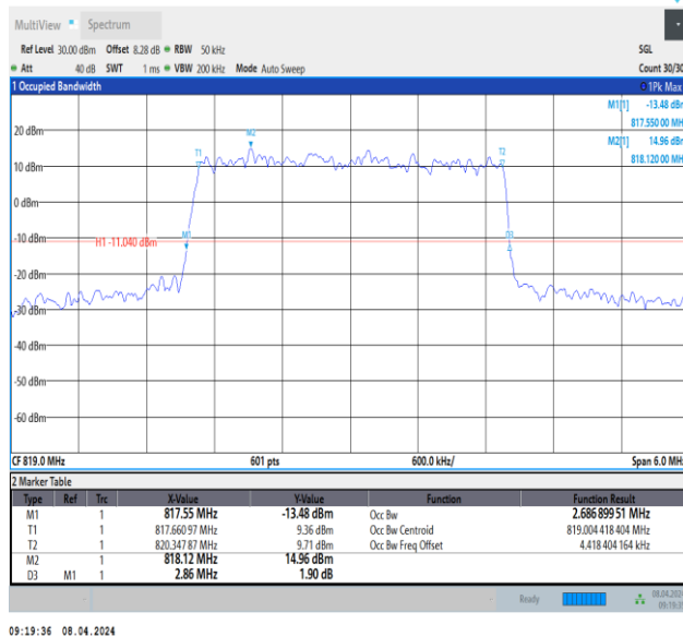
26(814-824)-3MHz-64QAM-26740-15RB#0-PASS
