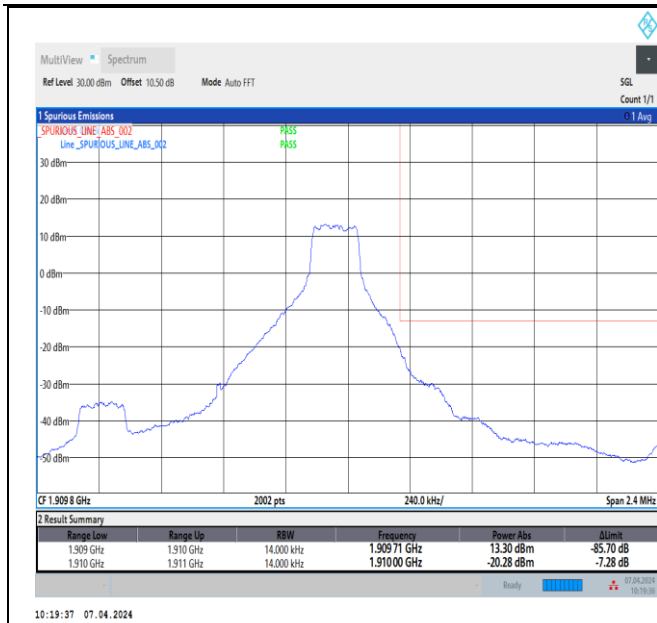
Band2_1.4MHz_QPSK_19193_1RB#5
