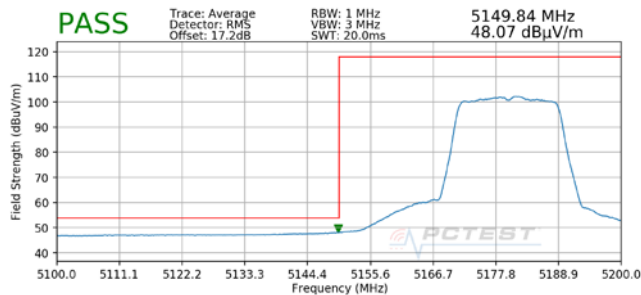
Plot 7-15. Radiated Lower Band Edge Plot MIMO (Average – UNII Band 1)
