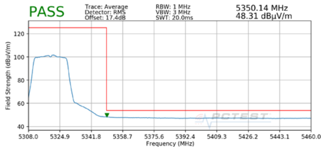
Plot 7-17. Radiated Upper Band Edge Plot MIMO (Average – UNII Band 2A)
