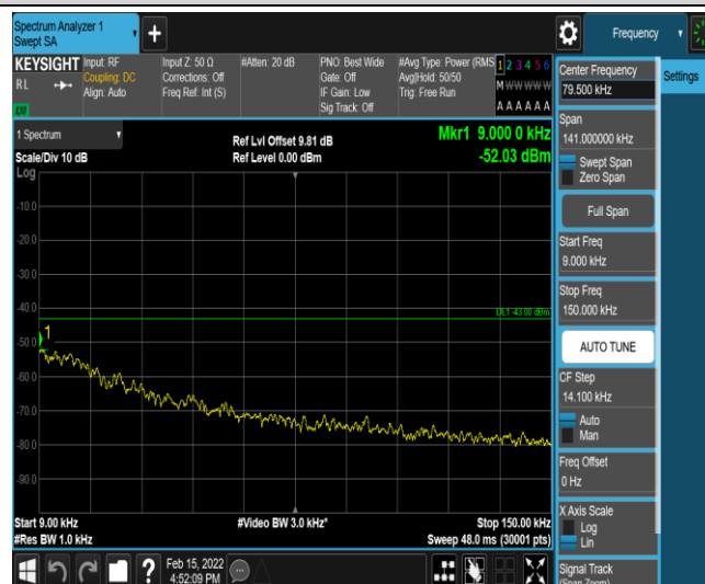
Band25-20MHz-16QAM-26140-1-0-Low-0.009-0.15--52.03-PASS
