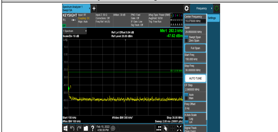
Band25-20MHz-QPSK-26590-1-0-High-0.15-30--47.62-PASS
