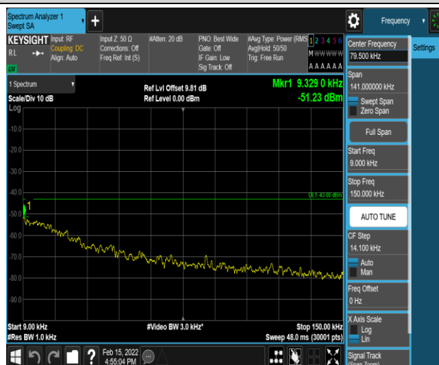
Band25-20MHz-16QAM-26365-1-0-Low-0.009-0.15--51.23-PASS
