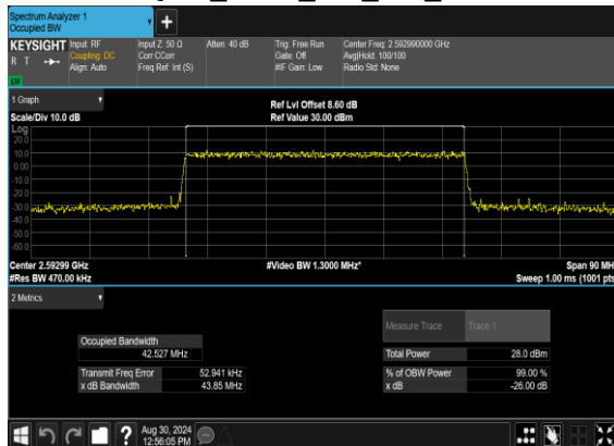
N41(45M)_CP-OFDM_64 QAM_Outer_Full_Mid_CH
