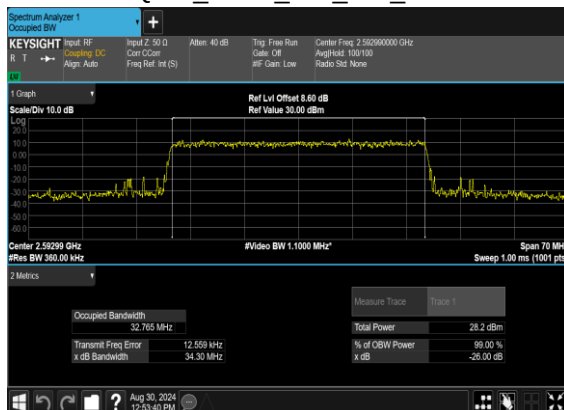
N41(35M)_CP-OFDM_64 QAM_Outer_Full_Mid_CH
