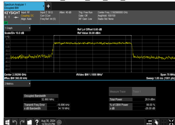
N41(35M)_CP-OFDM_16 QAM_Outer_Full_Mid_CH
