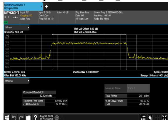
N41(35M)_CP-OFDM_256 QAM_Outer_Full_Mid_CH
