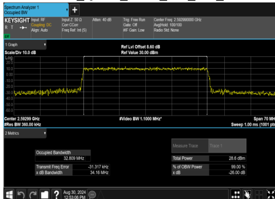
N41(35M)_CP- OFDM_QPSK_Outer_Full_Mid_CH
