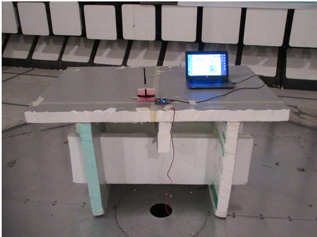
Radiated Emissions @ 3 m EUT with 2.96 Dipole Antenna, Orthogonal Position 1
