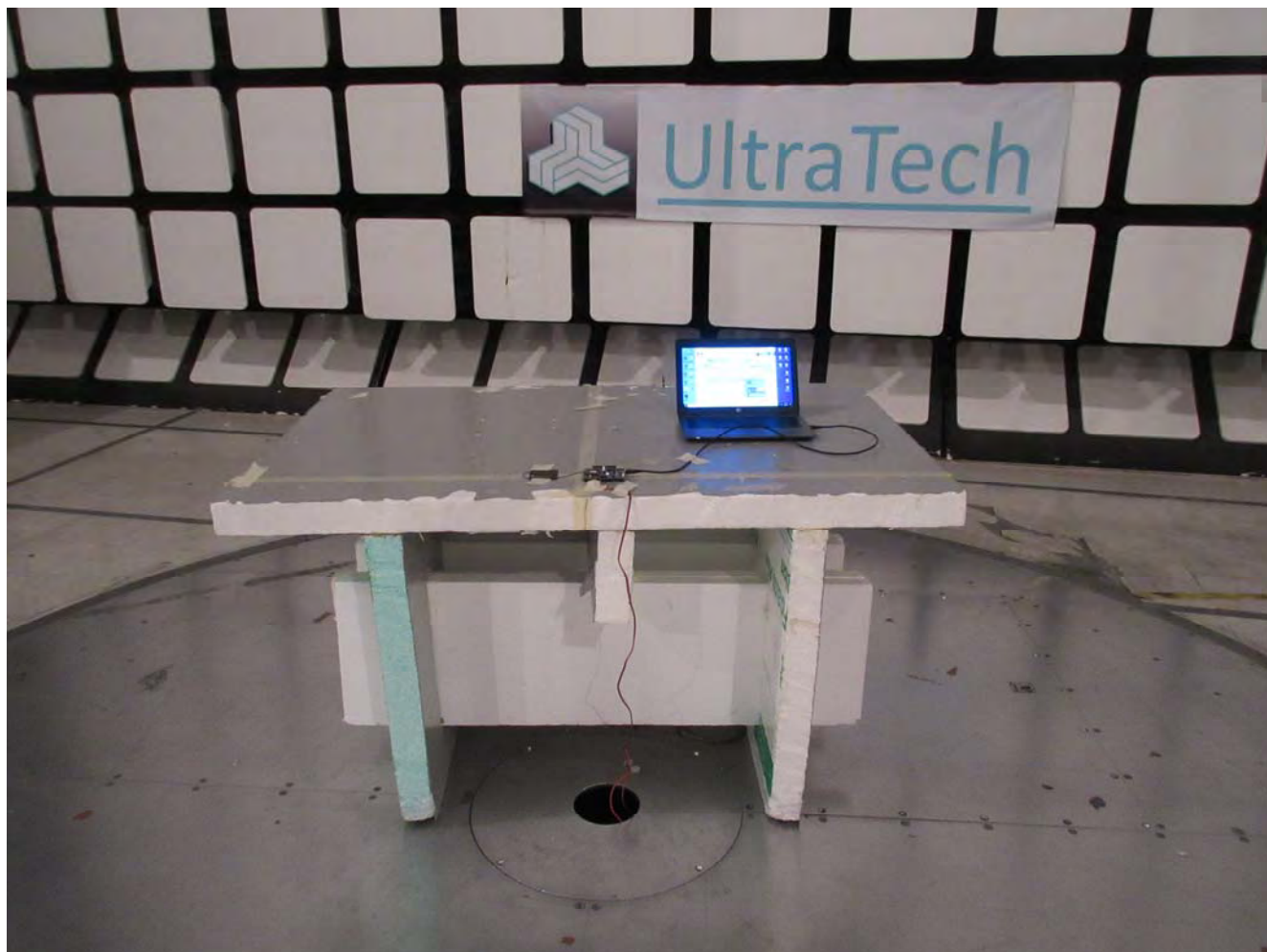
Radiated Emissions @ 3 m EUT with 2 dBi Flat Antenna, Orthogonal Position 1
