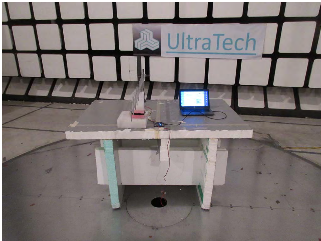
Radiated Emissions @ 3 m EUT with 15.1 dBi Yagi Antenna, Orthogonal Position 1
