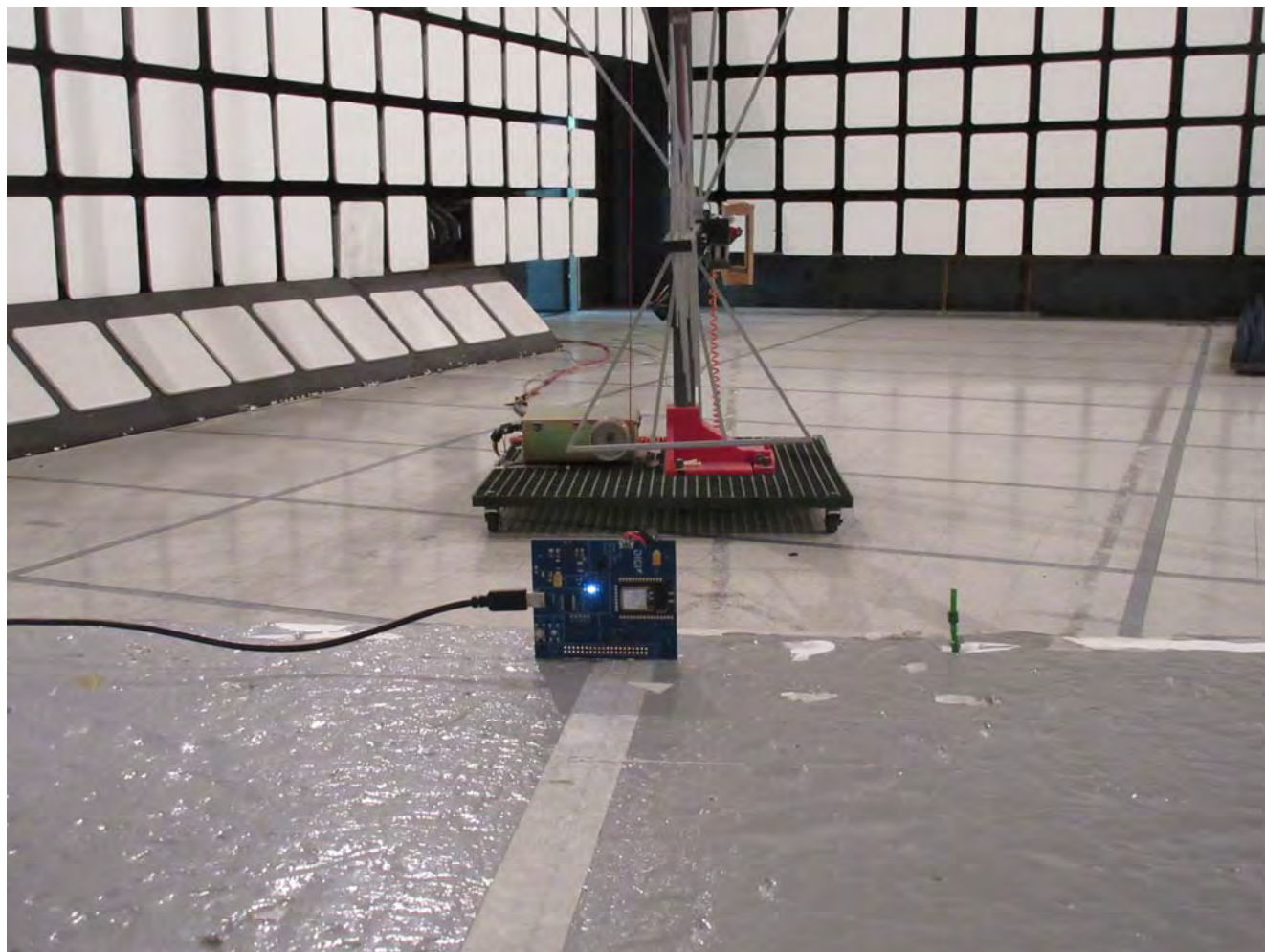
Radiated Emissions @ 3 m EUT with 0.8 dBi Ceramic Chip Antenna, Orthogonal Position 2
