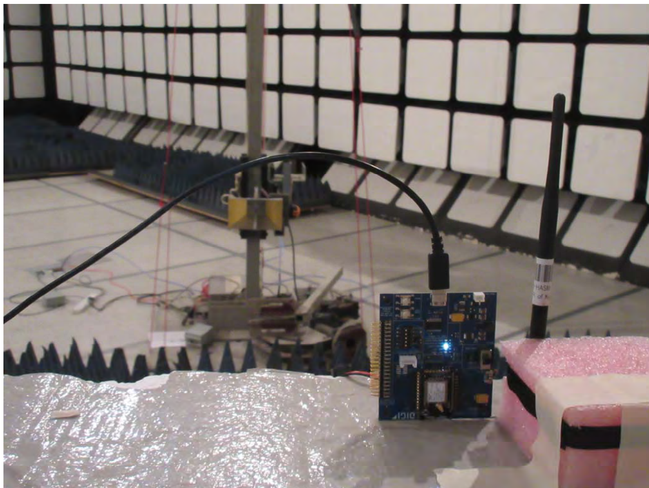
Radiated Emissions @ 3 m EUT with 2.96 Dipole Antenna, Orthogonal Position 3
