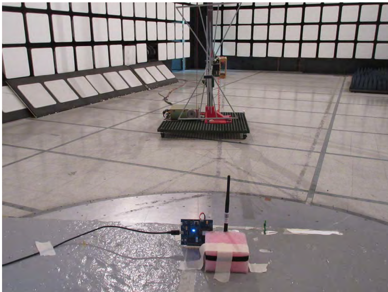
Radiated Emissions @ 3 m EUT with 2.96 Dipole Antenna, Orthogonal Position 2
