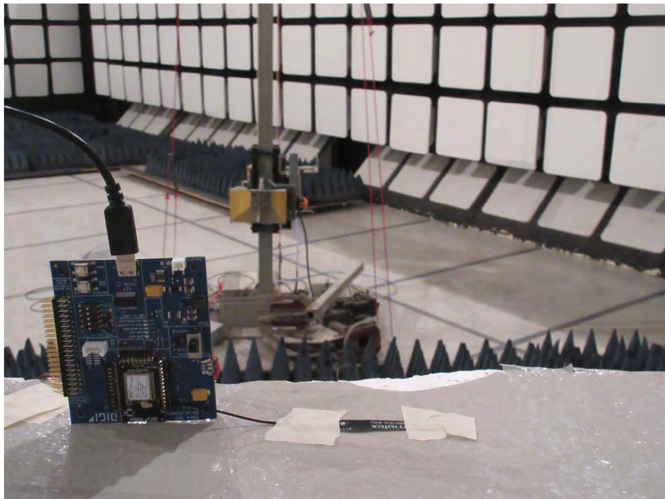
Radiated Emissions @ 3 m EUT with 1 dBi Flex Antenna, Orthogonal Position 3
