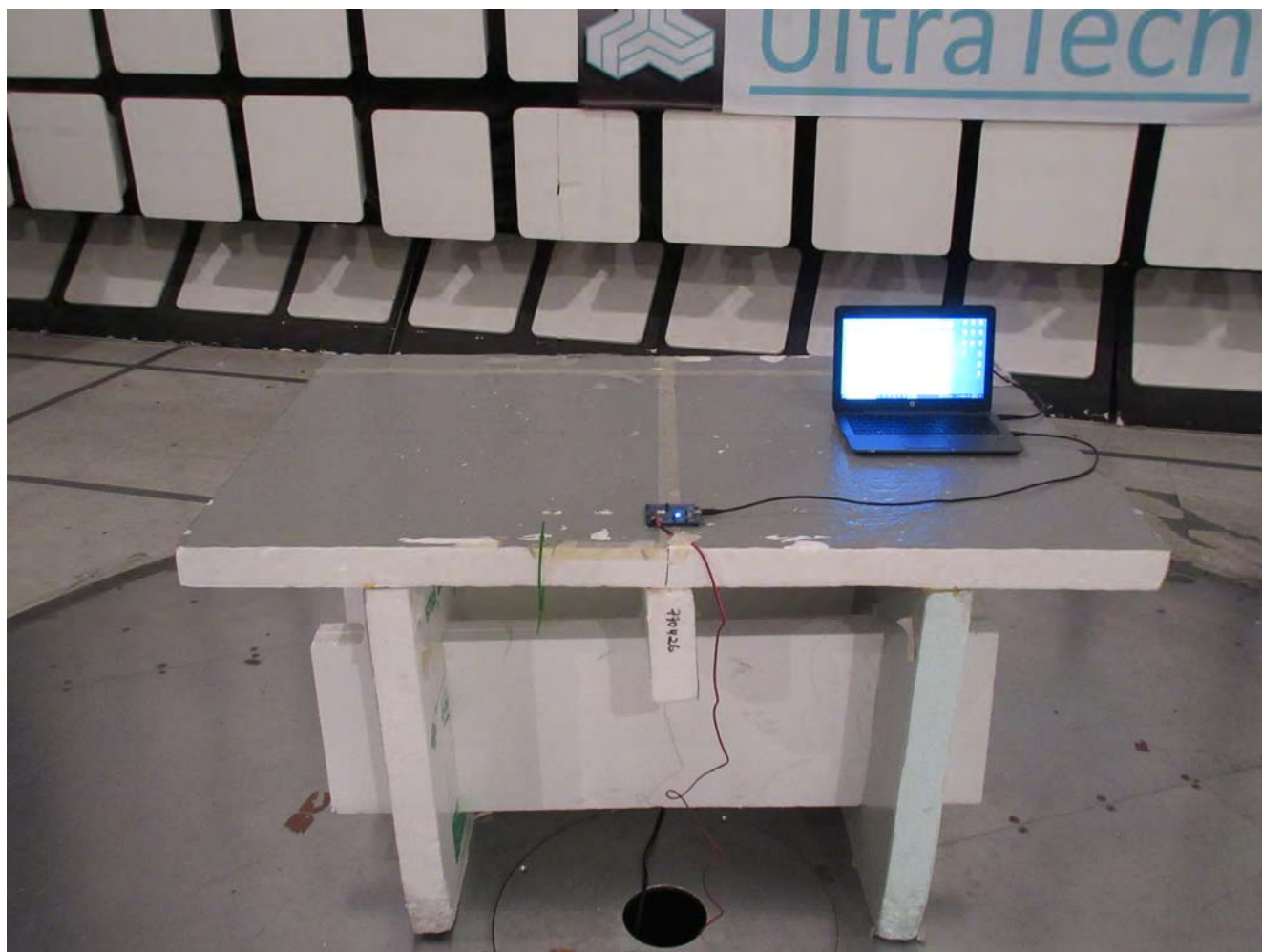
Radiated Emissions @ 3 m EUT with 0.8 dBi Ceramic Chip Antenna, Orthogonal Position 1
