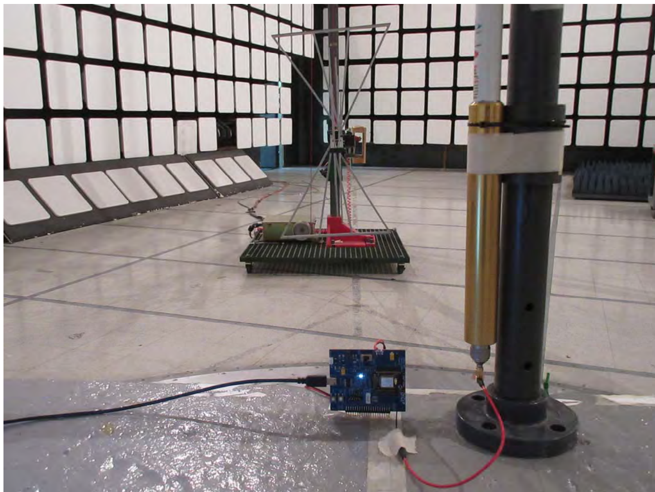
Radiated Emissions @ 3 m EUT with 8.0 dBi Omni Directional Antenna, Orthogonal Position 2
