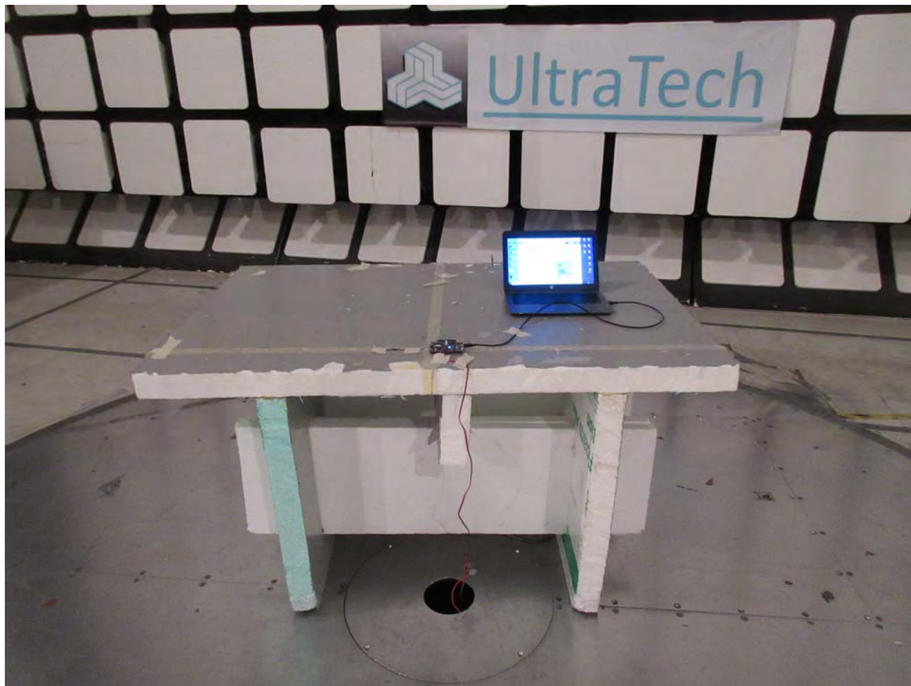
Radiated Emissions @ 3 m EUT with 1 dBi Flex Antenna, Orthogonal Position 1
