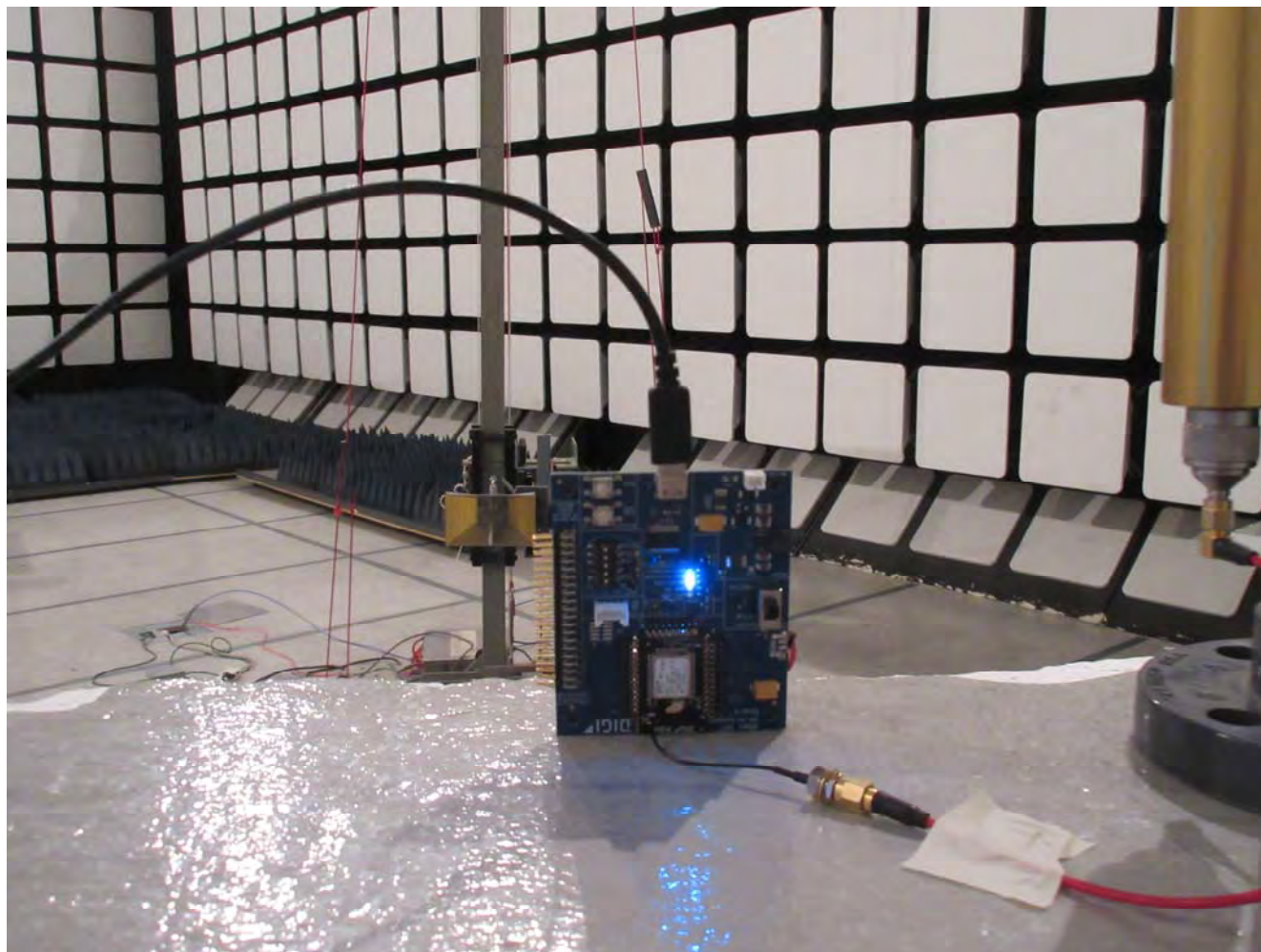
Radiated Emissions @ 3 m EUT with 8.0 dBi Omni Directional Antenna, Orthogonal Position 3
