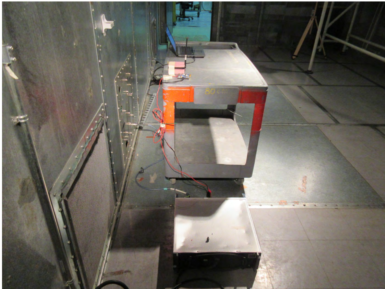
Power Line Conducted Emissions (EUT with External Antenna)
