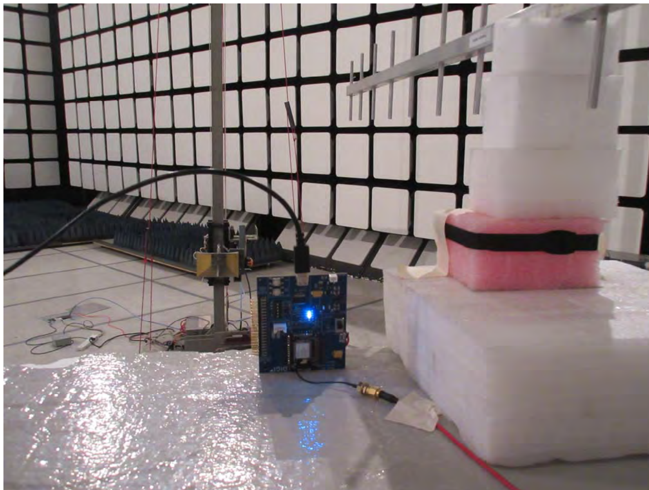
Radiated Emissions @ 3 m EUT with 15.1 dBi Yagi Antenna, Orthogonal Position 3
