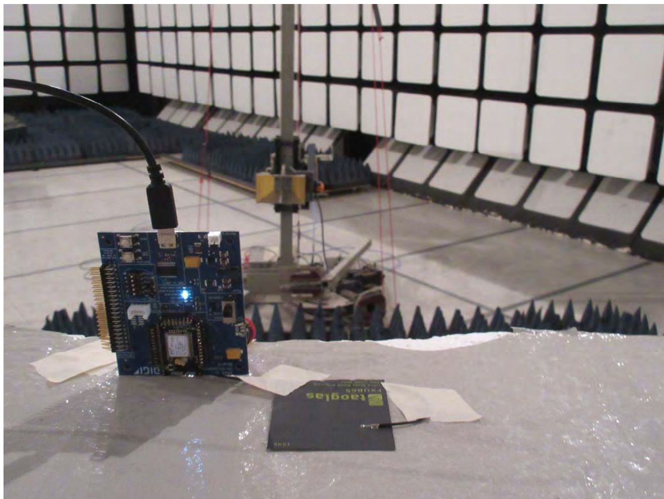
Radiated Emissions @ 3 m EUT with 2 dBi Flat Antenna, Orthogonal Position 3
