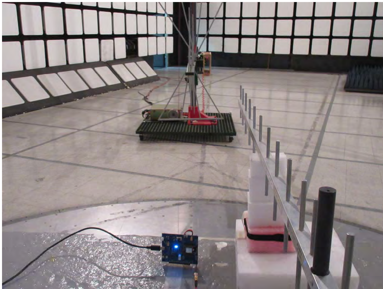
Radiated Emissions @ 3 m EUT with 15.1 dBi Yagi Antenna, Orthogonal Position 2
