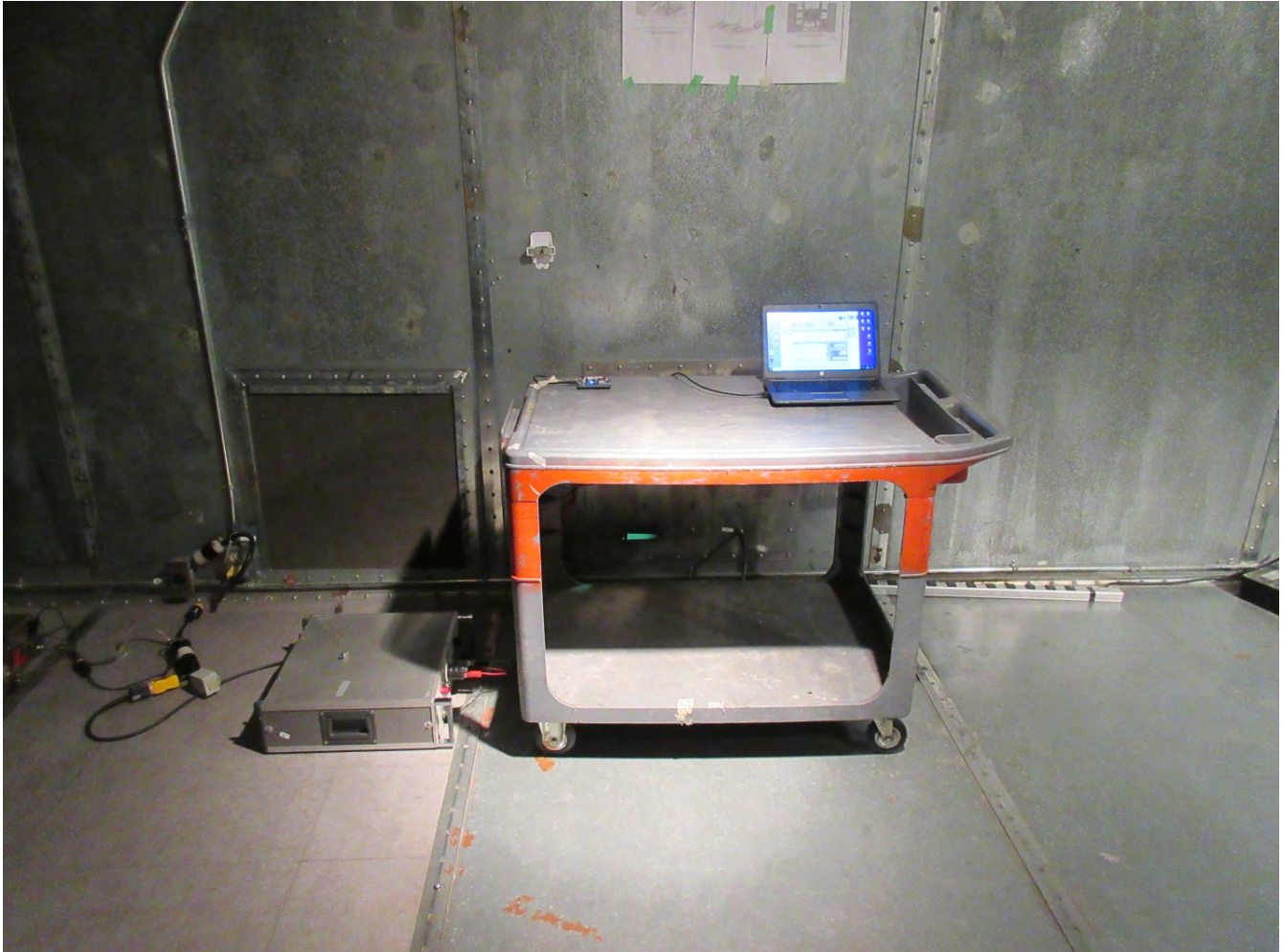
Power Line Conducted Emissions (EIT with Integral Chip Antenna)
