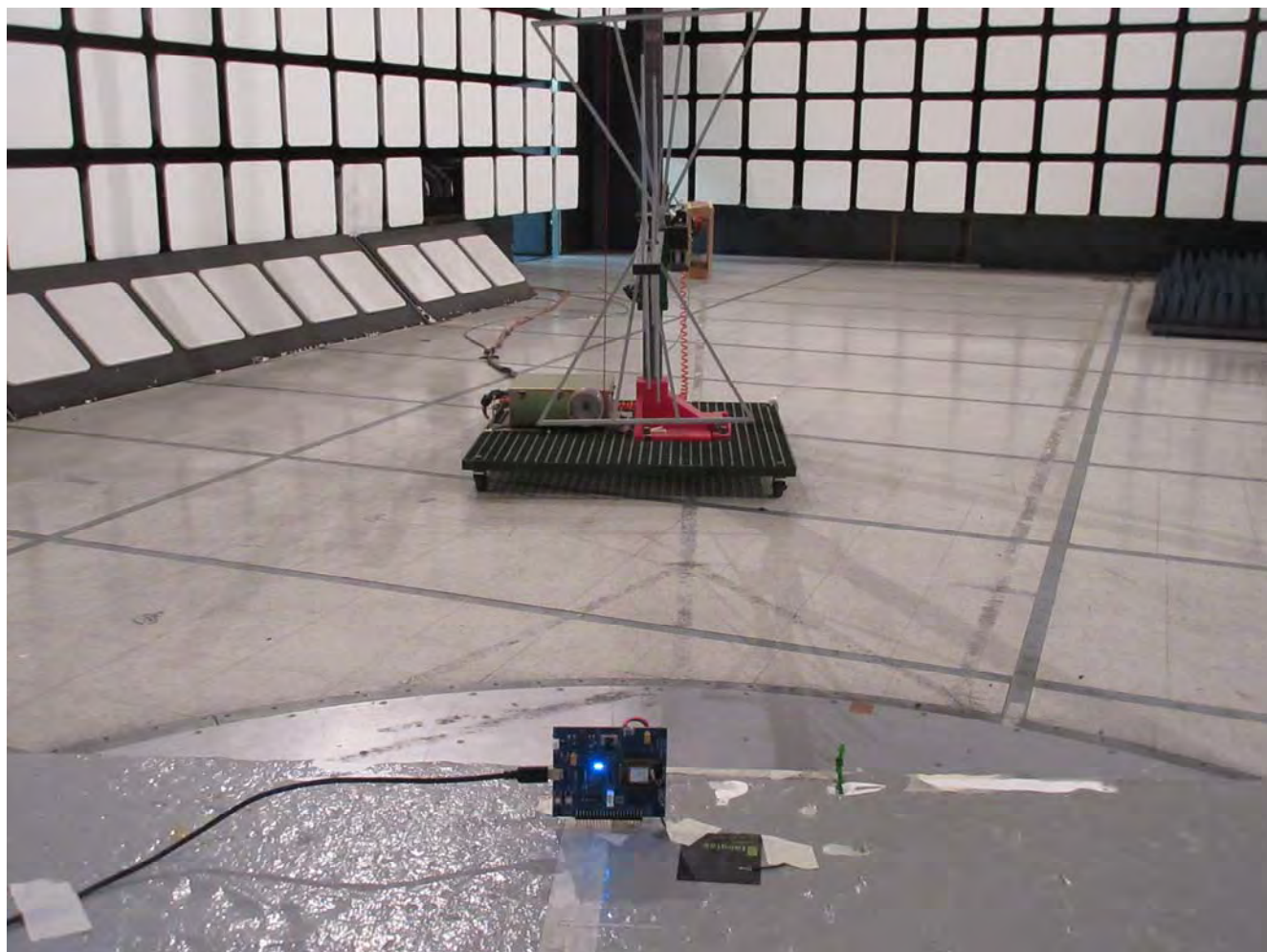
Radiated Emissions @ 3 m EUT with 2 dBi Flat Antenna, Orthogonal Position 2
