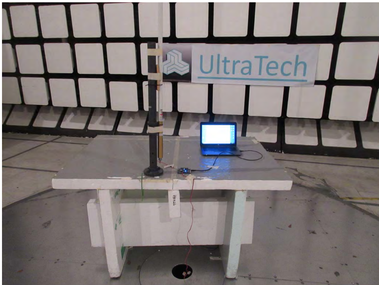
Radiated Emissions @ 3 m EUT with 8.0 dBi Omni Directional Antenna, Orthogonal Position 1
