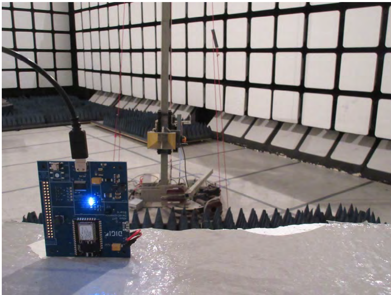
Radiated Emissions @ 3 m EUT with 0.8 dBi Ceramic Chip Antenna, Orthogonal Position 3
