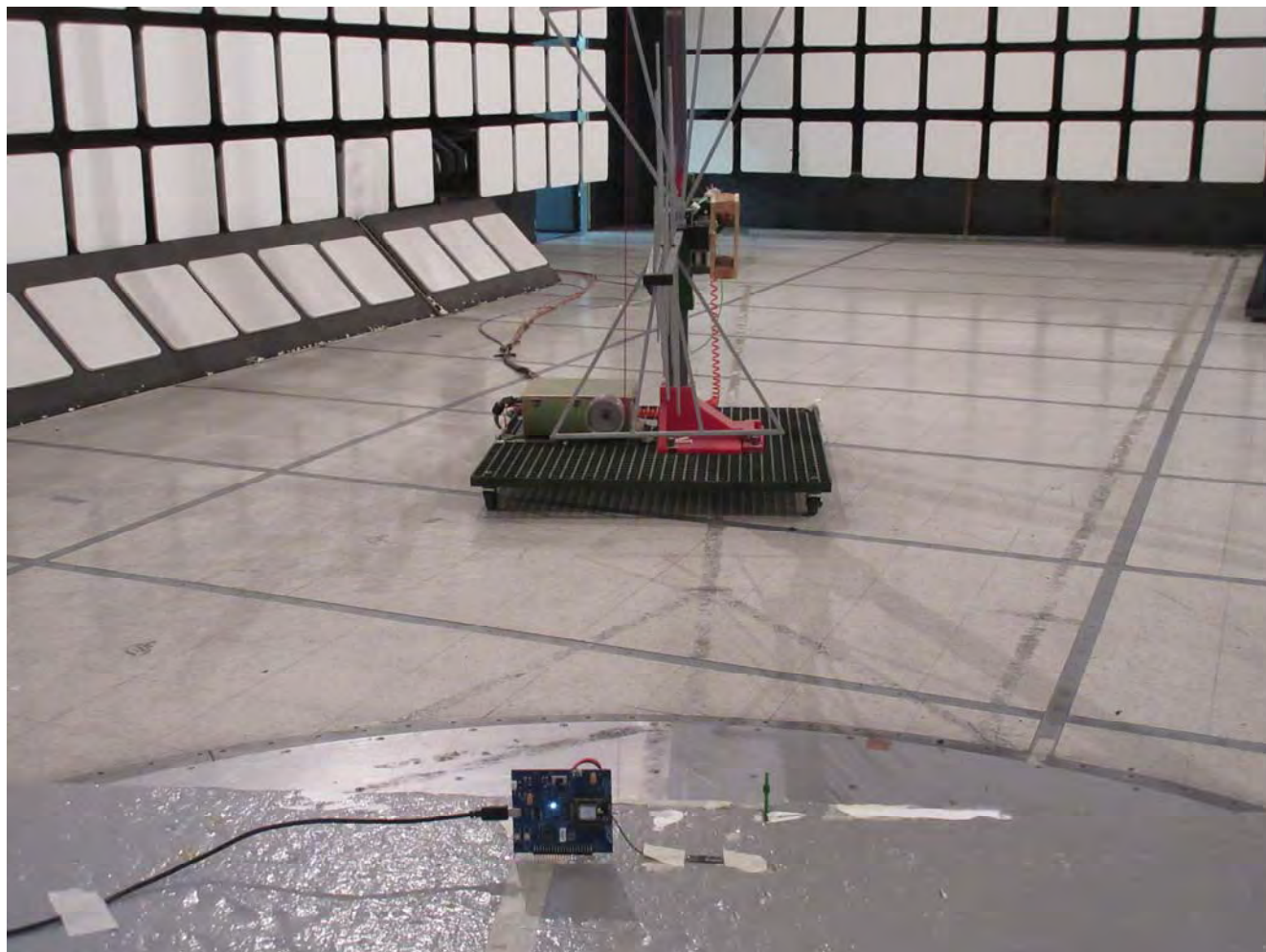
Radiated Emissions @ 3 m EUT with 1 dBi Flex Antenna, Orthogonal Position 2
