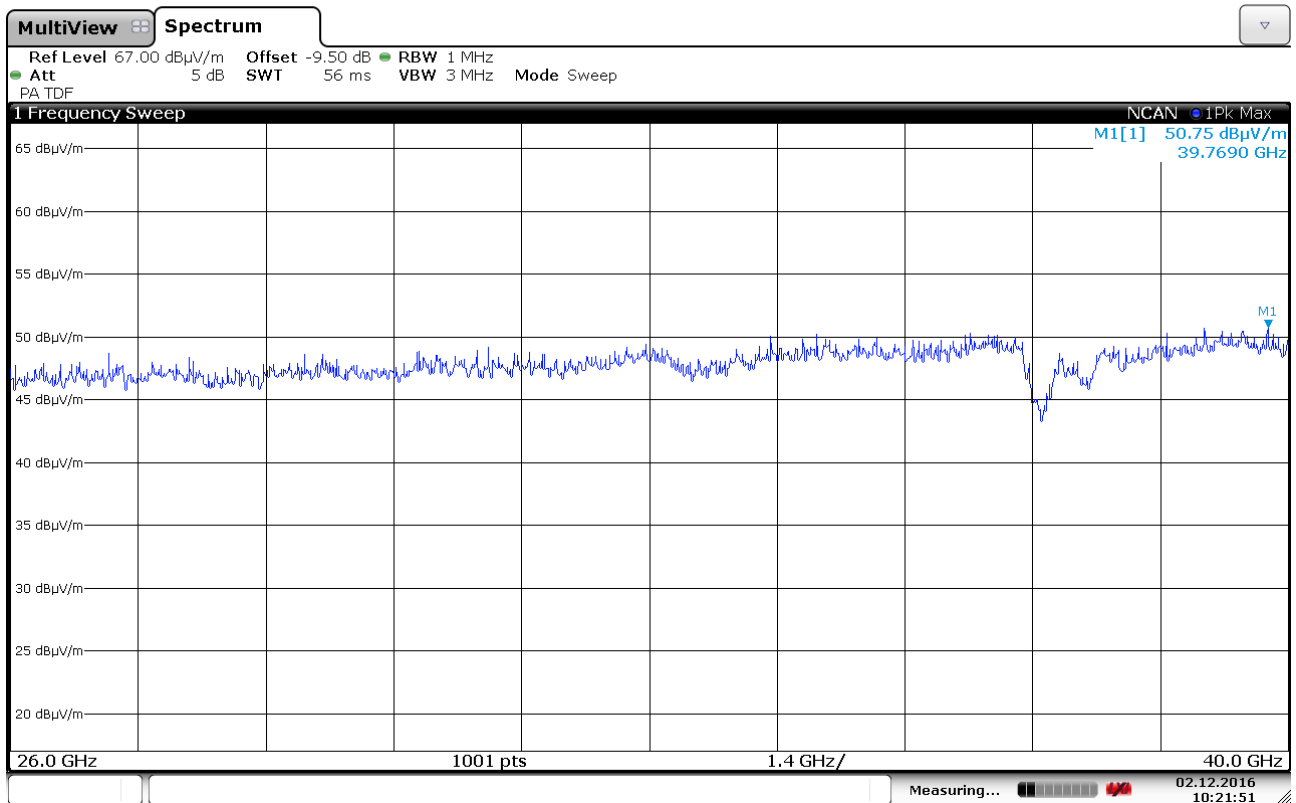
Radiated Emissions, 26.0 – 40.0 GHz, 5300 MHz, 802.11n HT20, MIMO, HP
