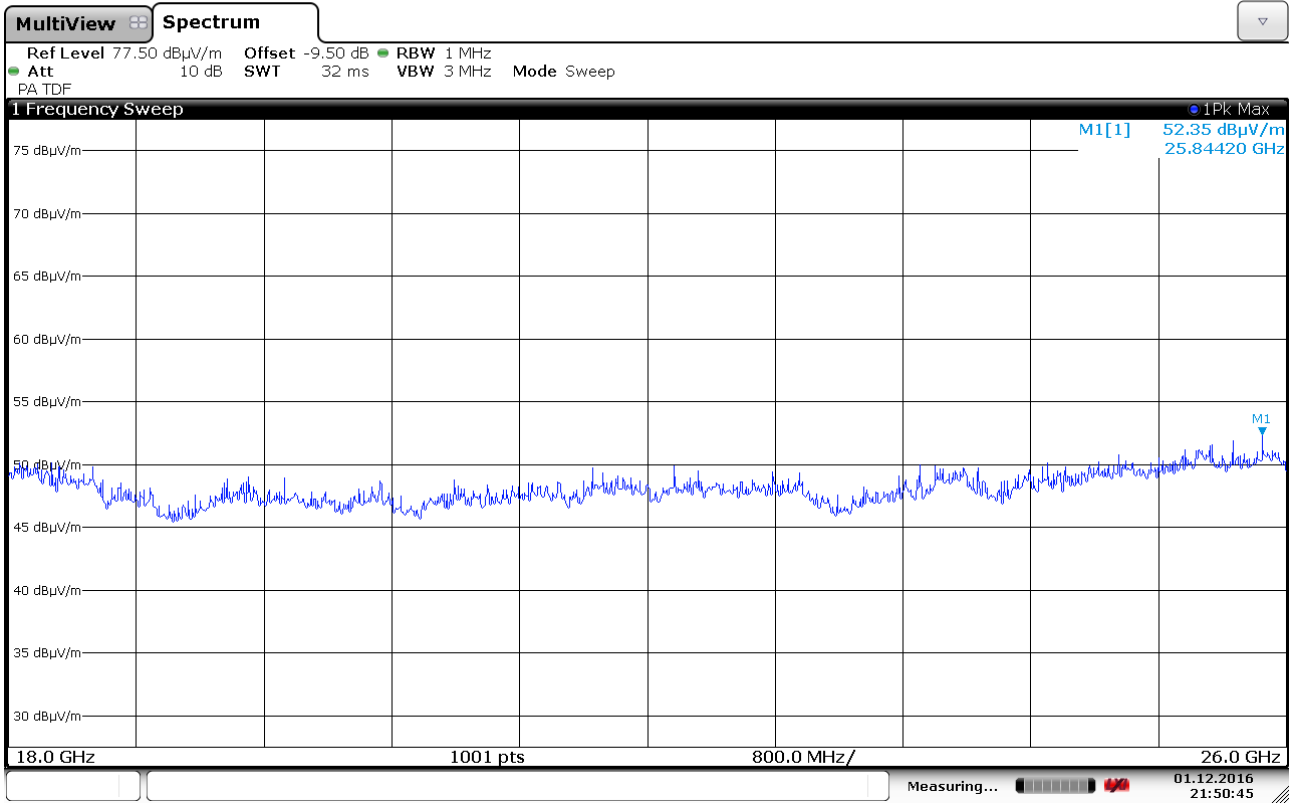
Radiated Emissions, 18.0 – 26.0 GHz, 5320 MHz, 802.11n HT20, MIMO, HP
