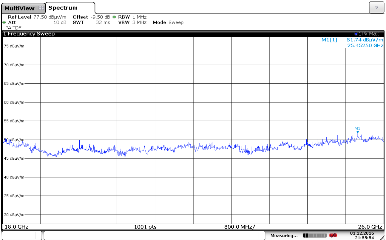
Radiated Emissions, 18.0 – 26.0 GHz, 5320 MHz, 802.11a 6M, Ant 0, VP
