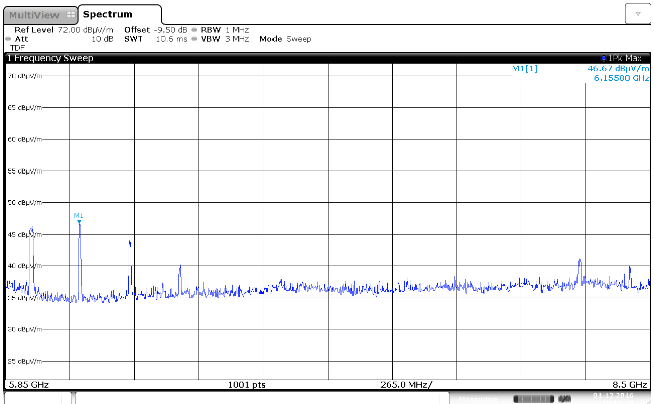
Radiated Emissions, 5.85 – 8.5 GHz, 5500 MHz, 802.11a 6M, Ant 0, VP
