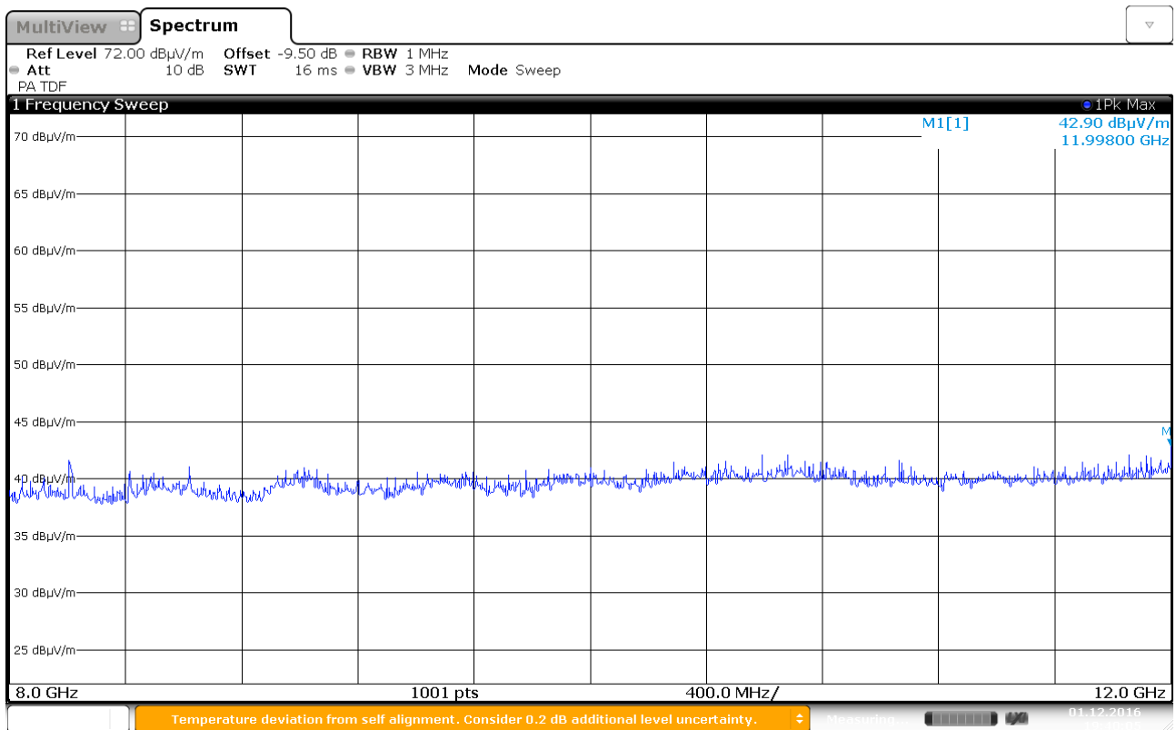
Radiated Emissions, 8.0 – 12.0 GHz, 5500 MHz, 802.11a 6M, Ant 1, VP
