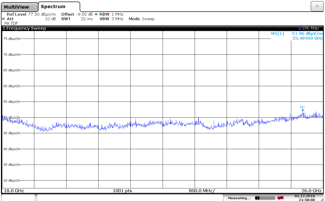
Radiated Emissions, 18.0 – 26.0 GHz, 5320 MHz, 802.11a 6M, Ant 1, VP
