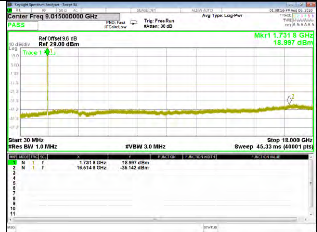
Band4_15M_QPSK_Low
