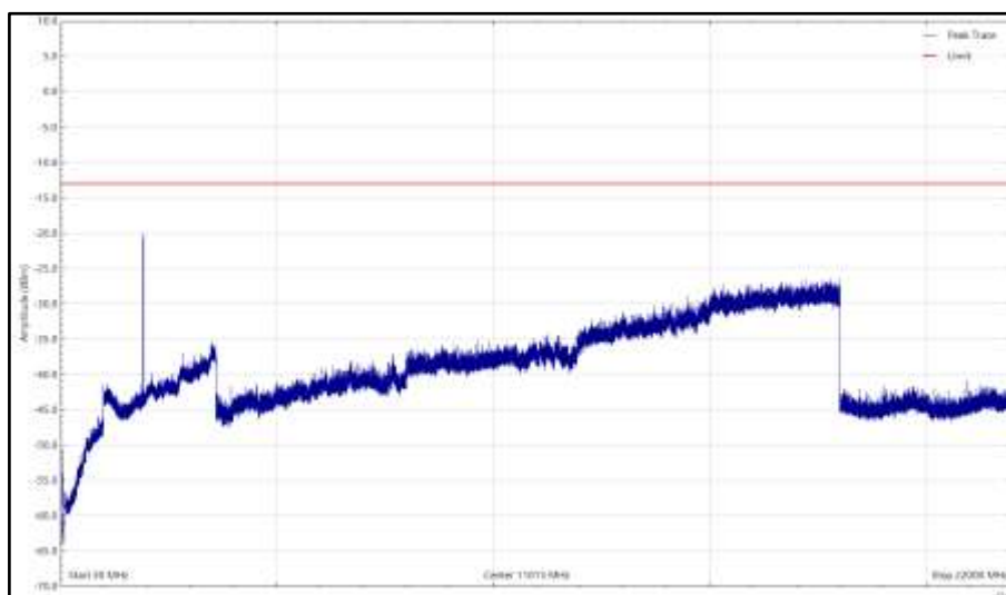
Bot - NR&NB-IoT - B2, 1935MHz, 30 MHz to 22 GHz, Vertical (Peak)
