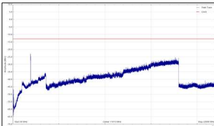
Bot - NR&NB-IoT - B25, 1940MHz, 30 MHz to 22 GHz, Vertical (Peak)
