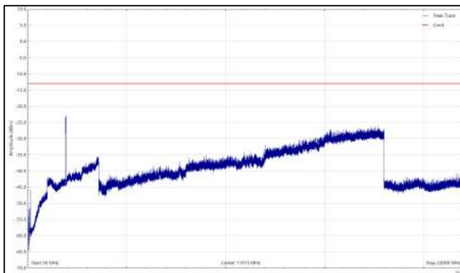
Bot - NR&NB-IoT - B25, 1940MHz, 30 MHz to 22 GHz, Horizontal (Peak)
