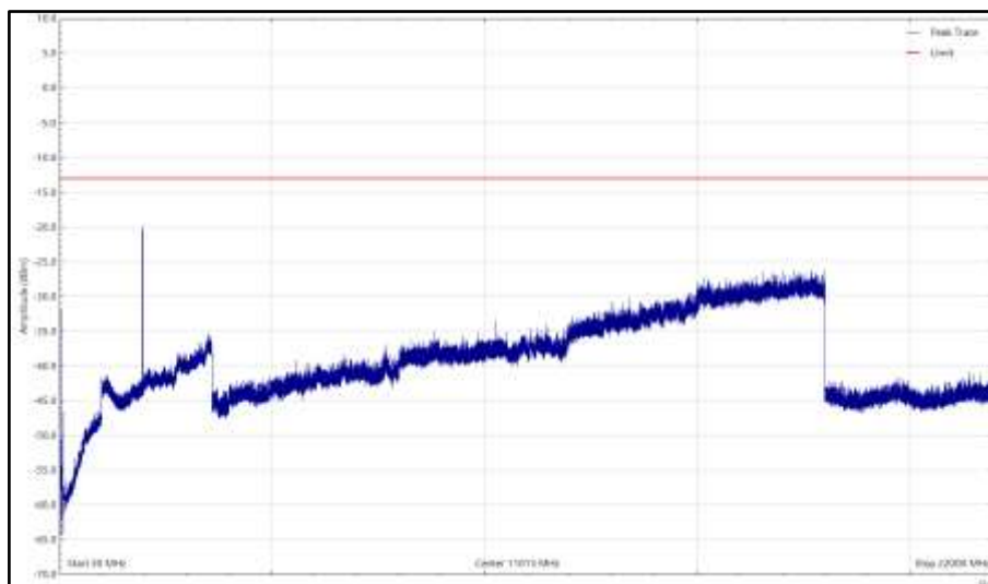
Mid - NR&NB-IoT - B25, 1962.5MHz, 30 MHz to 22 GHz, Vertical (Peak)
