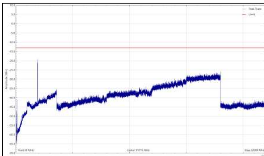
Bot - NR&NB-IoT - B2, 1935MHz, 30 MHz to 22 GHz, Horizontal (Peak)
