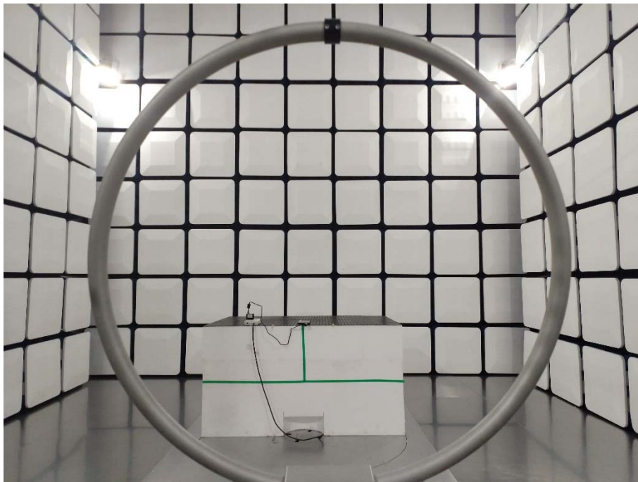
Below 30MHz-WIFI
